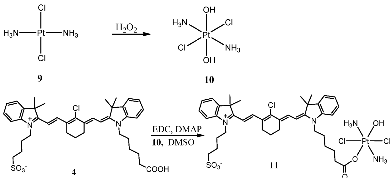
Scheme 4 - Illustrative reaction scheme for the synthesis of DZ-CIS ester.
