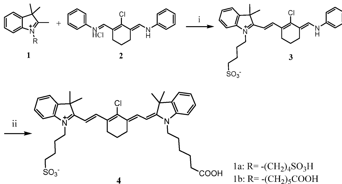
Scheme 1. Reagents and conditions: (i) 1a , NaOAc, EtOH, reflux, 3h; (ii) 1b , NaOAc, EtOH, reflux, 3h
