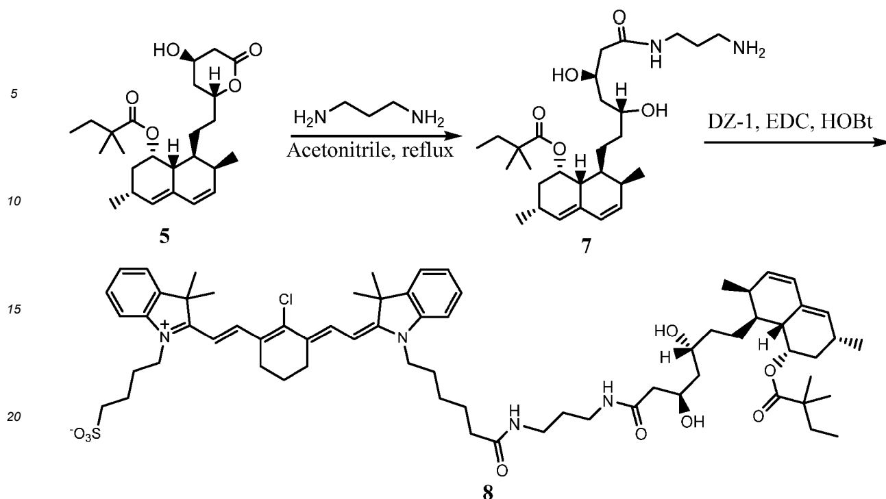
Scheme 3 - Illustrative reaction scheme for the synthesis of DZ-SIM amide.
