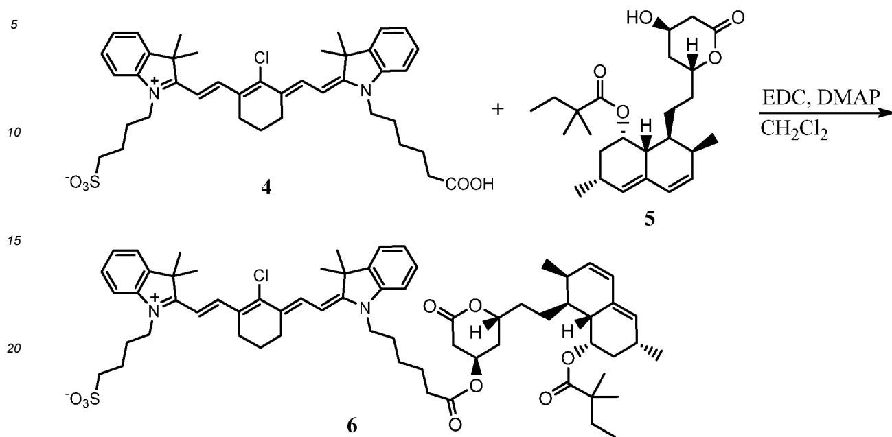
Scheme 2. - Illustrative reaction scheme for the synthesis of DZ-SIM ester
