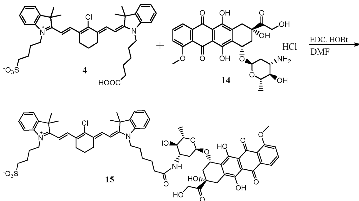
Scheme 6. Synthesis of DZ-1-Dox amide conjugate
