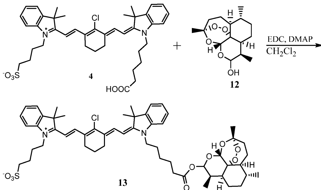
Scheme 5. Synthesis of DZ-ART ester conjugate
