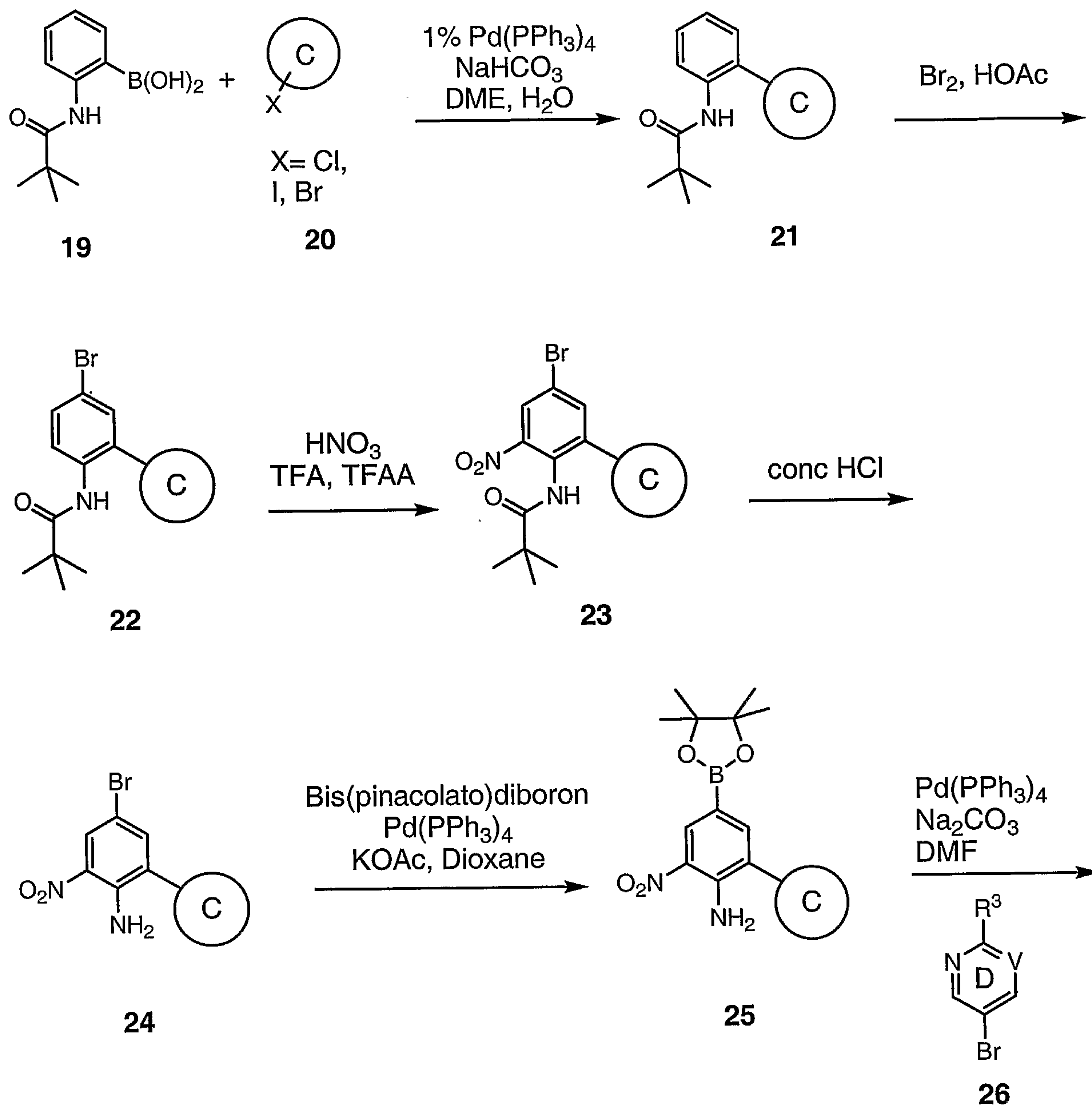
Scheme V
