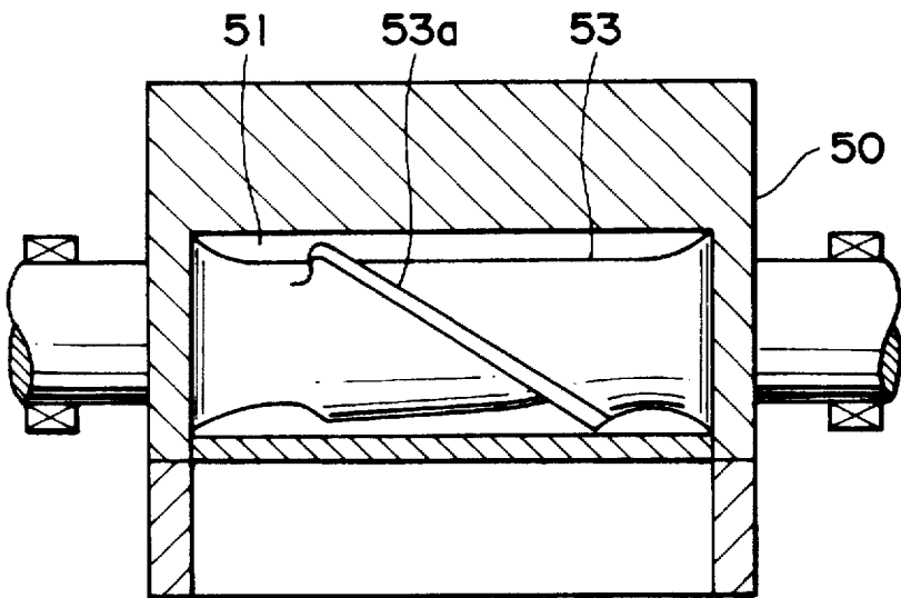
CROSS SECTIONAL VIEW TAKEN ALONG LINE A-A OF FIG.6
