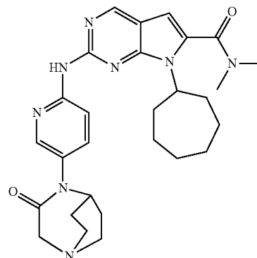
7-cyclopentyl-N,N-dimethyl-2-(5-(3-oxo-1,4-diazabicyclo[3.2.2]nonan-4-yl)pyridin-2-ylamino)-7H-pyrrolo[2,3-d]pyrimidine-6-carboxamide
