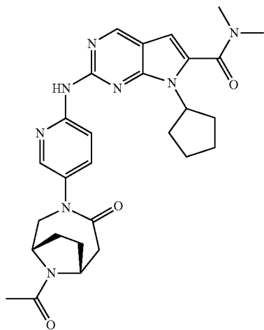
2-(5-((1S,6R)-9-acetyl-4-oxo-3,9-diazabicyclo[4.2.1]nonan-3-yl)pyridin-2-ylamino)-7-cyclopentyl-N,N-dimethyl-7H-pyrrolo[2,3-d]pyrimidine-6-carboxamide
