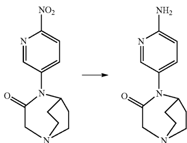
4-(6-aminopyridin-3-yl)-1,4-diazabicyclo[3.2.2]nonan-3-one
