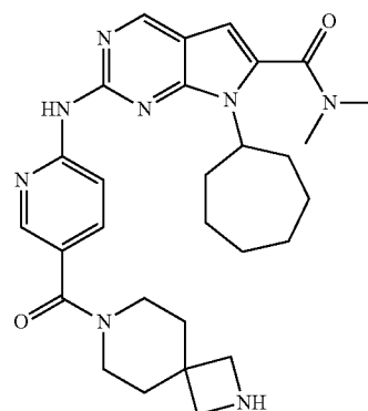
2-(5-(2,7-diazaspiro[3.5]nonane-7-carbonyl)pyridin-2-ylamino)-7-cycloheptyl-N,N-dimethyl-7H-pyrrolo[2,3-d]pyrimidine-6-carboxamide
