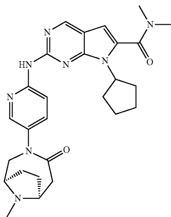
7-cyclopentyl-N,N-dimethyl-2-(5-((1R,6S)-9-methyl-4-oxo-3,9-diazabicyclo[4.2.1]nonan-3-yl)pyridin-2-ylamino)-7H-pyrrolo[2,3-d]pyrimidine-6-carboxamide
