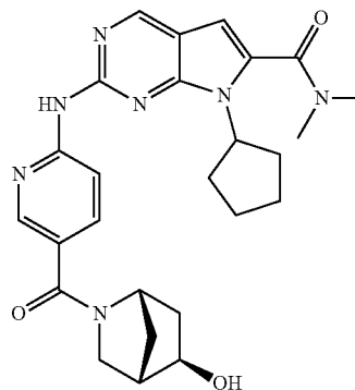
7-cyclopentyl-2-(5-((1S,4S,5R)-5-hydroxy-2-azabicyclo[2.2.1]heptan-2-carbonyl)pyridin-2-ylamino)-N,N-dimethyl-7H-pyrrolo[2,3-d]pyrimidine-6-carboxamide
