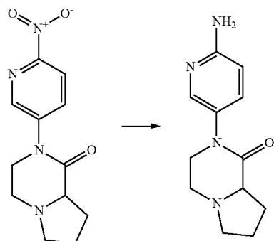
2-(6-Amino-pyridin-3-yl)-hexahydro-pyrrolo[1,2-a] pyrazin-1-one
