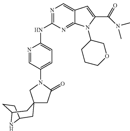
N,N-dimethyl-2-(5-(5'-oxo-8-azaspiro[bicyclo[3.2.1]octane-3,3'-pyrrolidine]-1'-yl)pyridin-2-ylamino)-7-(tetrahydro-2H-pyran-3-yl)-7H-pyrrolo[2,3-d]pyrimidine-6-carboxamide
