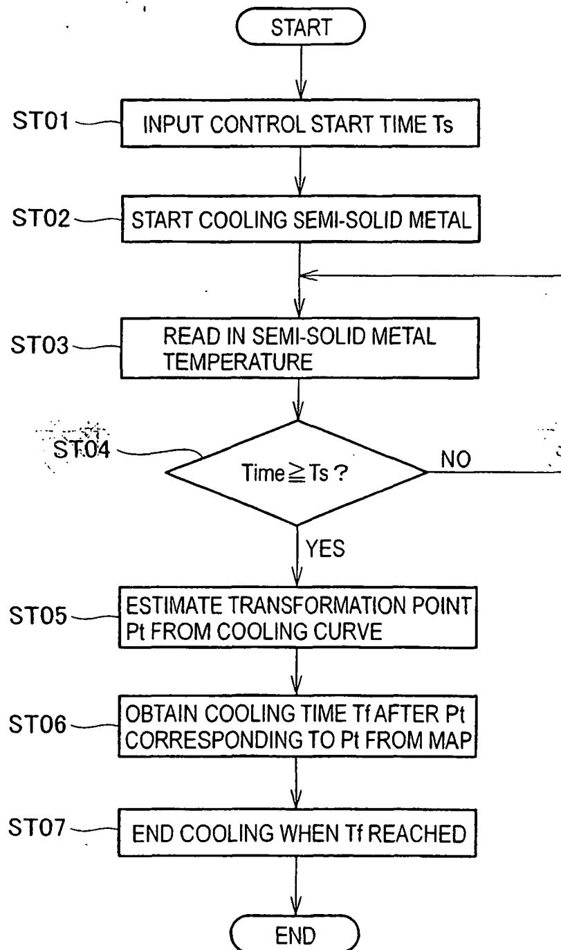
FIG. 35 (Prior Art)
