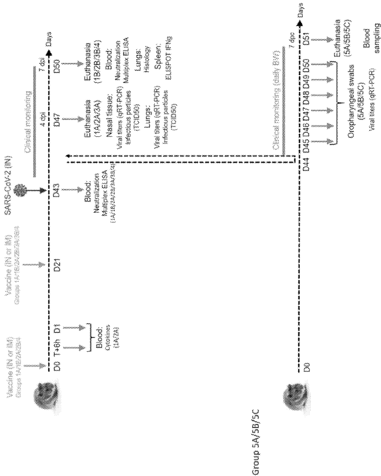
Scheme 3
