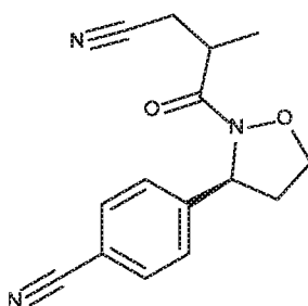
DIASTEREOMER. 2
