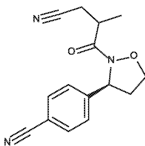
DIASTEREOISOMER 1
