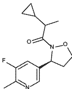
DIASTEREOISOMER 1
