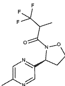
DIASTEREOISOMER 2
