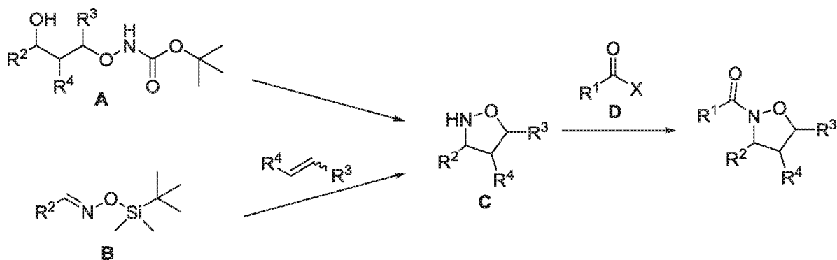
Scheme I
