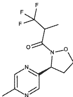
DIASTEREOISOMER 1
