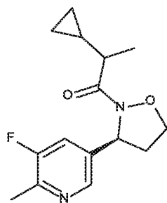
DIASTEREOISOMER 2
