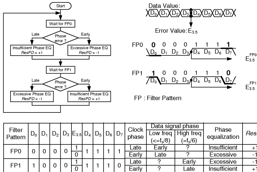
Filter Pattern Decoder for phase distortion
