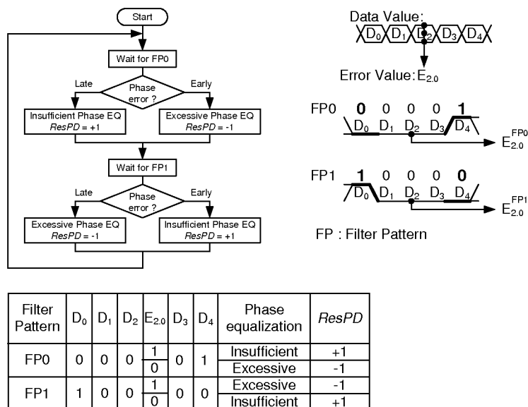
Filter Pattern Decoder for phase distortion
