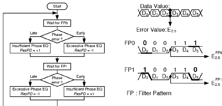
Filter Pattern Decoder for phase distortion
