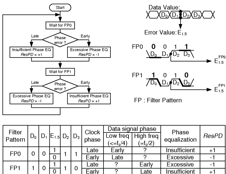
Filter Pattern Decoder for phase distortion
