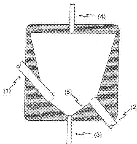
Figure 7. Reservoir design 7. Placement of (2) is arbitrary.
