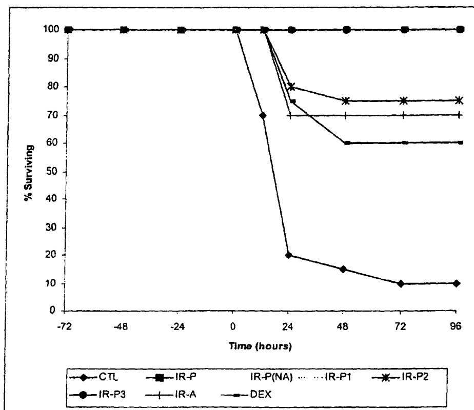
Figure 58. To determine the effect of high-dose LPS treatment in IR treated mice. Balb/c mice (n=30) were injected intraperitoneally with LPS (150 mg/kg) and survival was assessed daily 5 days. PBS-treated Balb/c mice succumbed to shock between days 1 and 2 after high-dose LPS injection, with only 10% of the animals were alive on day 5. In contrast, 100% of IR-P, or its fraction IR-P1, IR-P3 treated mice were alive on day 5 ( P < 0.001 ), while IR-P2, IR-A and Dexamethasone treated mice demonstrated around 70% of surviving.
