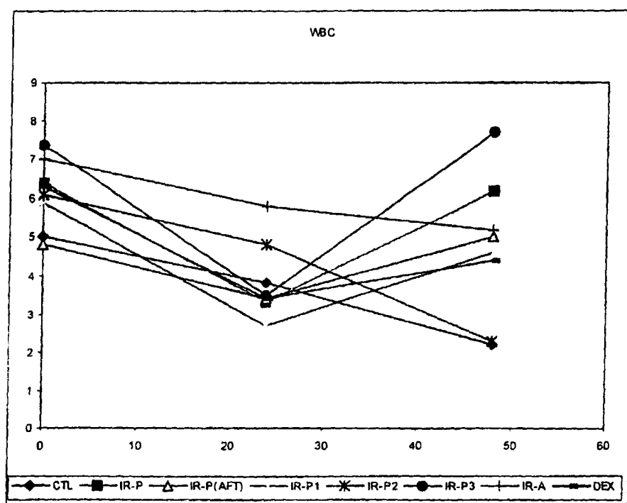
Figure 63 Our results show that mice treated with IR-A, IR-P and its fractions have moderate to normal level of WBC at t=48 hours then the control and dexamethasone treated mice, suggesting less inflammatory responses in IR treated mice.
