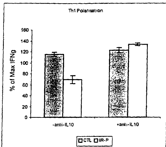
Figure 38 shows an increase in IFN-gamma production in Th1 polarization conditions in IR-P group, which suggests that the promoting effect of IR-P on Th2 subset is at least IL-10 dependent (for detail see text).
