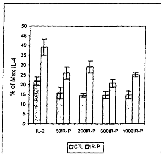
figure 37 shows that CD4 + T cells from PBS and IR-P mice treated (in vivo) with different doses of IR-P (in vitro) show decrease in IL-4 production which suggest the shift towards Th1 phenotype (see also figure 36).
