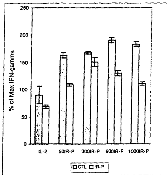
Figure 36 shows that CD4 + T cells from PBS and IR-P mice treated (in vivo) with different doses of IR-P (in vitro) show increase in IFN-gamma production which suggest the shift towards Th1 phenotype (see also figure 37).
