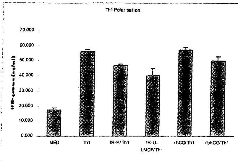
Figure 28. This figure shows that there is strong inhibition of IFN-gamma production found with IR-P and IR-U/LMDF on CD4+ cells polarizing towards Th1 phenotype (in vivo). There was only a moderate inhibition of IFN-gamma production observed with recombinant beta-hCG and no effect was seen with recombinant hCG as compare to control (MED).
