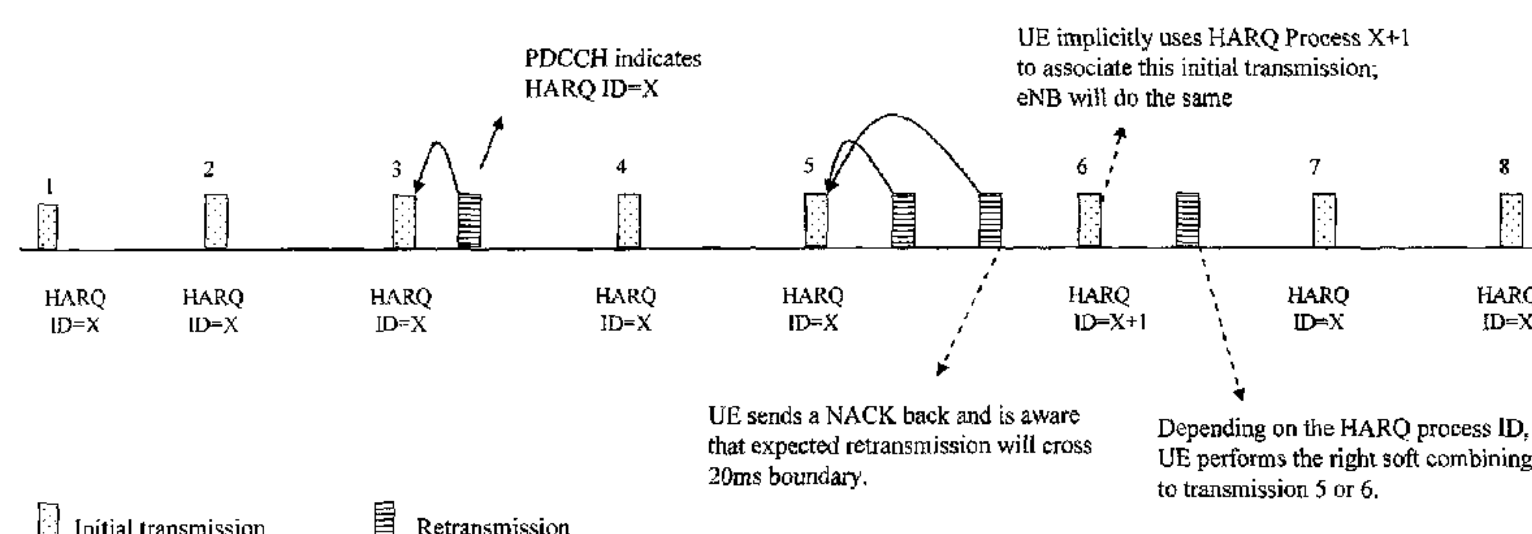
Figure 8c. Implicit dynamic assignment for the additional HARQ process to resolve the second case
