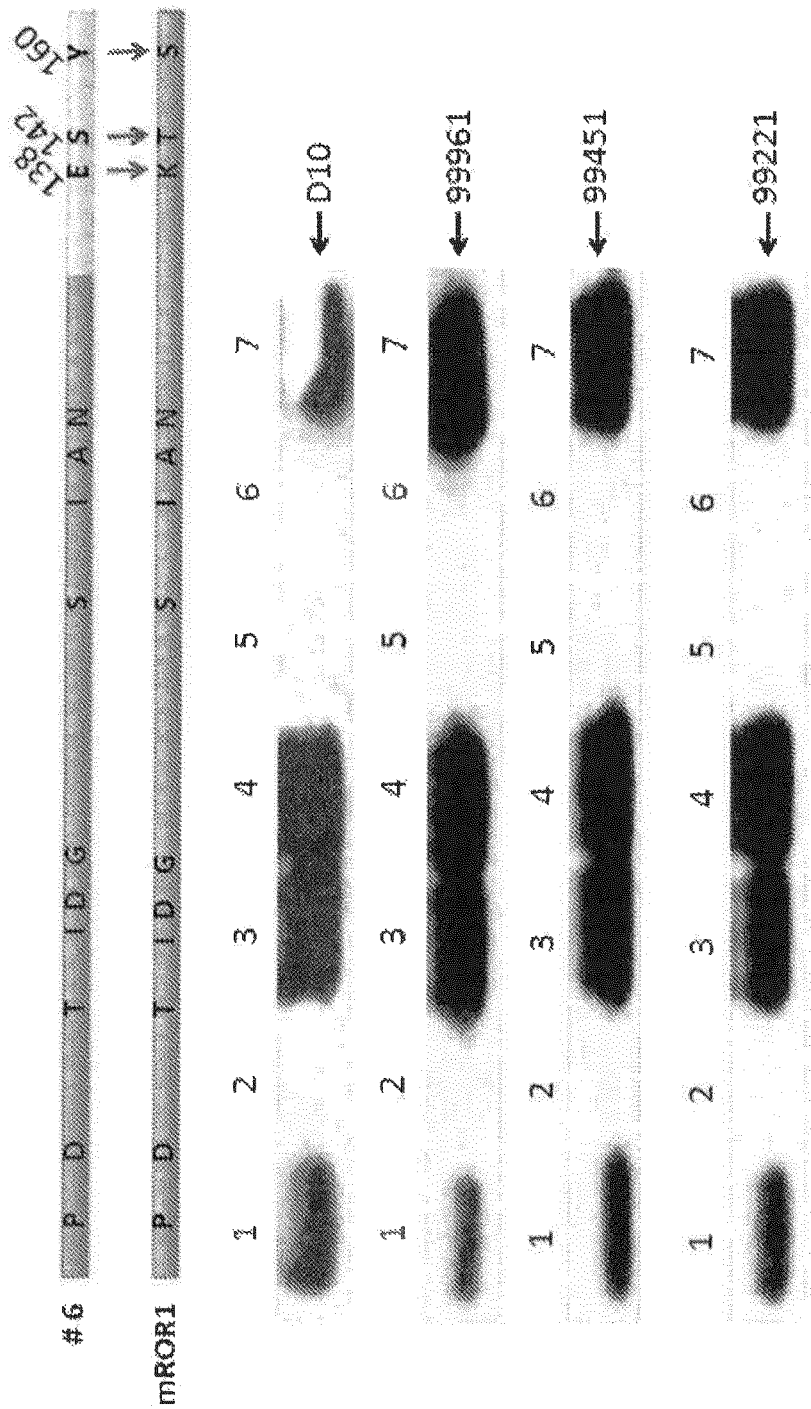
1. HuROR1 2. HuROR1 With E->K @138 3. HuROR1 With S->T @142 4. HuROR1 With Y->S @160 5. HuROR1 With E->K @138 & S->T @142 6. HuROR1 With E->K @138 & Y->S @160 7. HuROR1 With S->T @142 & Y->S @160
