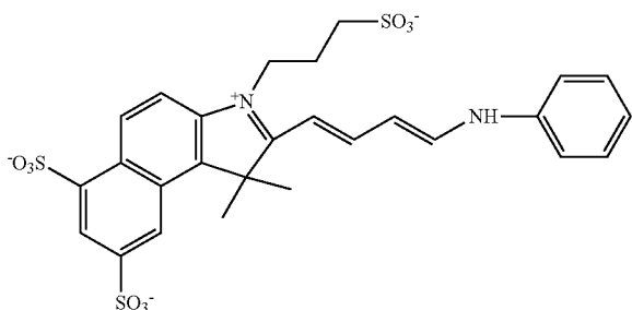
Compound 28
