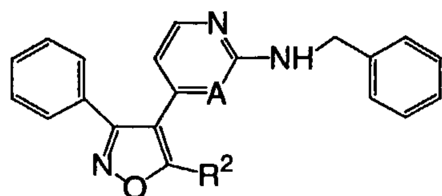
IVA-1 ( R^2=CH_3 )
