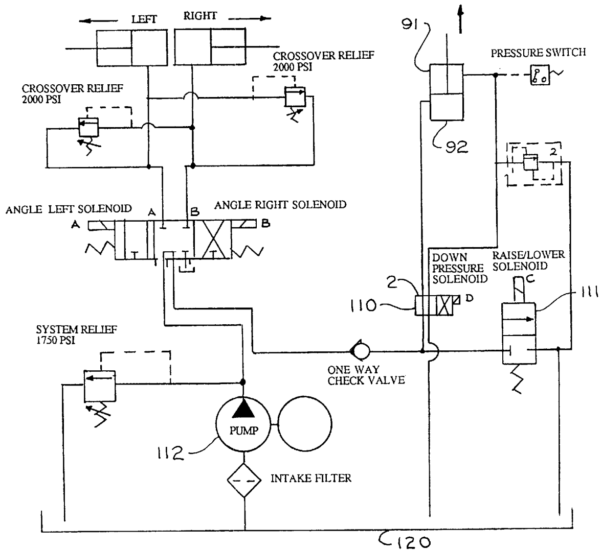
RAISE &amp; HOLD HYDRAULIC SYSTEM SCHEMATIC
