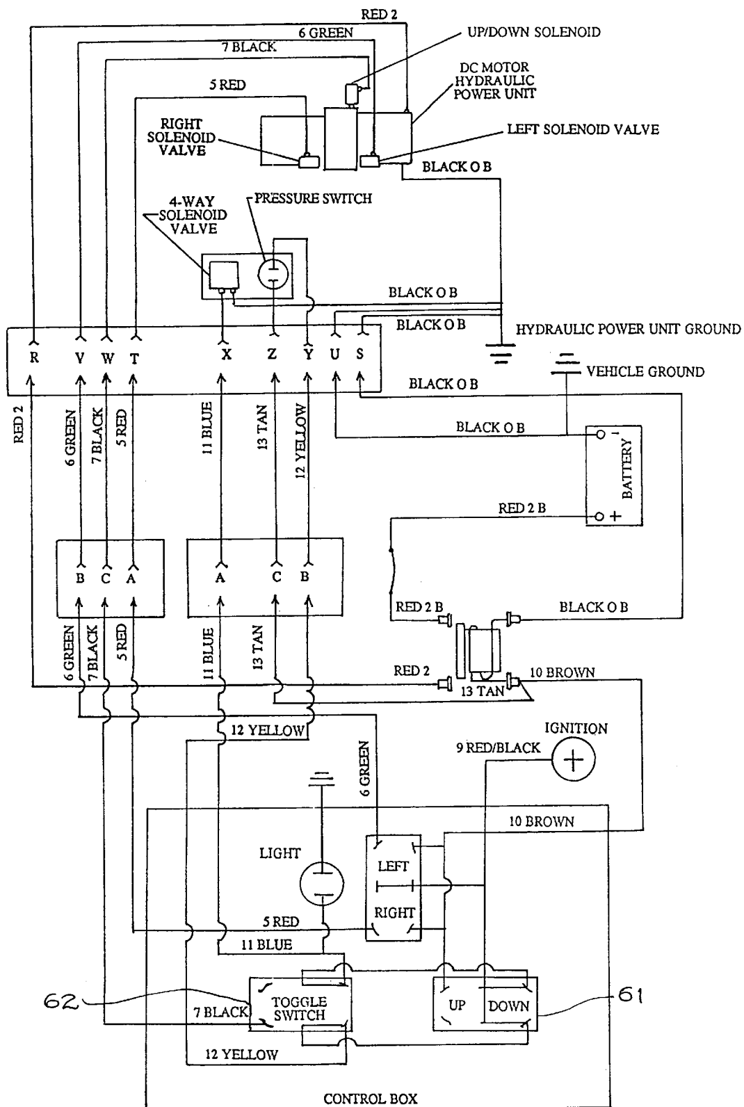
PRESSURE DOWN WIRING SCHEMATIC
