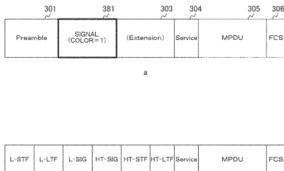
EXAMPLE OF PHYSICAL HEADER IN TWELFTH EMBODIMENT
