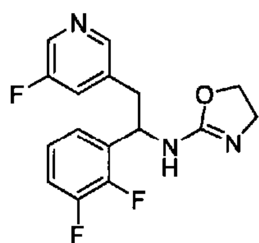
N-(1-(2, 3-Difluorophenyl)-2-(5-fluoropyridin-3-yl)ethyl)-4,5-dihydrooxazol-2-amine
