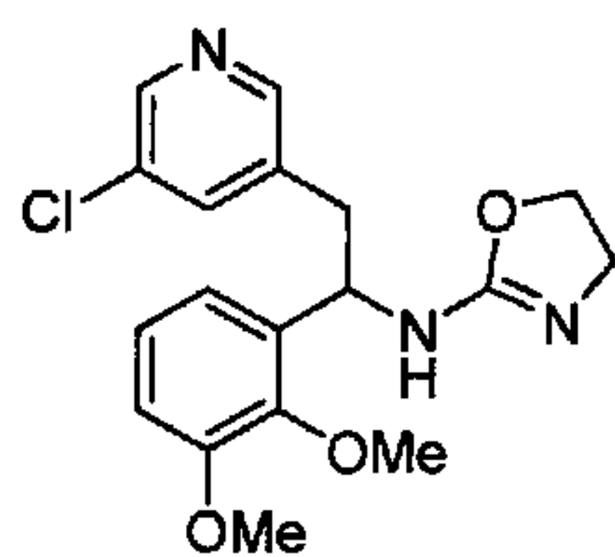
N-(2-(5-Chloropyridin-3-yl)-(1,2,3-dimethoxyphenyl)ethyl)-4,5-dihydrooxazol-2-amine
