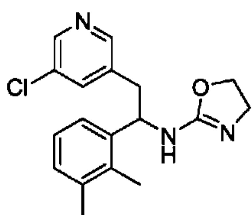
N-(2-(5-Chloropyridin-3-yl)-(1-(2,3-dimethylphenyl)ethyl)-4,5-dihydrooxazol-2-amine
