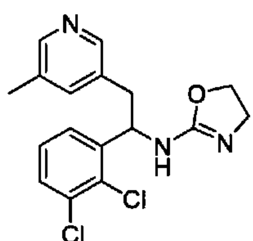
N-(1-(2,3-Dichlorophenyl)-2-(5-methylpyridin-3-yl)ethyl)-4,5-dihydrooxazol-2-amine
