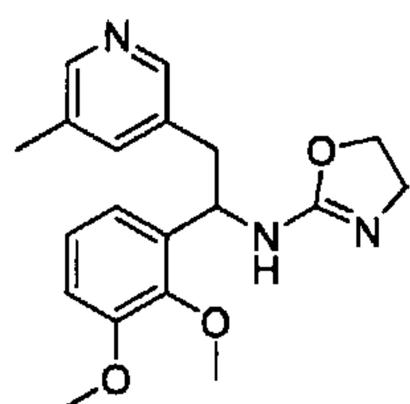
N-(1-(2,3-Dimethoxyphenyl)-2-(5-methylpyridin-3-yl)ethyl)-4,5-dihydrooxazol-2-amine
