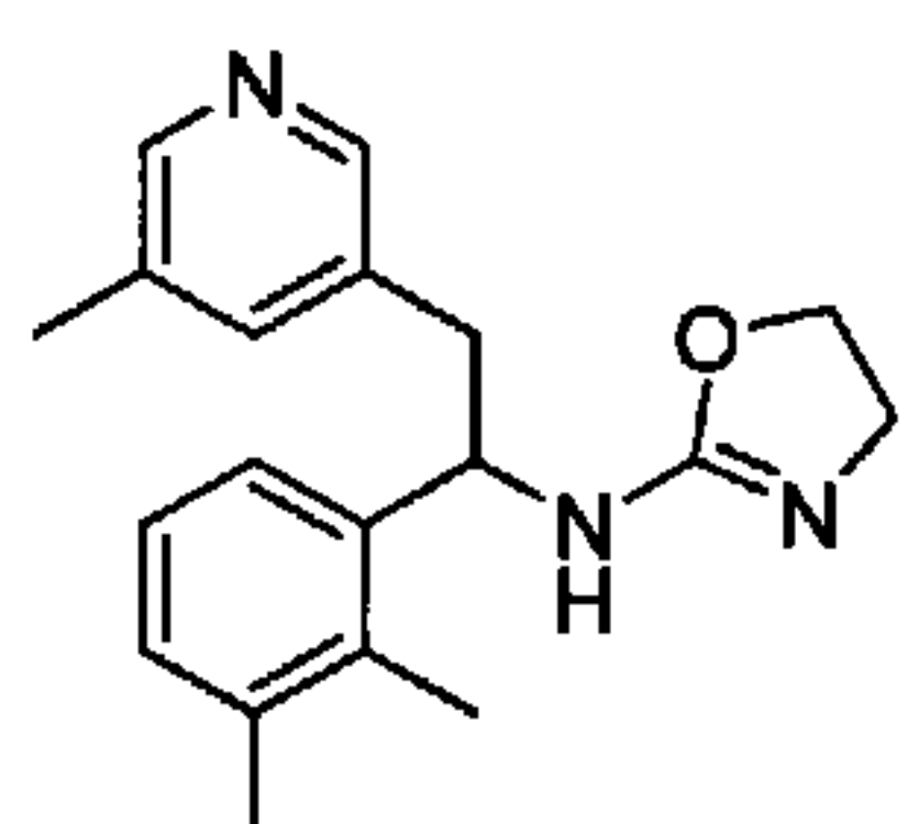
N-(1-(2,3-Dimethylphenyl)-2-(5-methylpyridin-3-yl)ethyl)-4,5-dihydrooxazol-2-amine
