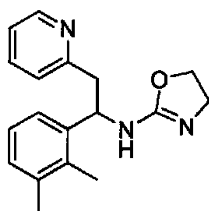
N-(1-(2,3-Dimethylphenyl)-2-(pyridin-2-yl)ethyl)-4,5-dihydrooxazol-2-amine
