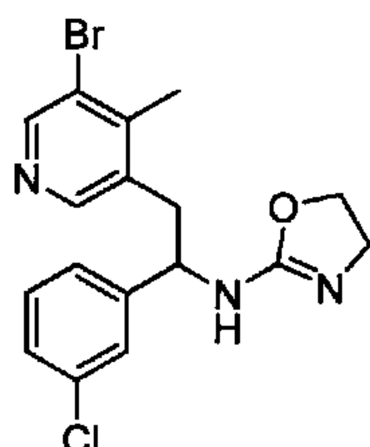
N-(2-(5-Bromo-4-methylpyridin-3-yl)-1-(3-chlorophenyl)ethyl)-4,5-
