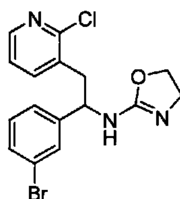
N-(1-(3-Bromophenyl)-2-(2-chloropyridin-3-yl)ethyl)-4,5-dihydrooxazol-2-amine
