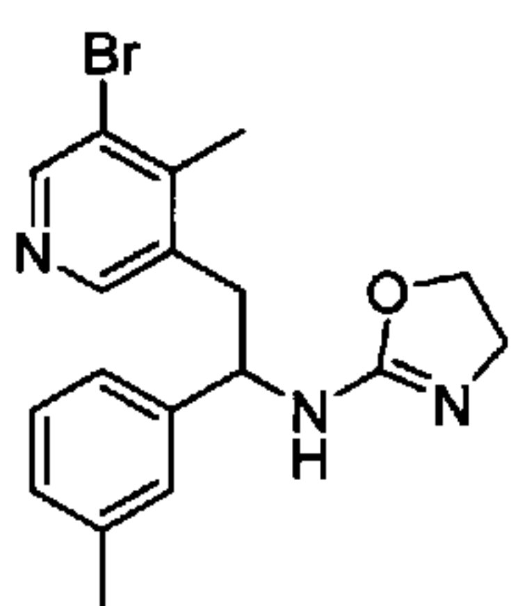
N-(2-(5-Bromo-4-methylpyridin-3-yl)-1-m-tolylethyl)-4,5-dihydrooxazol-2-amine
