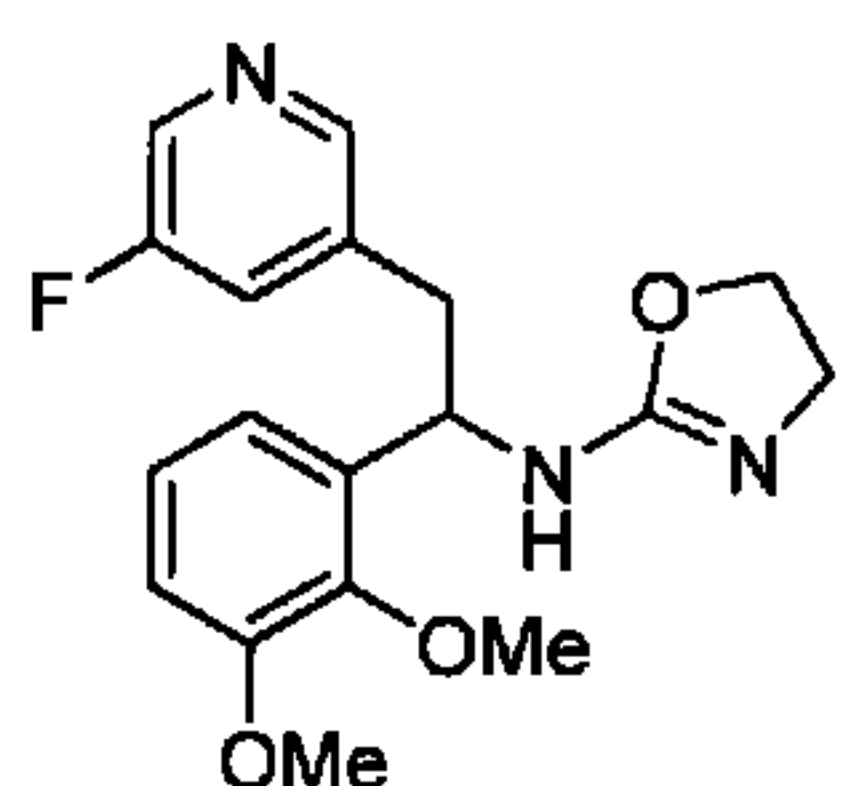
N-(1-(2, 3-Dimethoxyphenyl)-2-(5-fluoropyridin-3-yl)ethyl)-4,5-dihydrooxazol-2-amine
