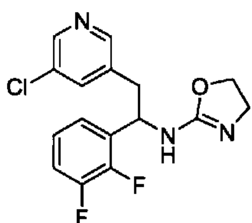
N-(2-(5-Chloropyridin-3-yl)-(1-(2,3-difluorophenyl)ethyl)-4,5-dihydrooxazol-2-amine
