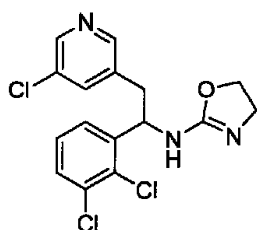
N-(2-(5-Chloropyridin-3-yl)-(1-(2,3-dichlorophenyl)ethyl)-4,5-dihydrooxazol-2-amine
