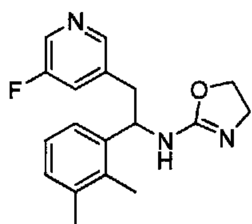
N-(1-(2,3-Dimethylphenyl)-2-(5-fluoropyridin-3-yl)ethyl)-4,5-dihydrooxazol-2-amine
