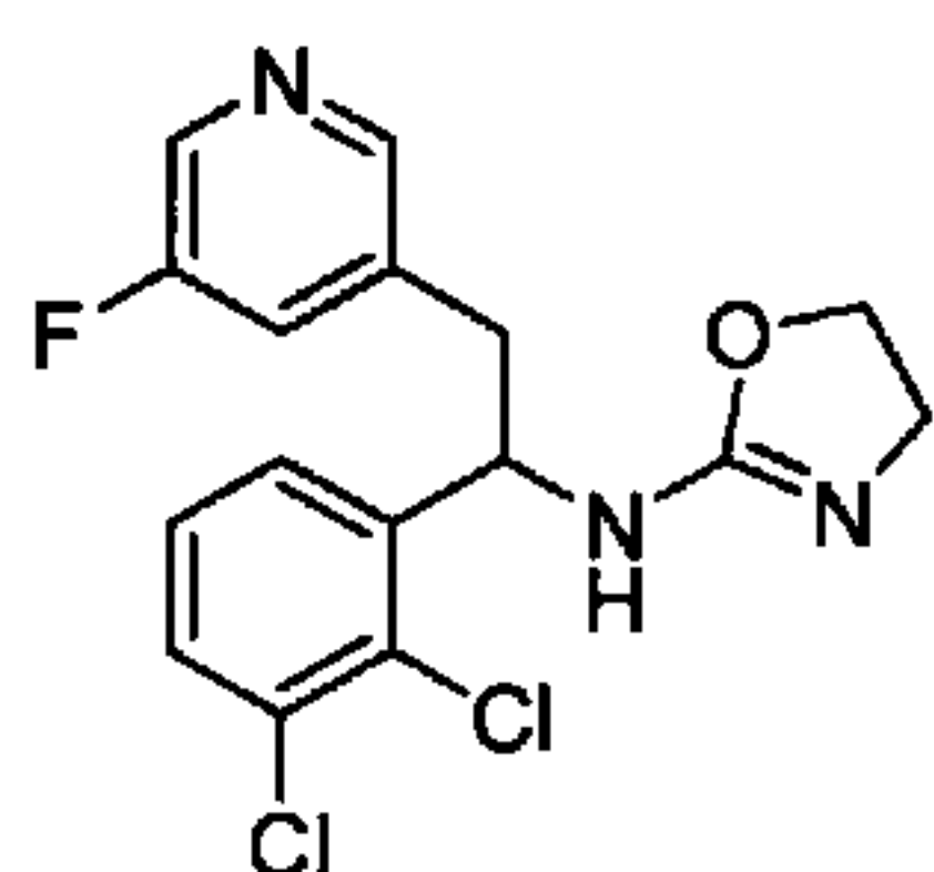
N-(1-(2,3-Dichlorophenyl)-2-(5-fluoropyridin-3-yl)ethyl)-4,5-dihydrooxazol-2-amine
