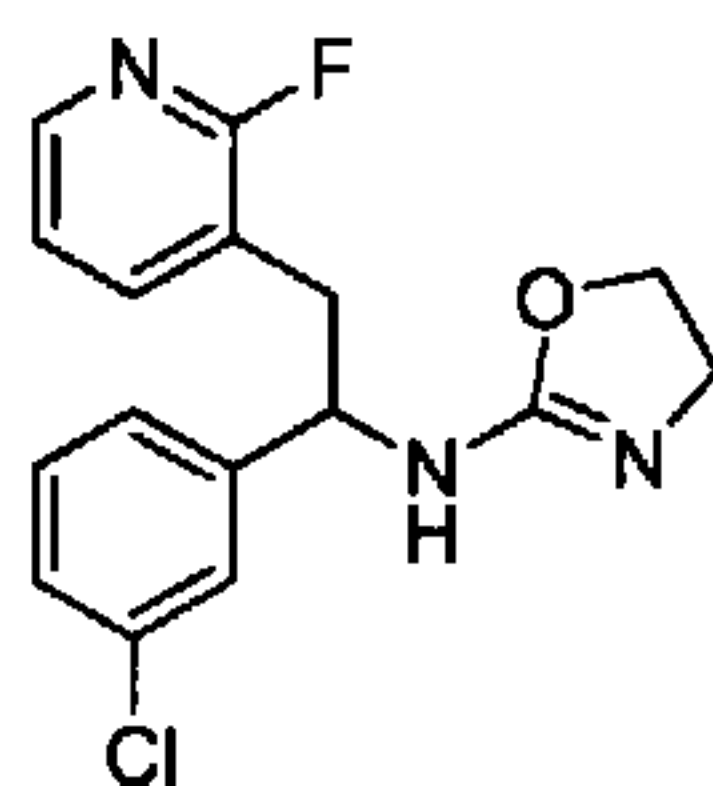
N-(1-(3-Chlorophenyl)-2-(2-fluoropyridin-3-yl)ethyl)-4,5-dihydrooxazol-2-amine
