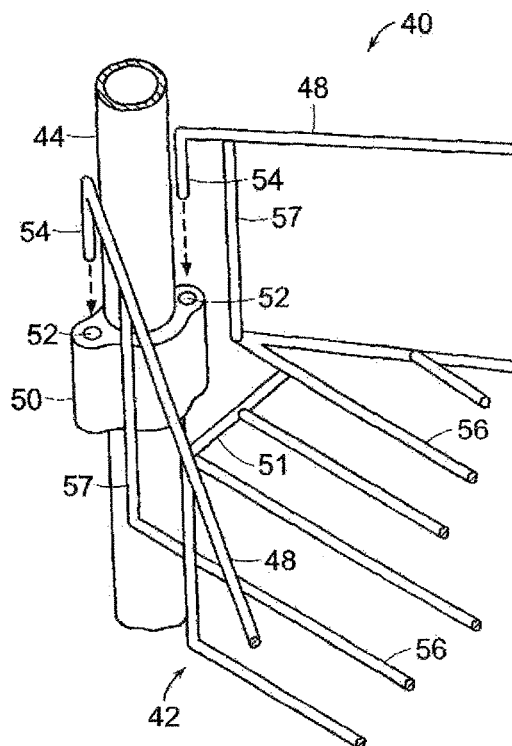
FIG. 2 PRIOR ART
