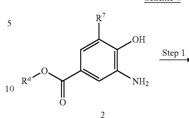
Scheme 4
