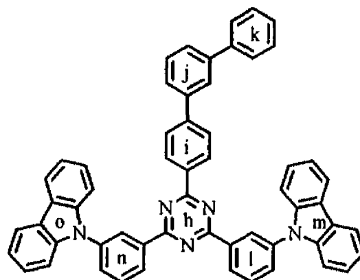
Compound 9 (Compound \alpha 2; degree of identity, 86%)
