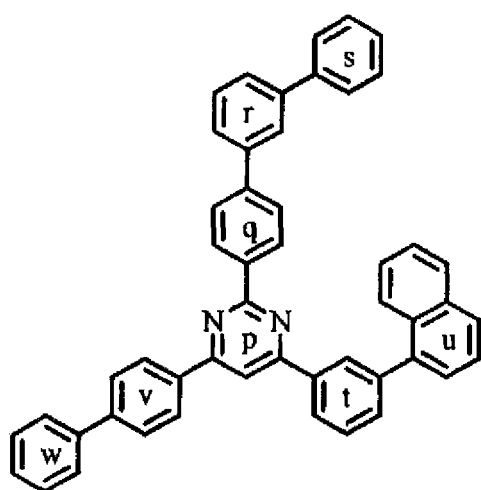
Compound 10 (Compound \alpha 3; degree of identity, 57%)
