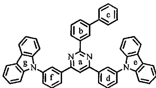
Compound 8 (Compound \alpha 1)
