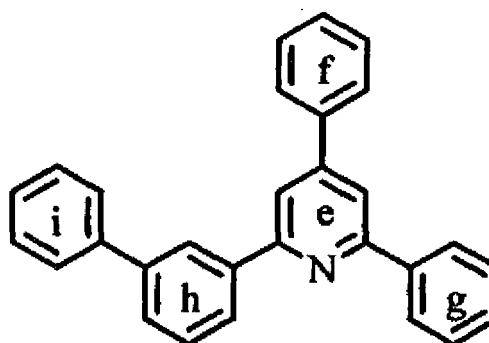
Compound 2 (Compound \alpha 2 ; degree of identity, 100%)
