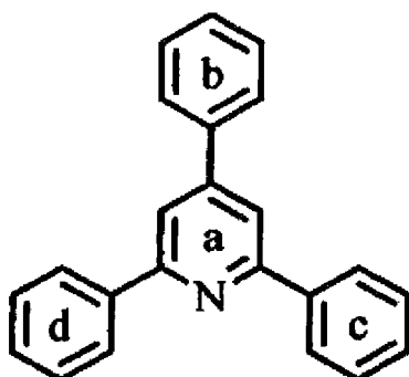
Compound 1 (Compound \alpha 1 )
