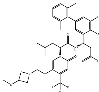
(S)-3-(5-chloro-4-fluoro-2',6'-dimethyl-[1,1'-biphenyl]-3-yl)-3-(S)-2-(5-(2-(3-methoxyazetidin-1-yl)ethyl)-2-oxo-4-(trifluoromethyl)pyridin-1(2H)-yl)-4-methylpentanamido)propanoic acid;
