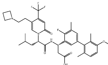
(S)-3-((S)-2-(5-(2-(azetidin-1-yl)ethyl)-2-oxo-4-(trifluoromethyl)pyridin-1(2H)-yl)-4-methylpentanamido)-3-(4-fluoro-3'-methoxy-2',5,6'-trimethyl-[1,1'-biphenyl]-3-yl)propanoic acid
