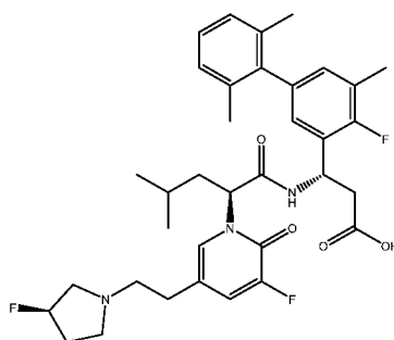
(S)-3-(4-fluoro-2',5,6'-trimethyl-[1,1'-biphenyl]-3-yl)-3-(S)-2-(3-fluoro-5-(2-(R)-3-fluoropyrrolidin-1-yl)ethyl)-2-oxopyridin-1(2H)-yl)-4-methylpentanamido)propanoic acid
