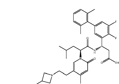
(S)-3-(4,5-difluoro-2',6'-dimethyl-[1,1'-biphenyl]-3-yl)-3-((S)-2-(5-(2-(3-fluoroazetidin-1-yl)ethyl)-2-oxopyridin-1(2H)-yl)-4-methylpentanamido)propanoic acid
