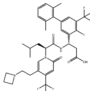
(S)-3-((S)-2-(5-(2-(azetidin-1-yl)ethyl)-2-oxo-4-(trifluoromethyl)pyridin-1(2H)-yl)-4-methylpentanamido)-3-(4-fluoro-2',6'-dimethyl-5-(trifluoromethyl)-[1,1'-biphenyl]-3-yl)propanoic acid
