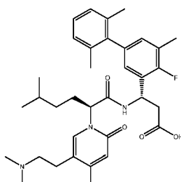
(S)-3-(S)-2-(5-(2-(dimethylamino)ethyl)-4-methyl-2-oxopyridin-1(2H)-yl)-5-methylhexanamido)-3-(4-fluoro-2',5,6'-trimethyl-[1,1'-biphenyl]-3-yl)propanoic acid;
