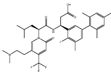
(S)-3-(S)-2-(5-(2-(dimethylamino)ethyl)-2-oxo-4-(trifluoromethyl)pyridin-1(2H)-yl)-4-methylpentanamido)-3-(4-fluoro-2',4',5,6'-tetramethyl-[1,1'-biphenyl]-3-yl)propanoic acid;
