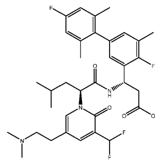
(S)-3-(4,4'-difluoro-2',5,6'-trimethyl-[1,1'-biphenyl]-3-yl)-3-(S)-2-(3-(difluoromethyl)-5-(2-(dimethylamino)ethyl)-2-oxopyridin-1(2H)-yl)-4-methylpentanamido)propanoic acid;
