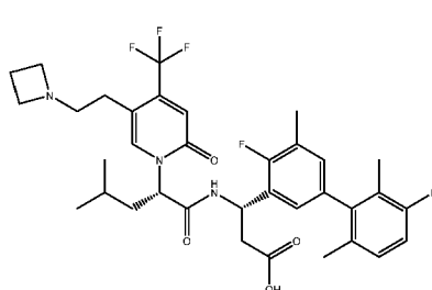
(S)-3-((S)-2-(5-(2-(azetidin-1-yl)ethyl)-2-oxo-4-(trifluoromethyl)pyridin-1(2H)-yl)-4-methylpentanamido)-3-(3',4'-difluoro-2',5,6'-trimethyl-[1,1'-biphenyl]-3-yl)propanoic acid
