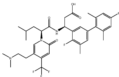
(S)-3-(4,4'-difluoro-2',5,6'-trimethyl-[1,1'-biphenyl]-3-yl)-3-(S)-2-(5-(2-(dimethylamino)ethyl)-2-oxo-4-(trifluoromethyl)pyridin-1(2H)-yl)-4-methylpentanamido)propanoic acid;
