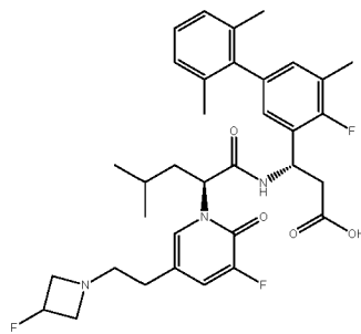
(S)-3-(4-fluoro-2',5,6'-trimethyl-[1,1'-biphenyl]-3-yl)-3-(S)-2-(3-fluoro-5-(2-(3-fluoroazetidin-1-yl)ethyl)-2-oxopyridin-1(2H)-yl)-4-methylpentanamido)propanoic acid
