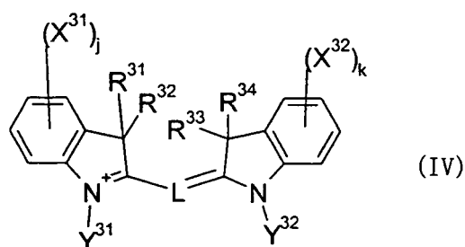
[Chem. 12-1]
