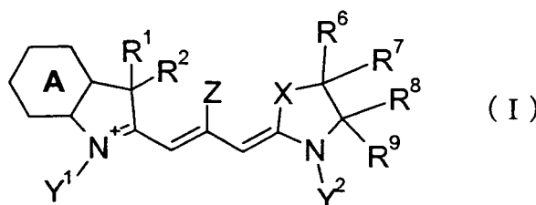
[Chem. 1]
