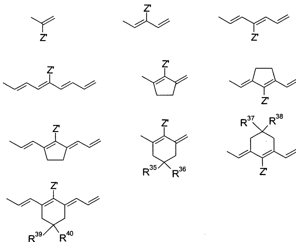
[Chem. 12-2]
