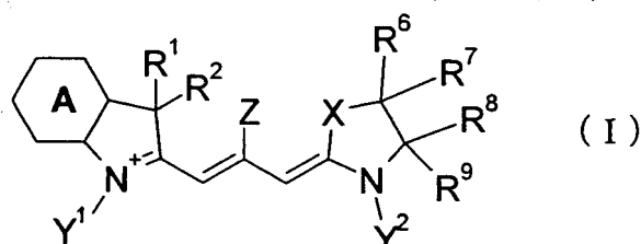
[Chem. 1]
