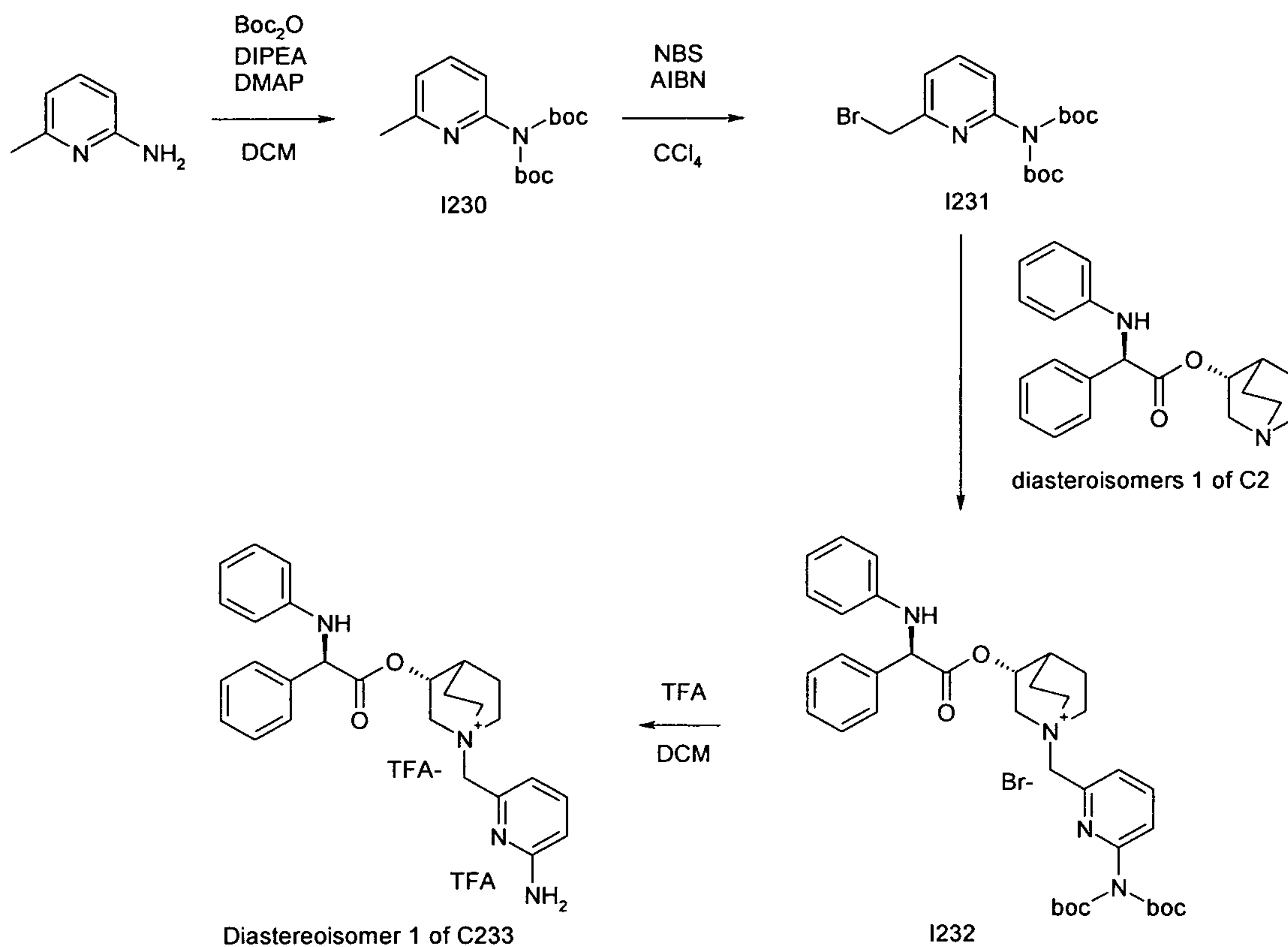
Scheme 53
