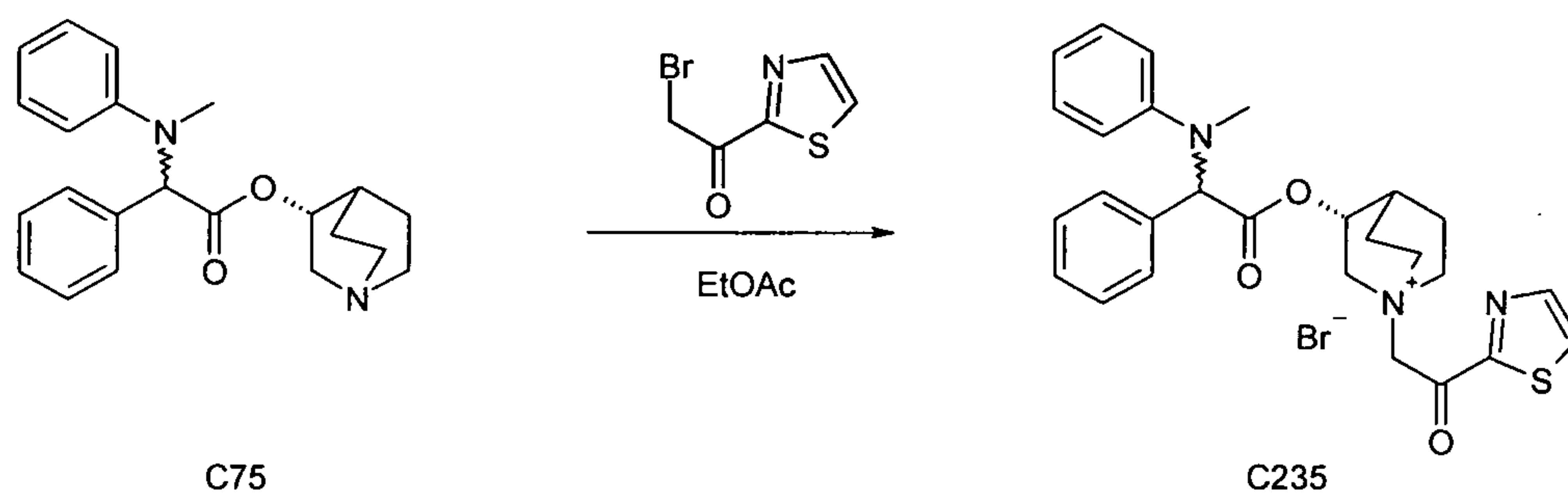
Scheme 55
