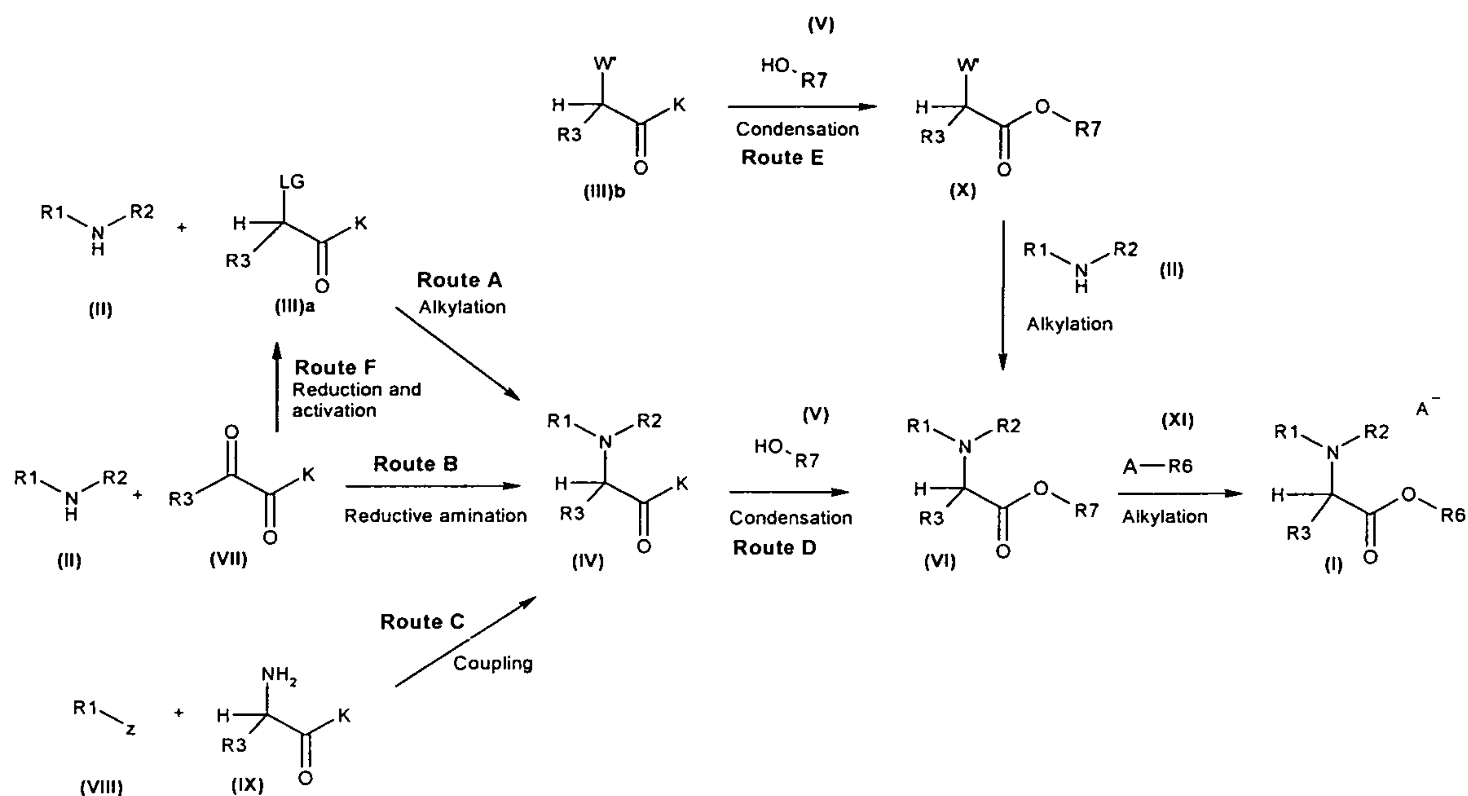
Scheme 1
