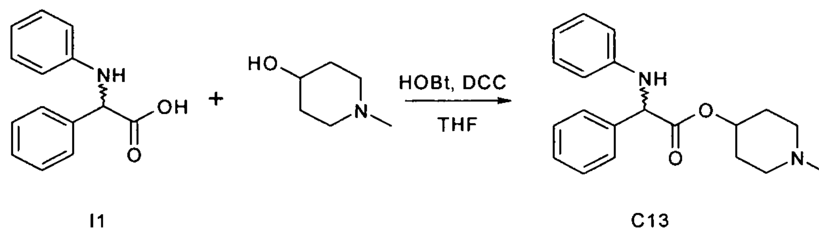
Scheme 5
