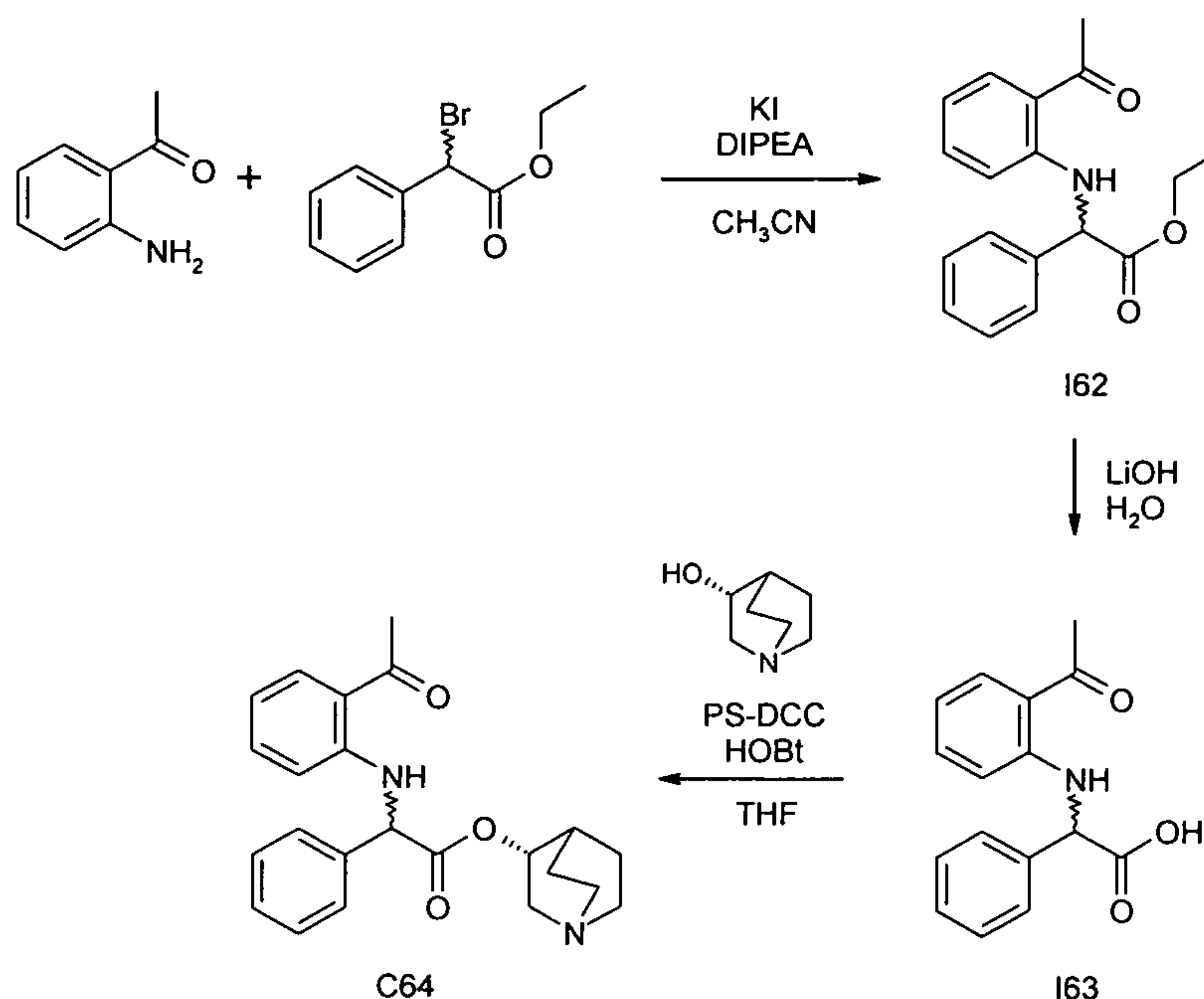
Scheme 24
