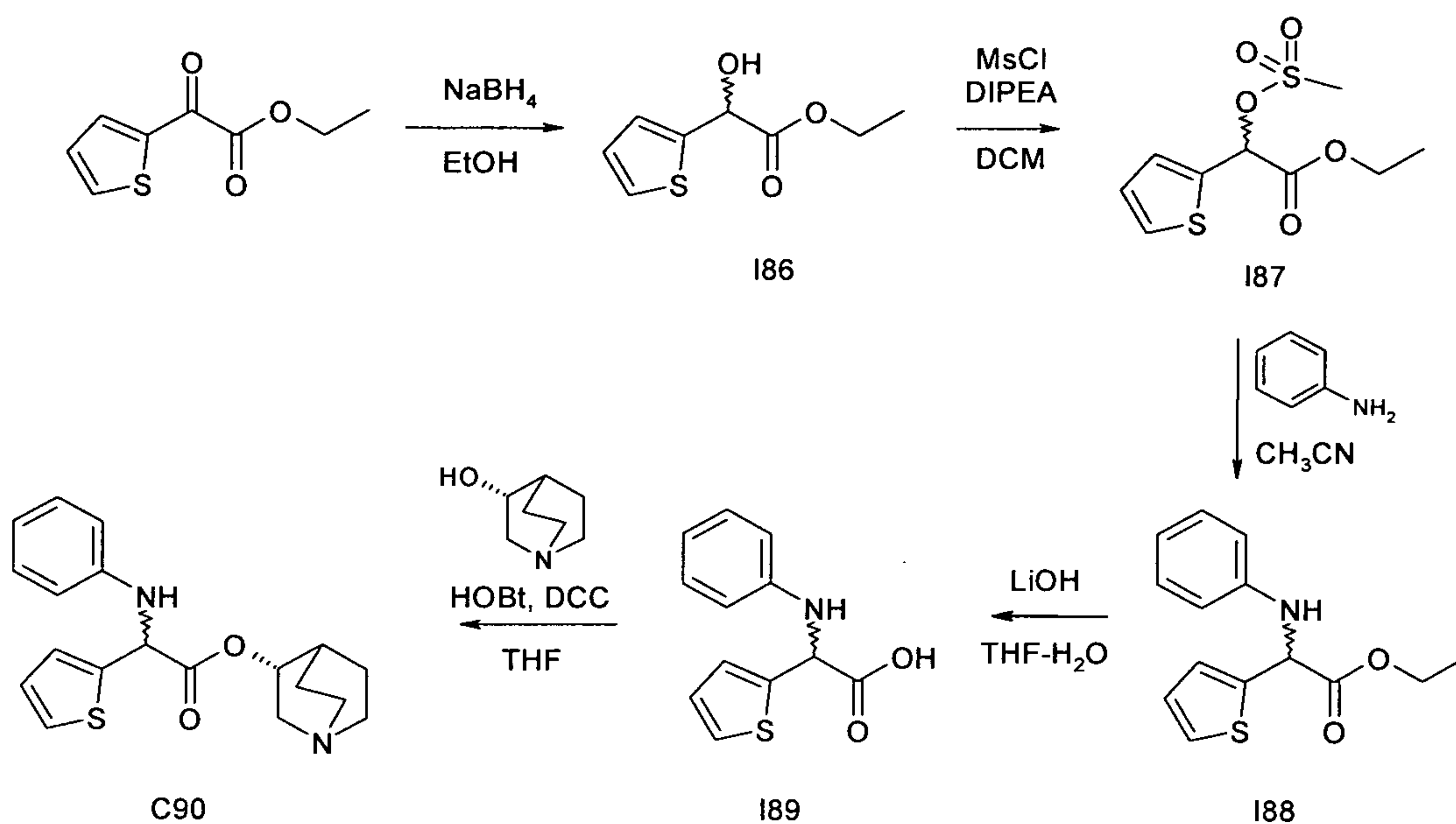
Scheme 32
