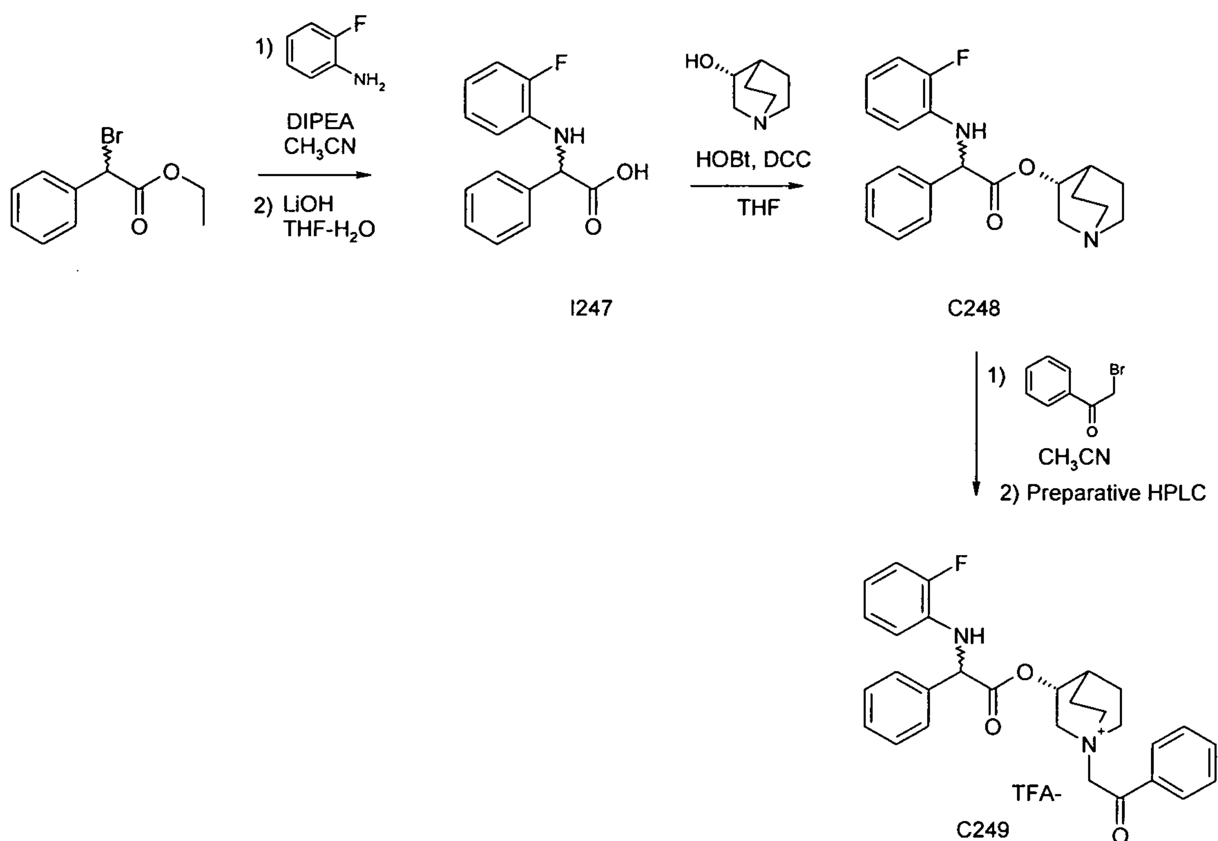
Scheme 64
