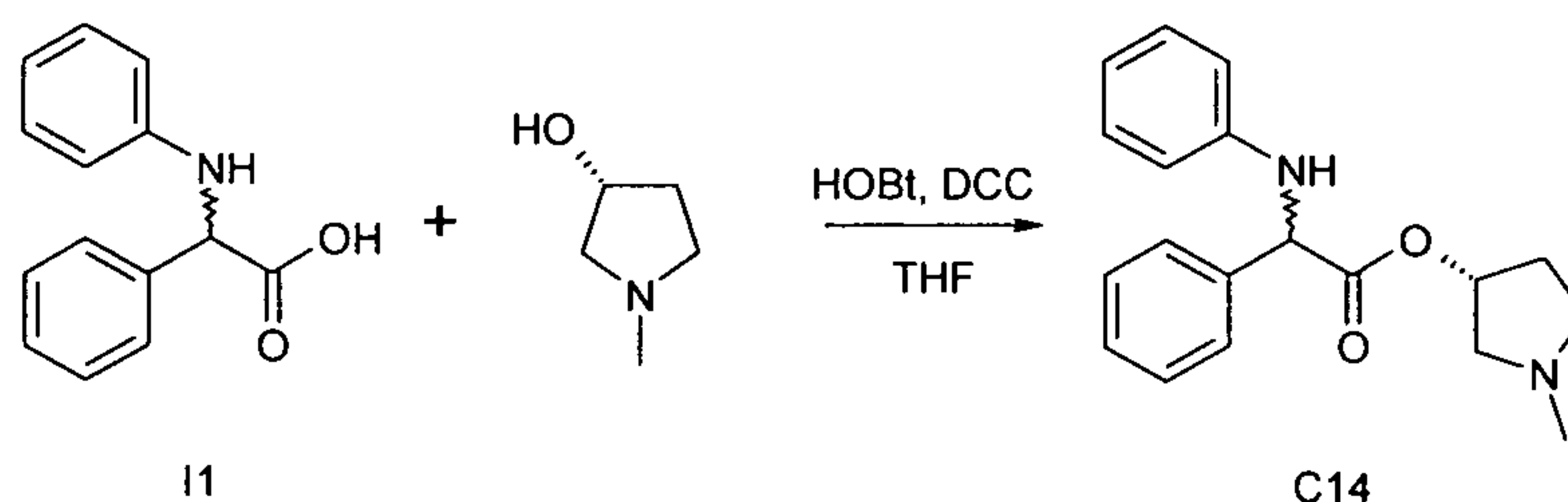
Scheme 6
