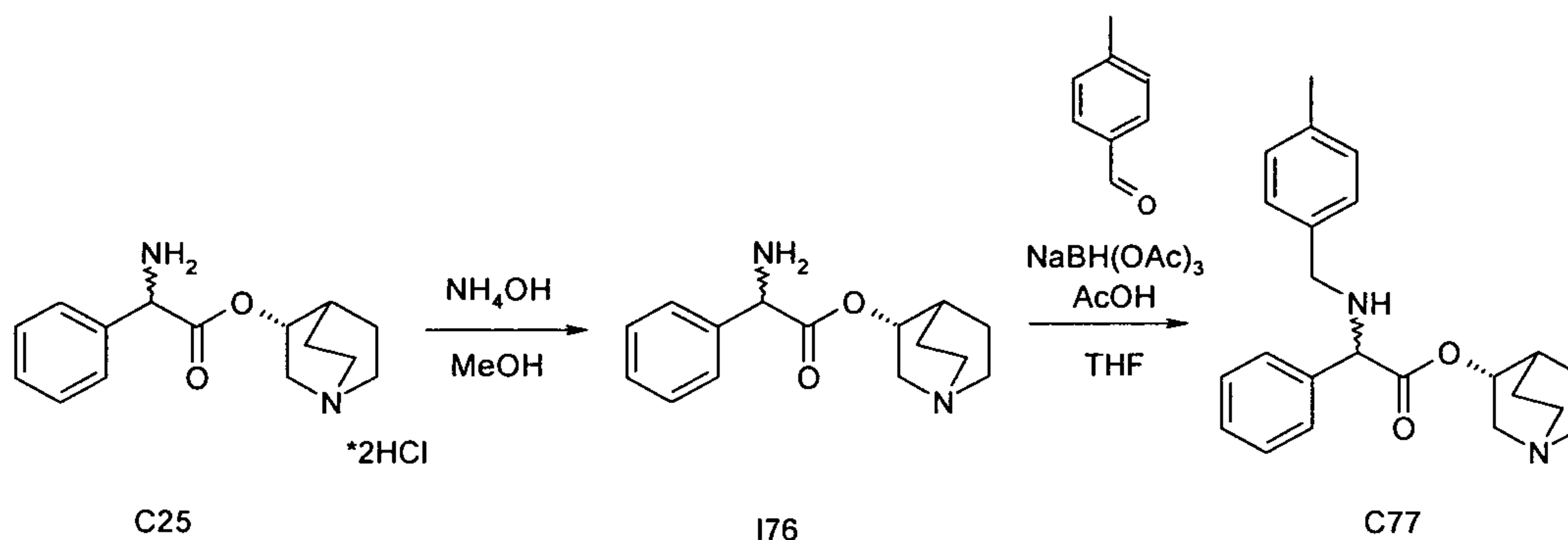
Scheme 29
