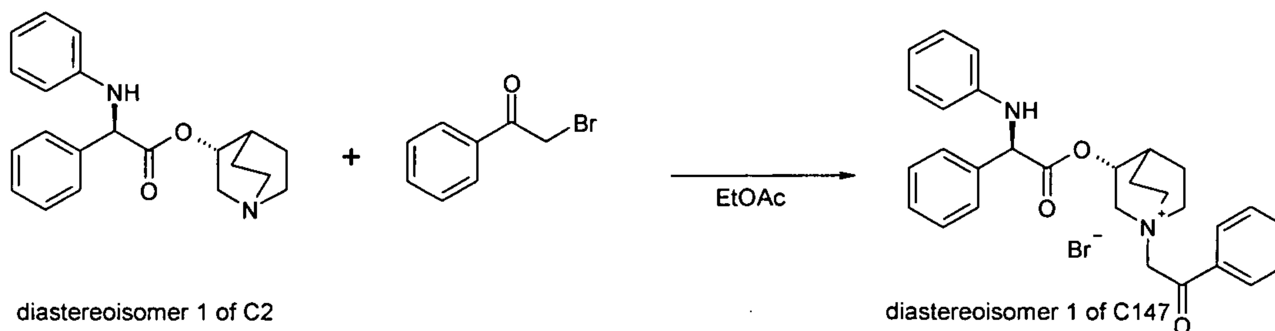
Scheme 41
