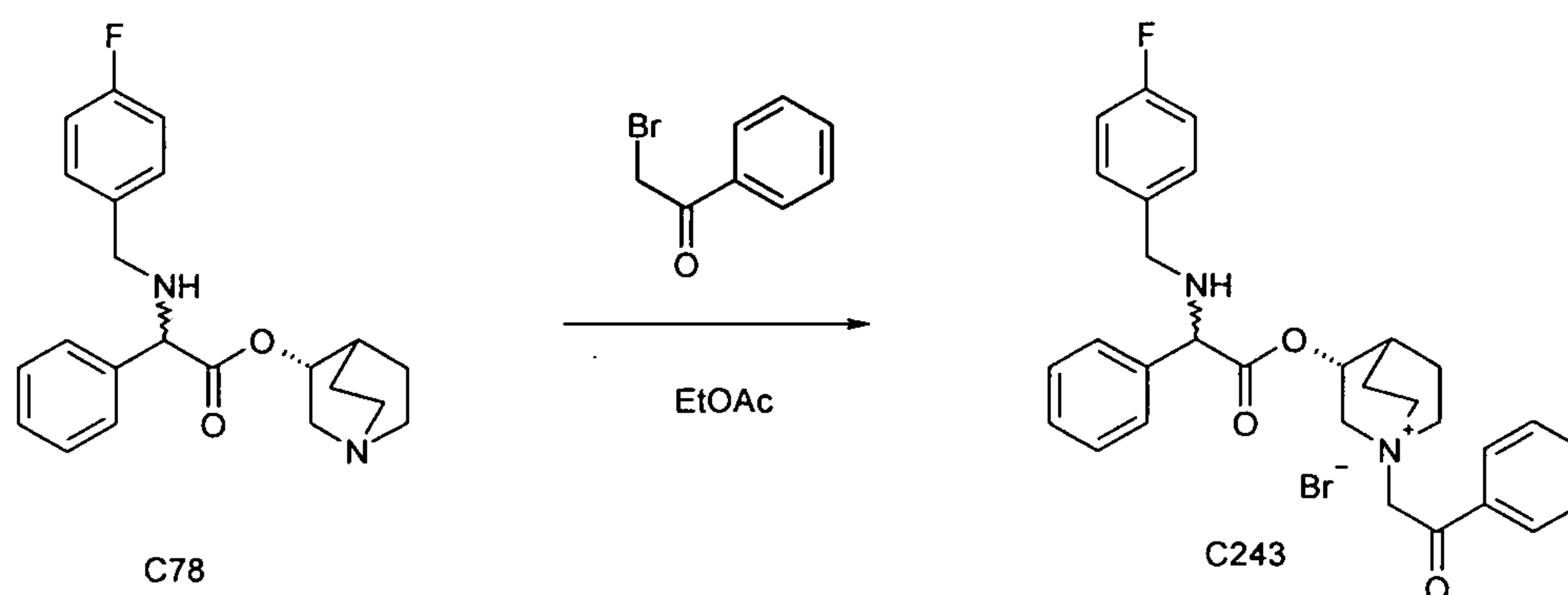
Scheme 62
