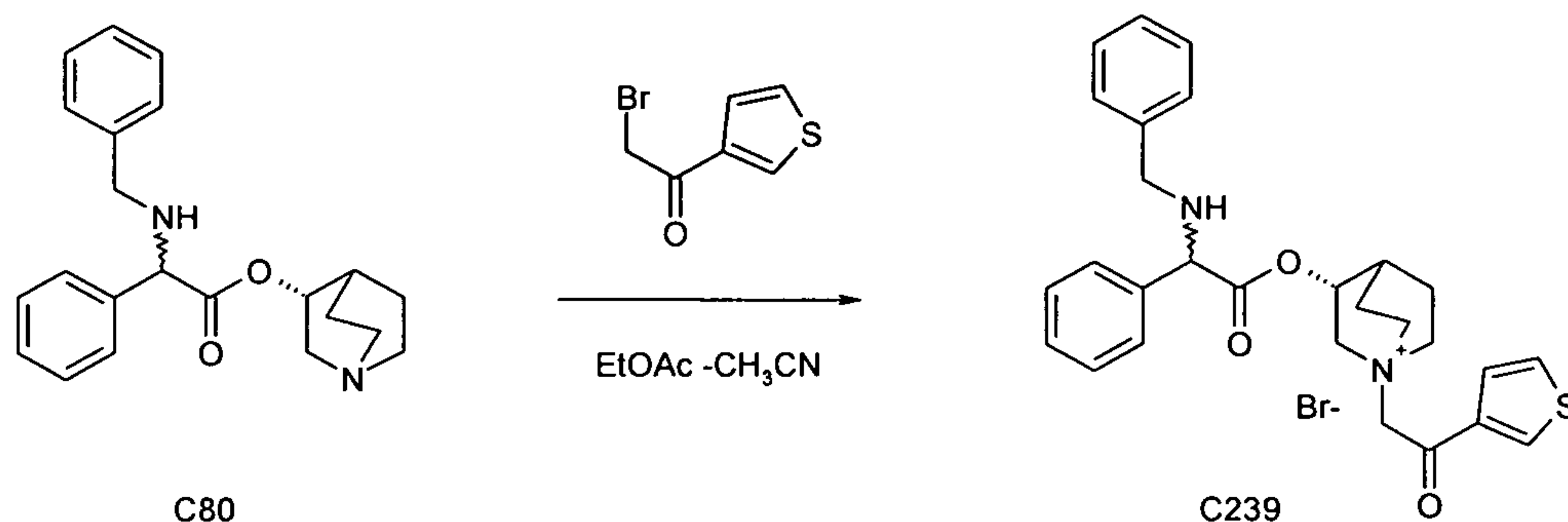
Scheme 58
