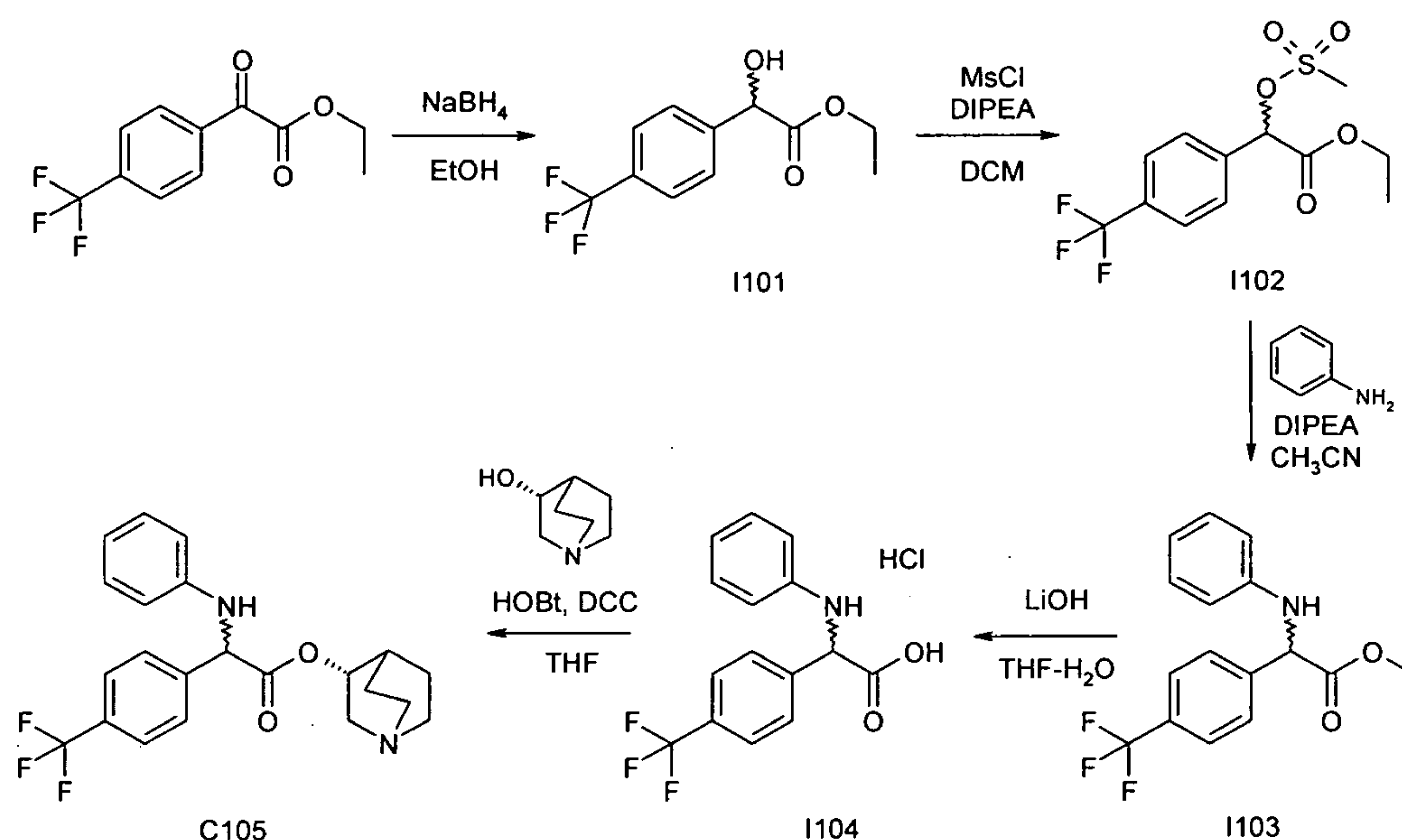
Scheme 36
