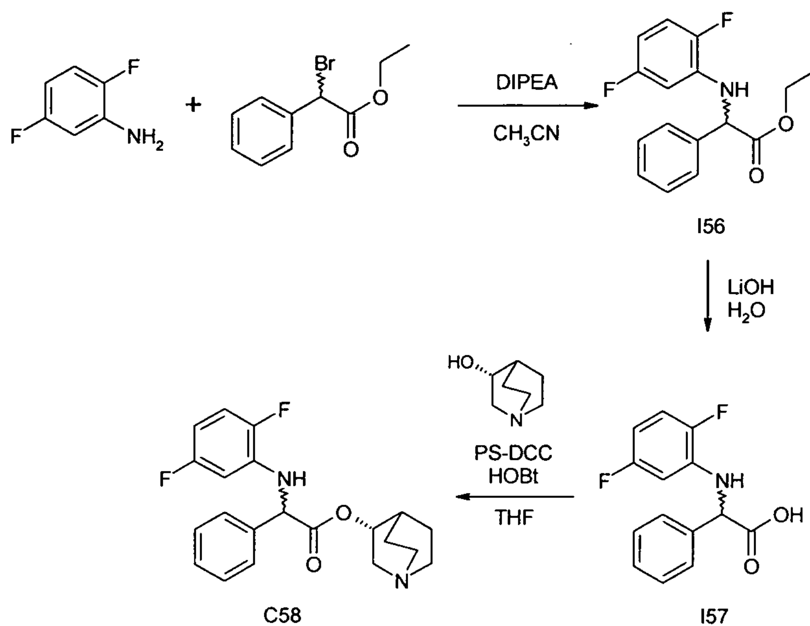
Scheme 22
