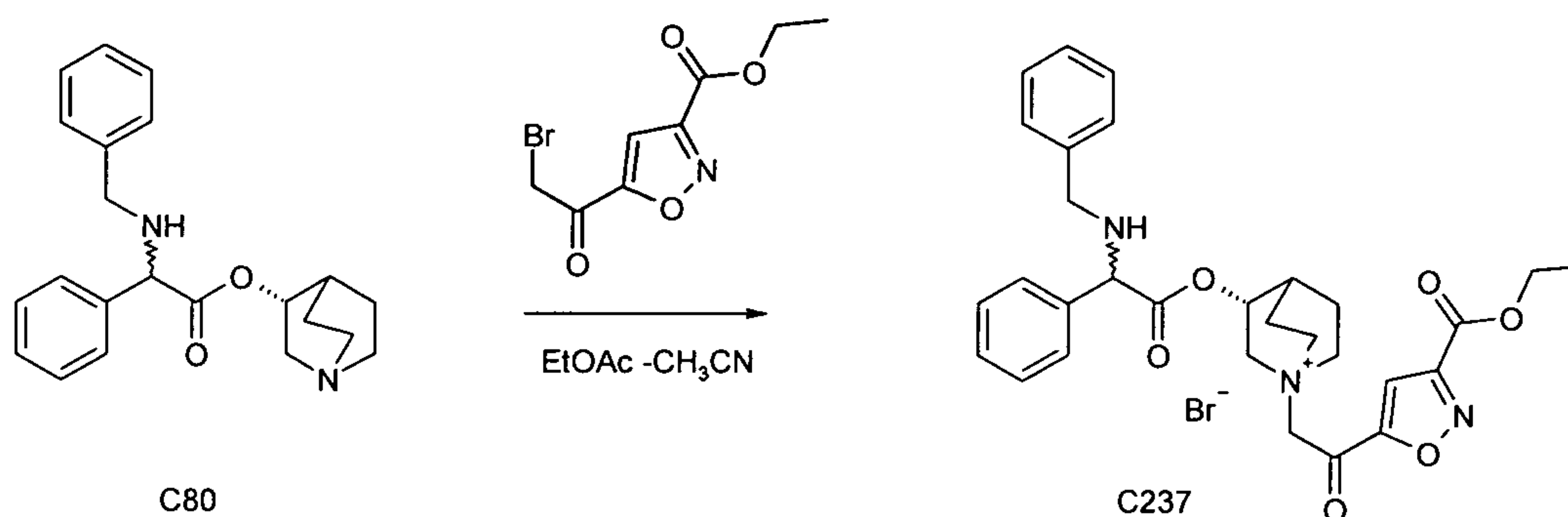
Scheme 56
