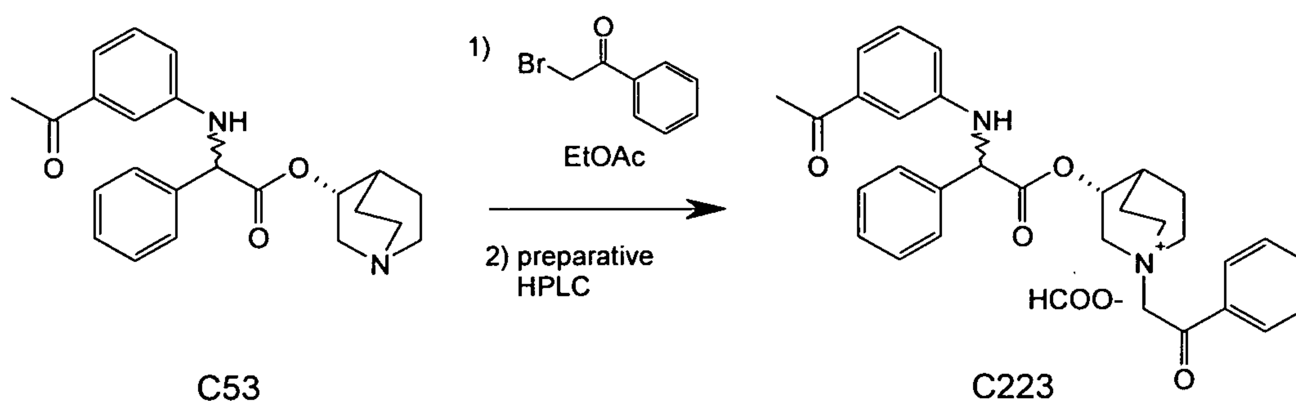
Scheme 49
