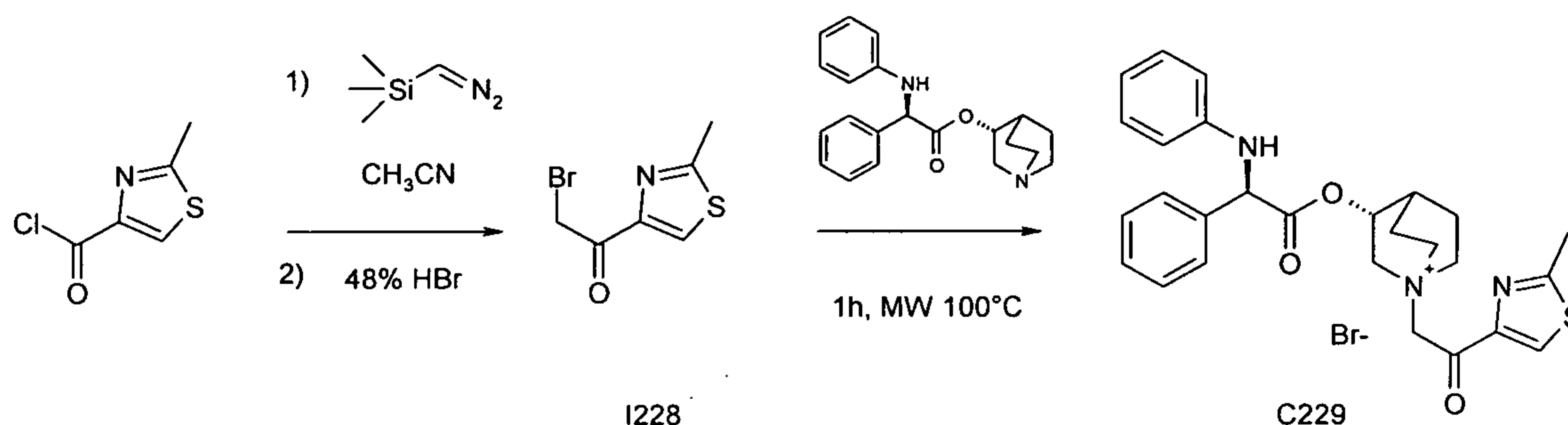
Scheme 52
