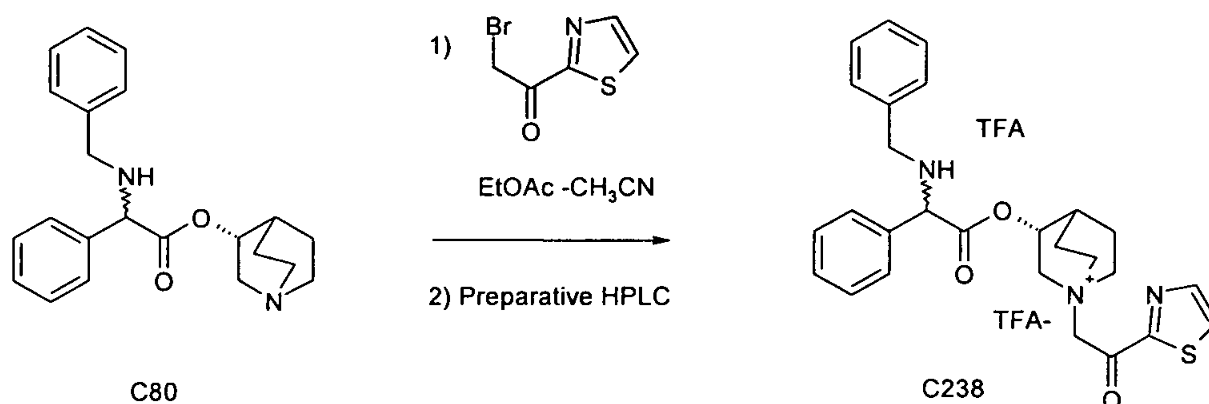
Scheme 57
