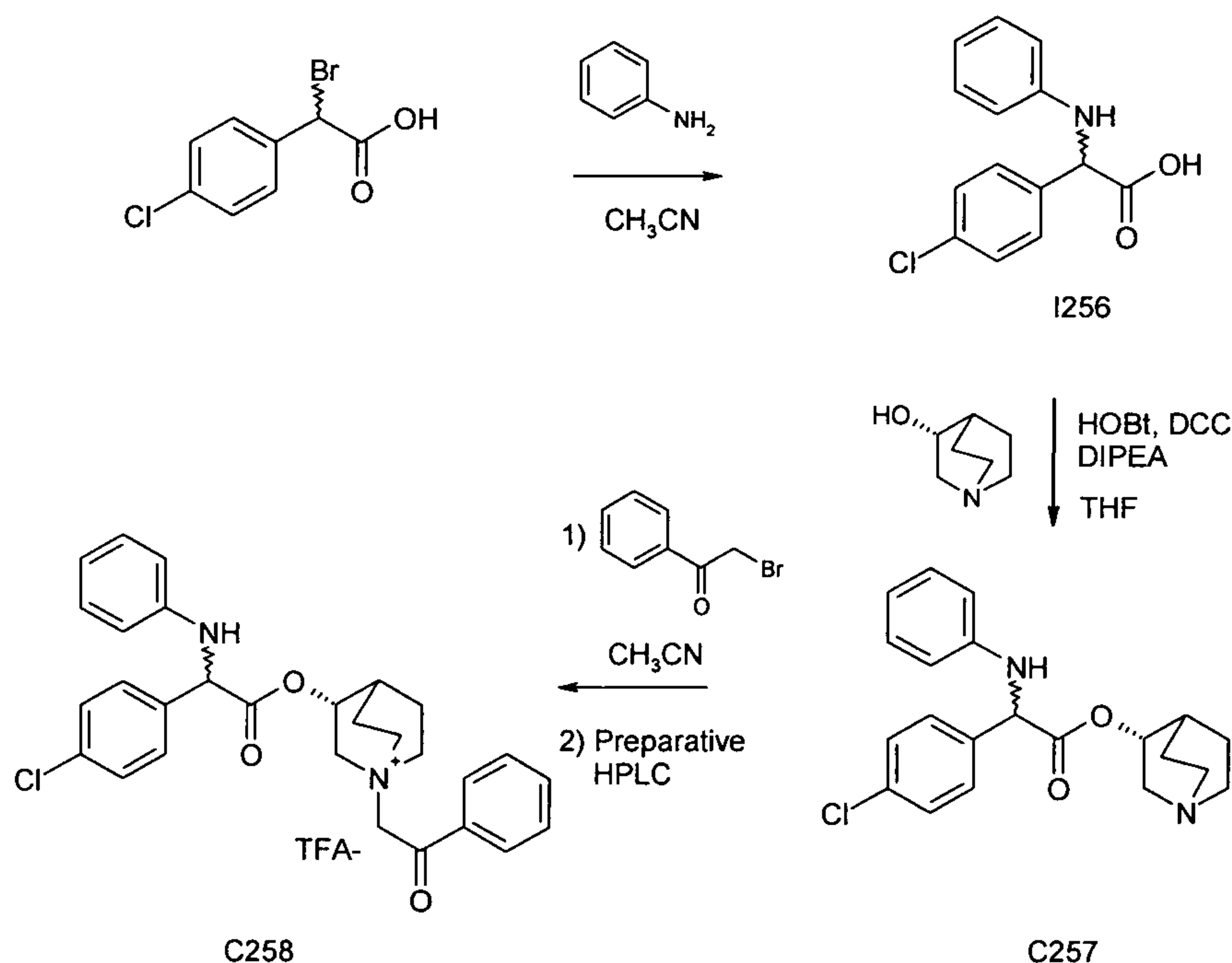
Scheme 66
