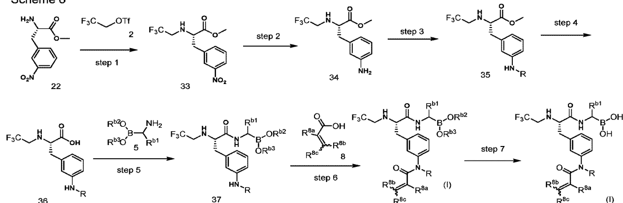
Scheme 7
