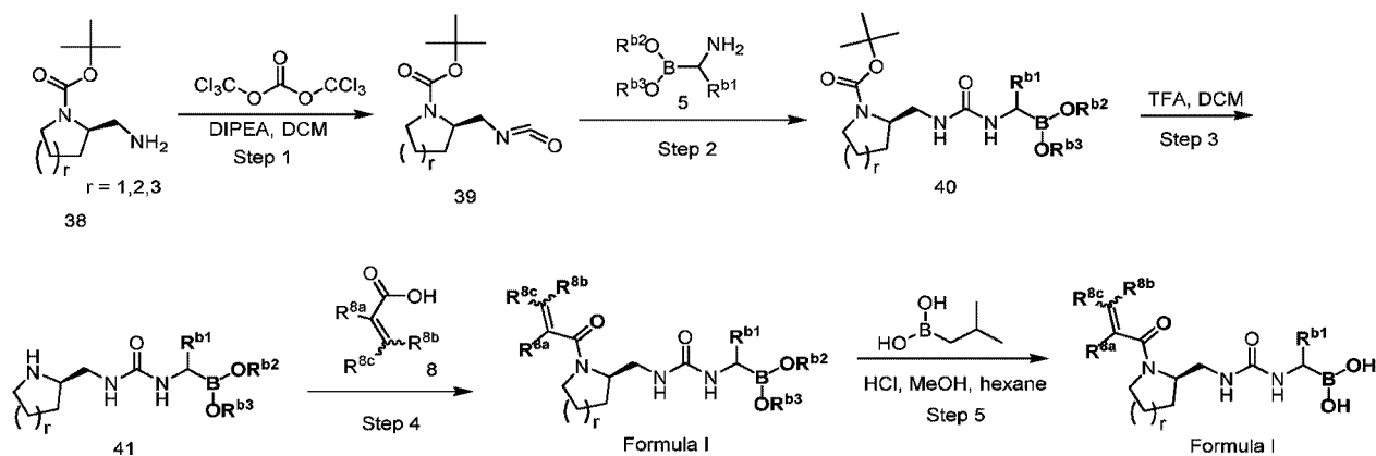
Scheme 7
