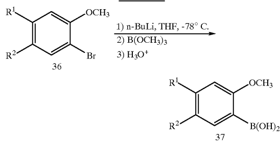
Scheme XI
