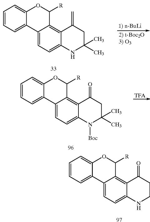
Scheme XXVII
