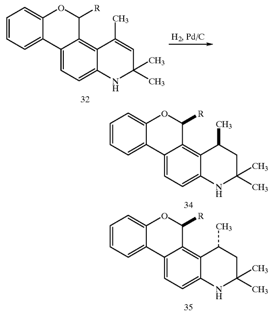
Scheme X
