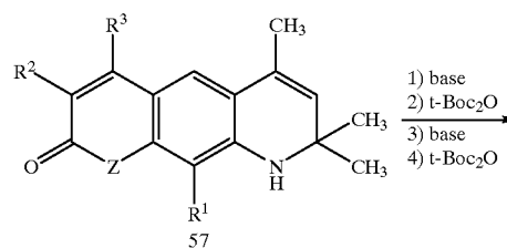
Scheme XLIV
