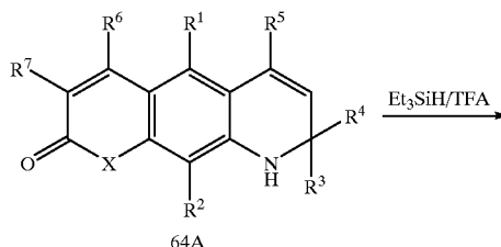
Scheme XLIX
