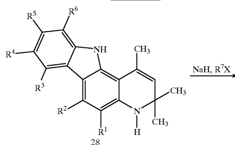
Scheme VIII
