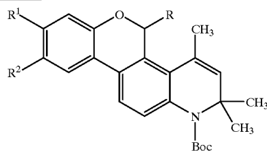
Scheme XXXIII
