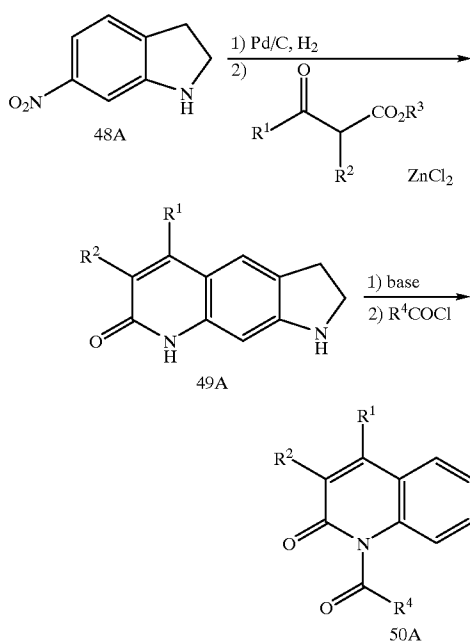
Scheme XLV
