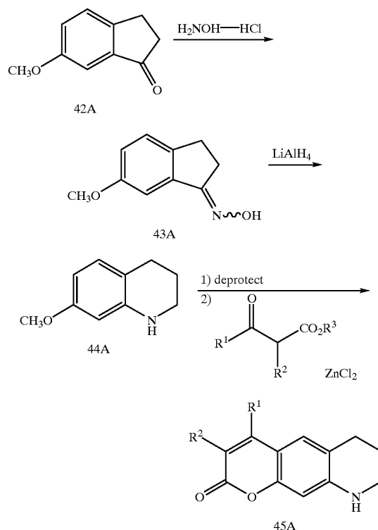
Scheme XLIII
