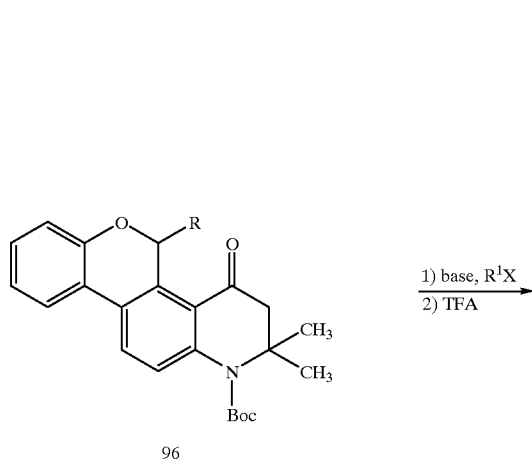
Scheme XXVIII
