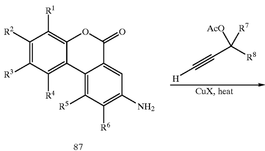
Scheme XXIII
