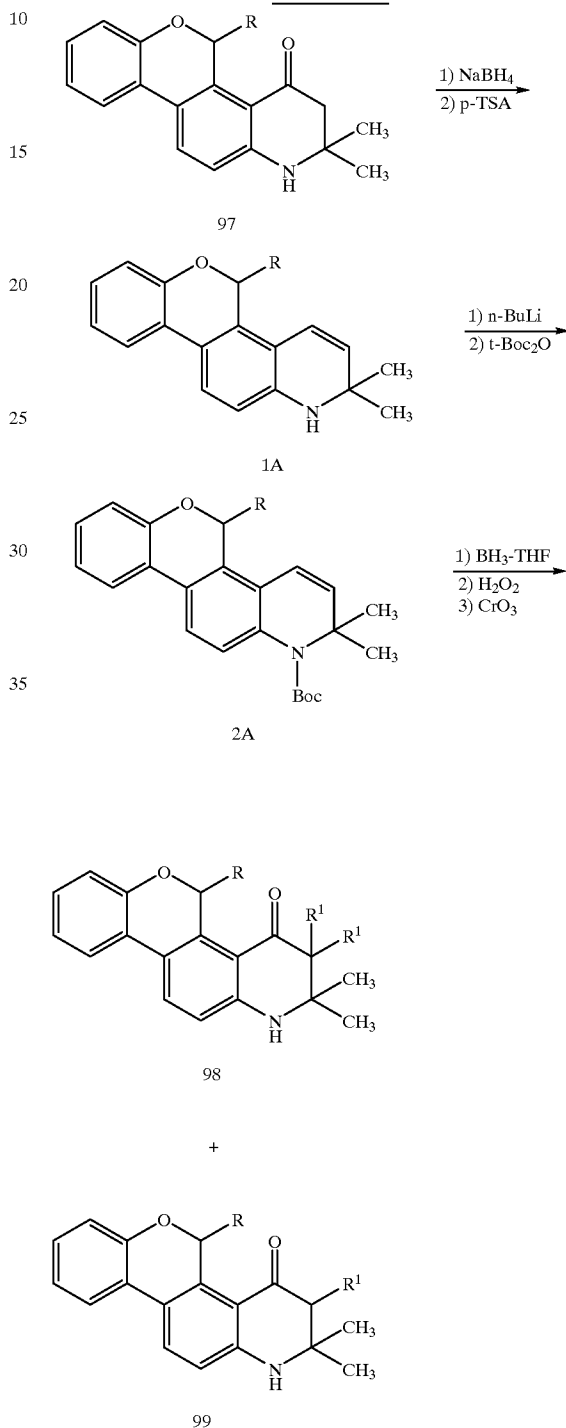
Scheme XXIX
