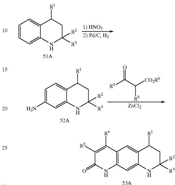
Scheme XLVI
