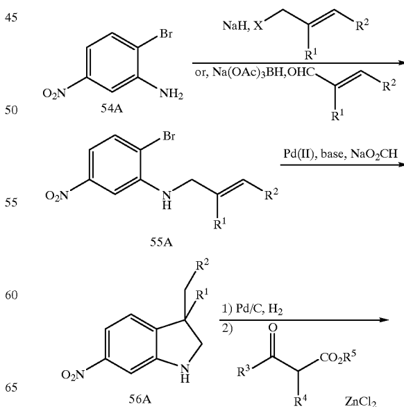
Scheme XLVII
