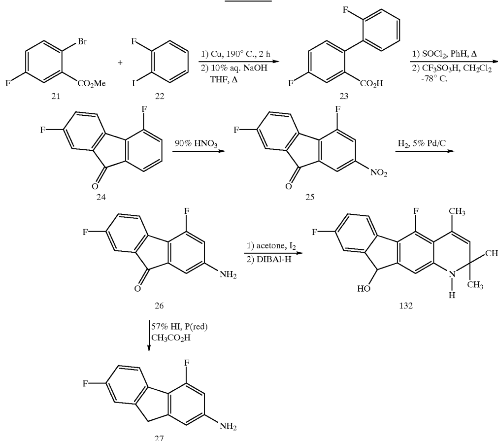
Scheme VII
