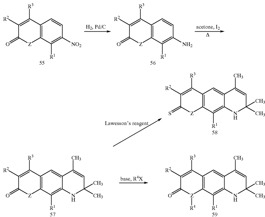
Scheme XVI
