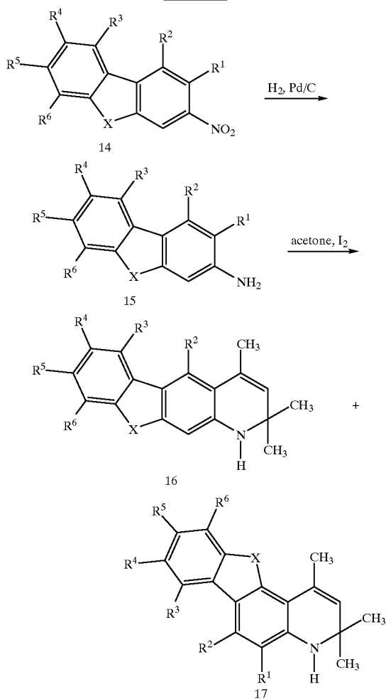
Scheme IV
