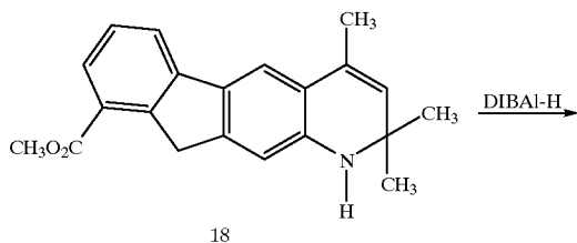
Scheme V
