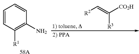
Scheme XLVIII
