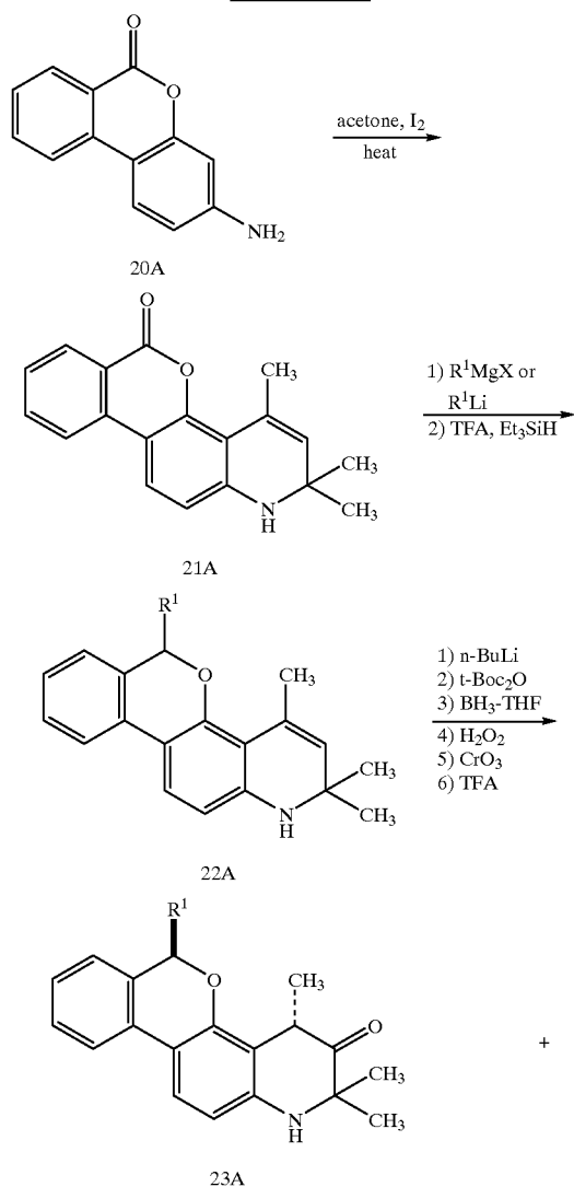
Scheme XXXV
