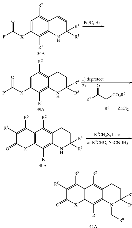
Scheme XLII
