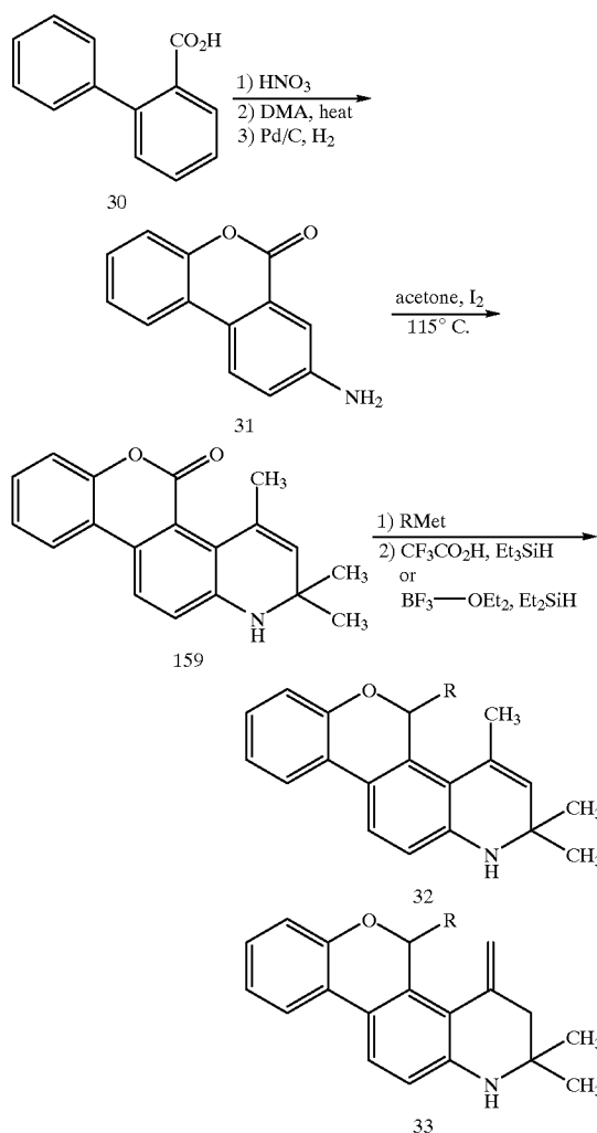
Scheme IX
