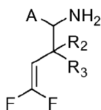
Formula (III);
