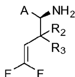
Formula (IV);
