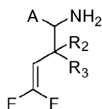
Formula (III);
