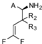
Formula (IV);
