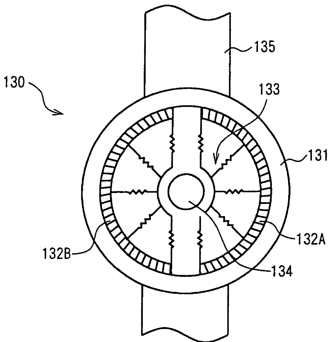
FIG. 2 (RELATED ART)
