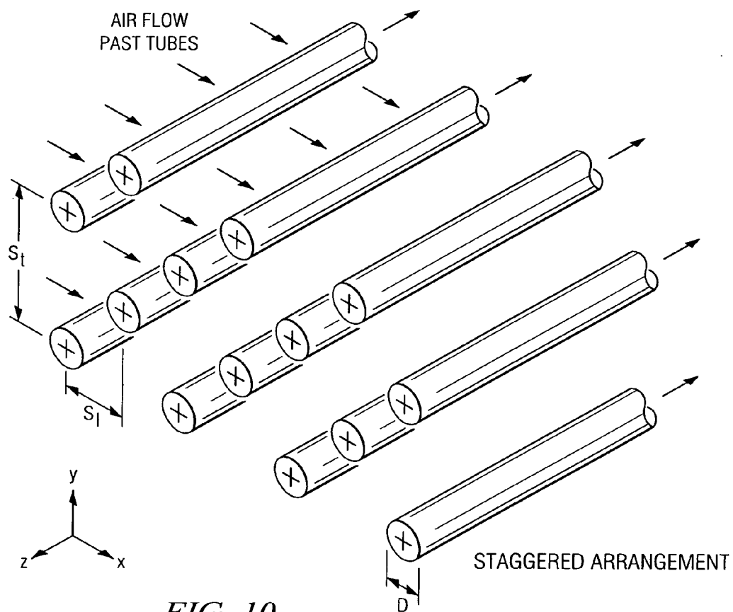
FIG. 10 METAL HYDRIDE TUBE PLACEMENT IN THE BENCH TOP MHAC
