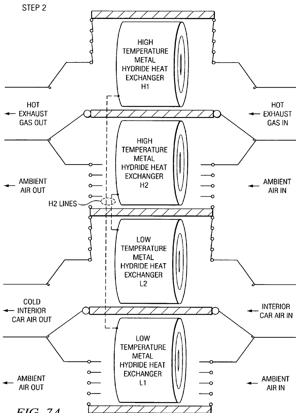
FIG. 7A OPERATIONAL SCHEMATIC FOR PROCESS STEP #2
