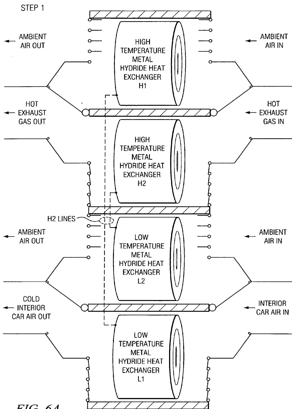
FIG. 6A OPERATIONAL SCHEMATIC FOR PROCESS STEP #1
