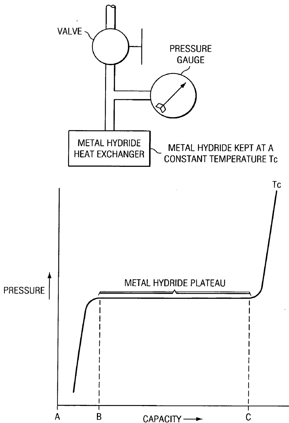
FIG. 3 PCT TEST APPARATUS AND PLOT
