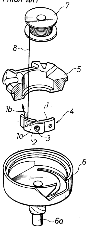
FIG. 1 PRIOR ART
