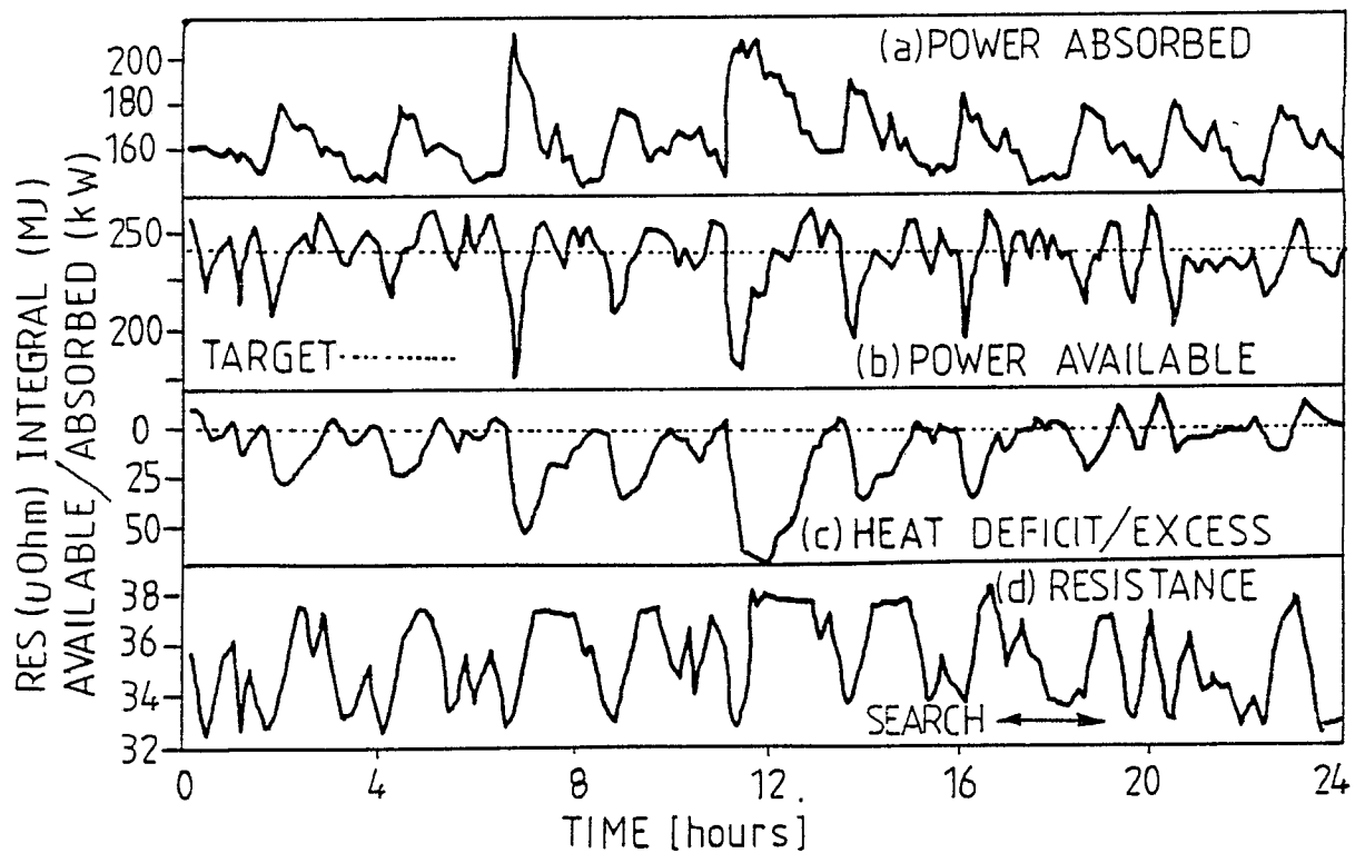
Fig. 8. Control System and Cell Response over 24 hours
