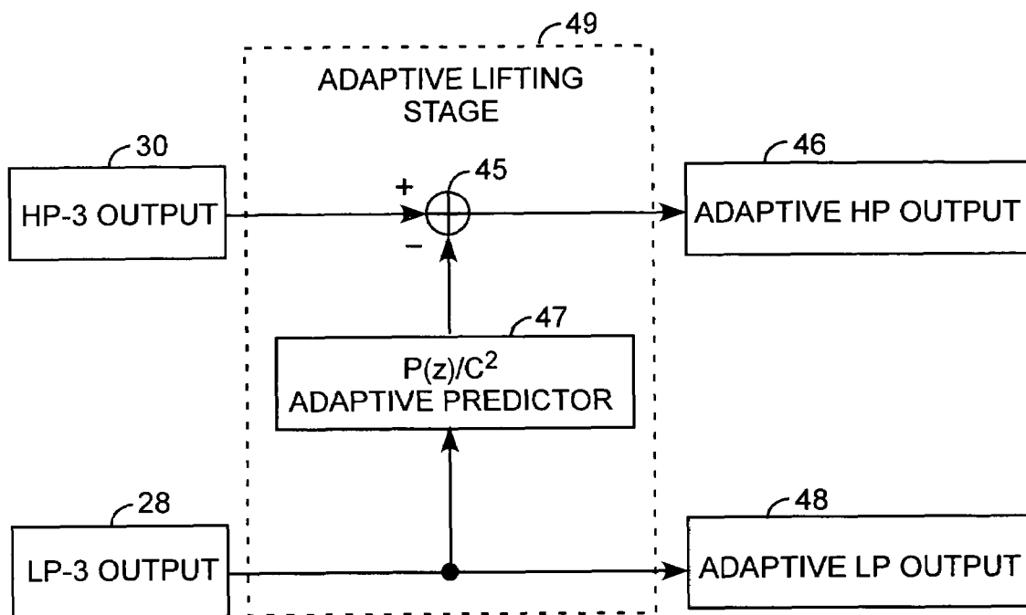
ADAPTIVE LIFTING STAGE WAVELET TRANSFORM
