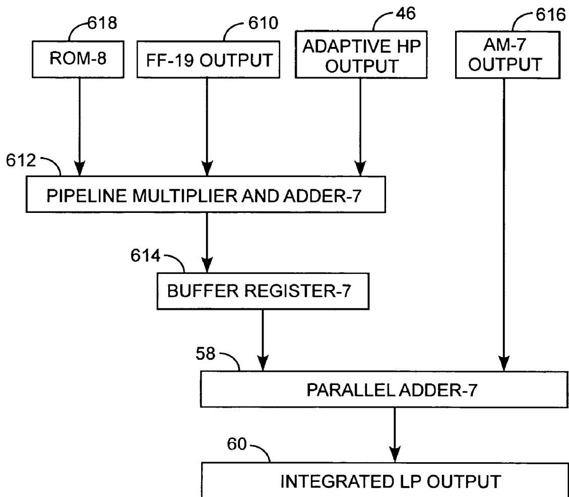
INTEGRATED LIFTING PIPELINE
