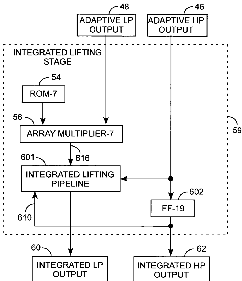
INTEGRATED LIFTING STAGE WAVELET TRANSFORM IMPLEMENTATION
