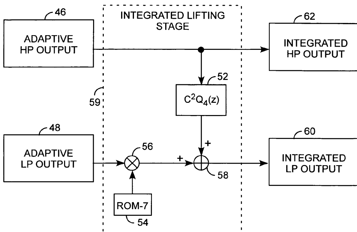
INTEGRATED LIFTING STAGE WAVELET TRANSFORM
