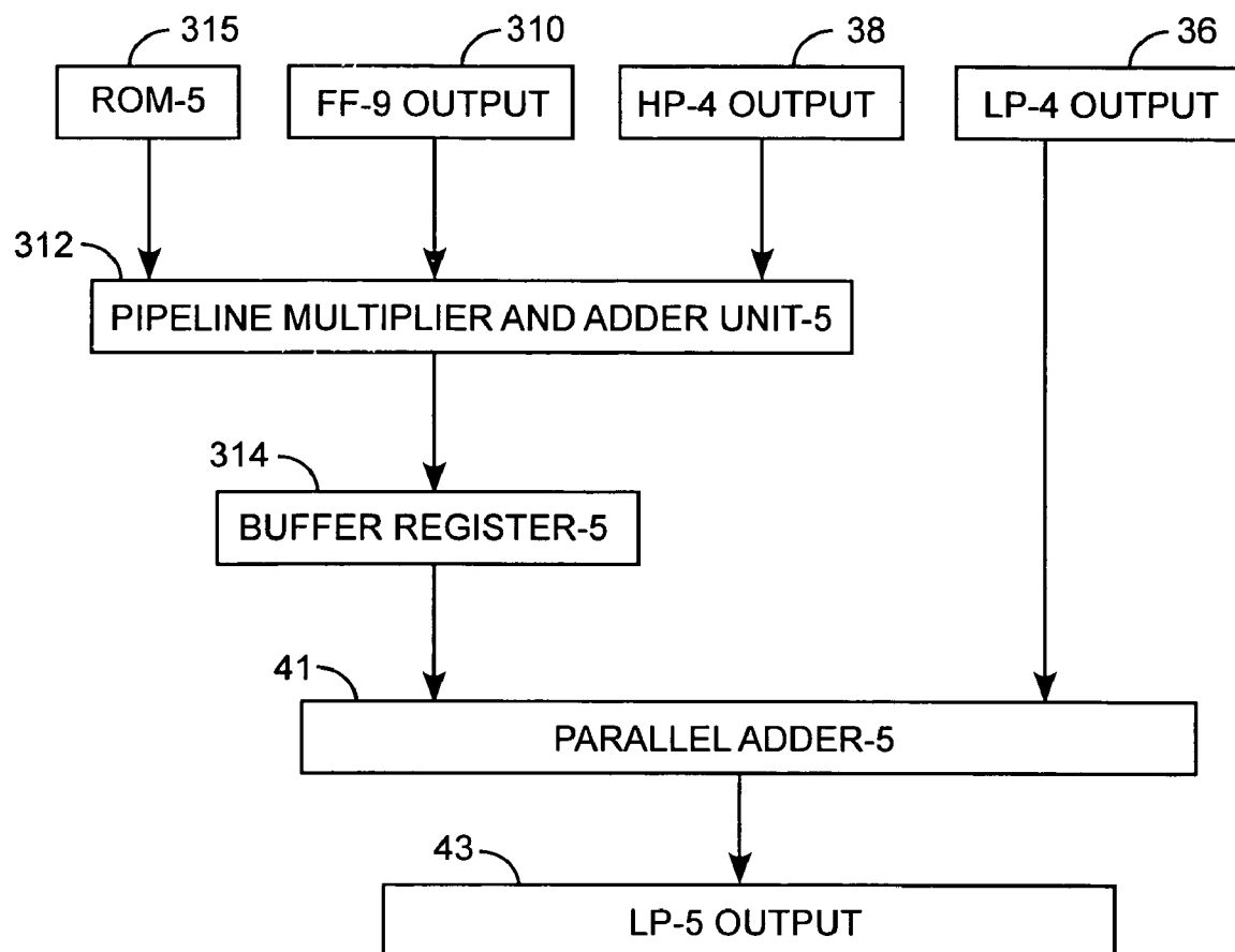
FIFTH LIFTING PIPELINE
