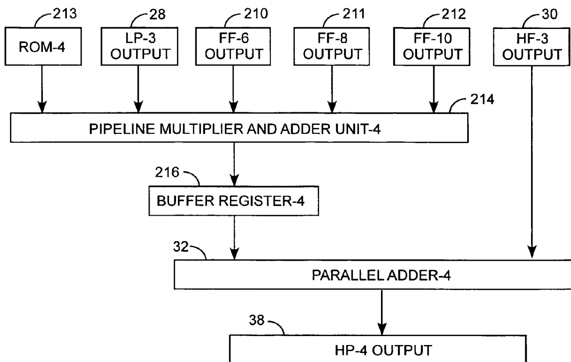
FOURTH LIFTING PIPELINE
