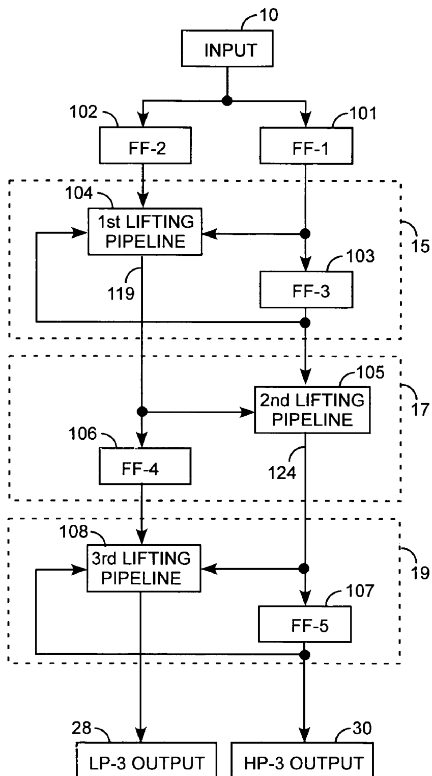
THREE LIFTING STAGE WAVELET TRANSFORM IMPLEMENTATION
