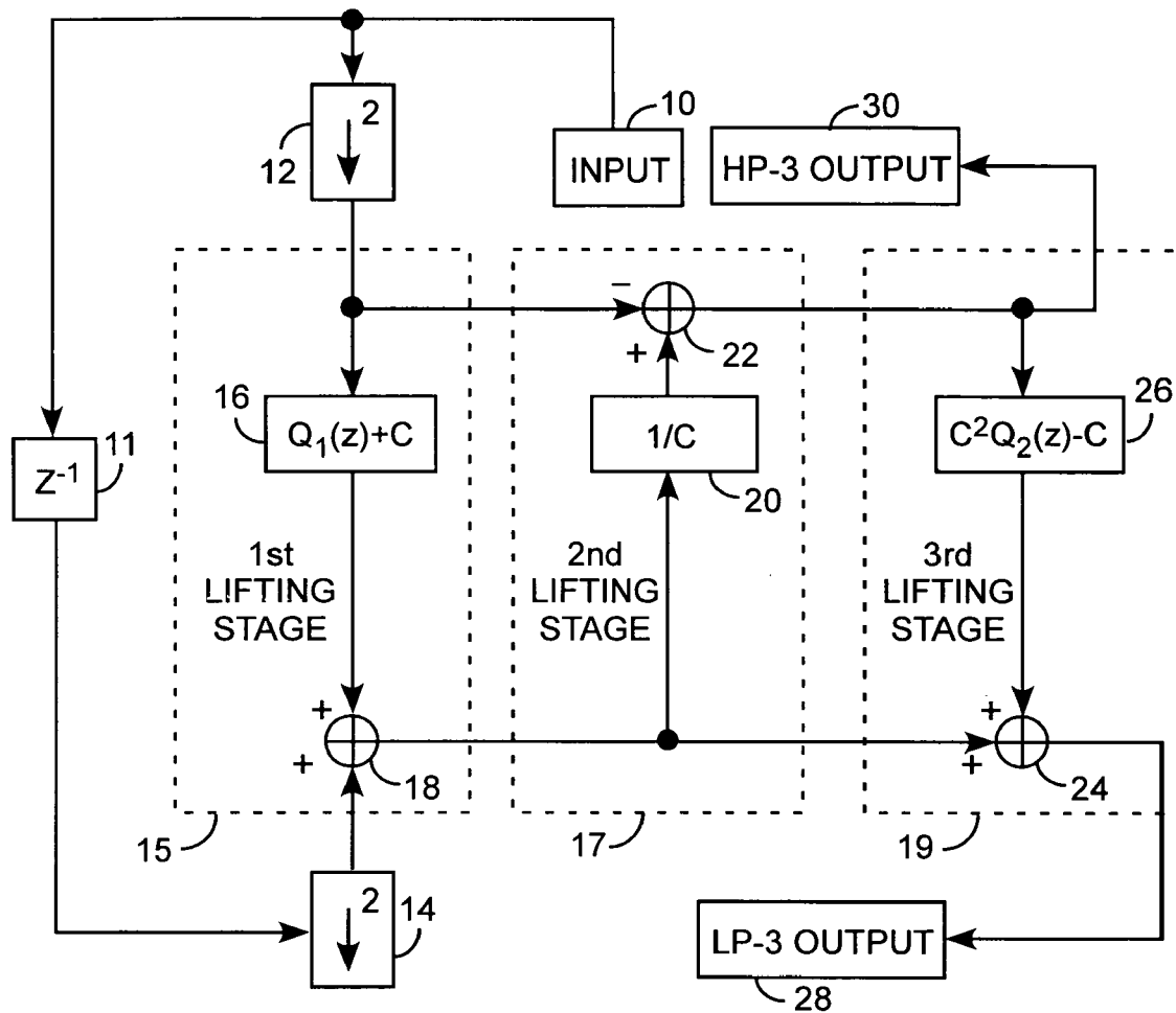
THREE LIFTING STAGE WAVELET TRANSFORM
