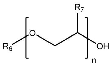
(Formula Va)
