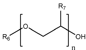
(Formula Va)
