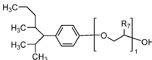
(Formula Vc)
