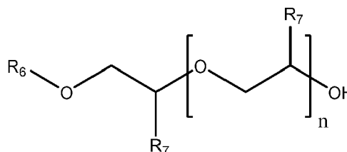
(Formula Vb)
