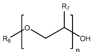
(Formula Va)
