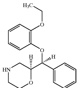
(S, S) 2-[(2-ethoxyphenoxy)(phenyl)methyl]morpholine
