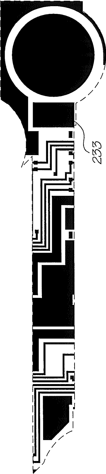
Metal 2 mask
