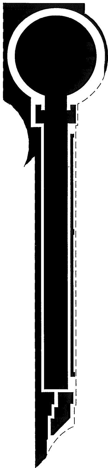
Metal 3 mask
