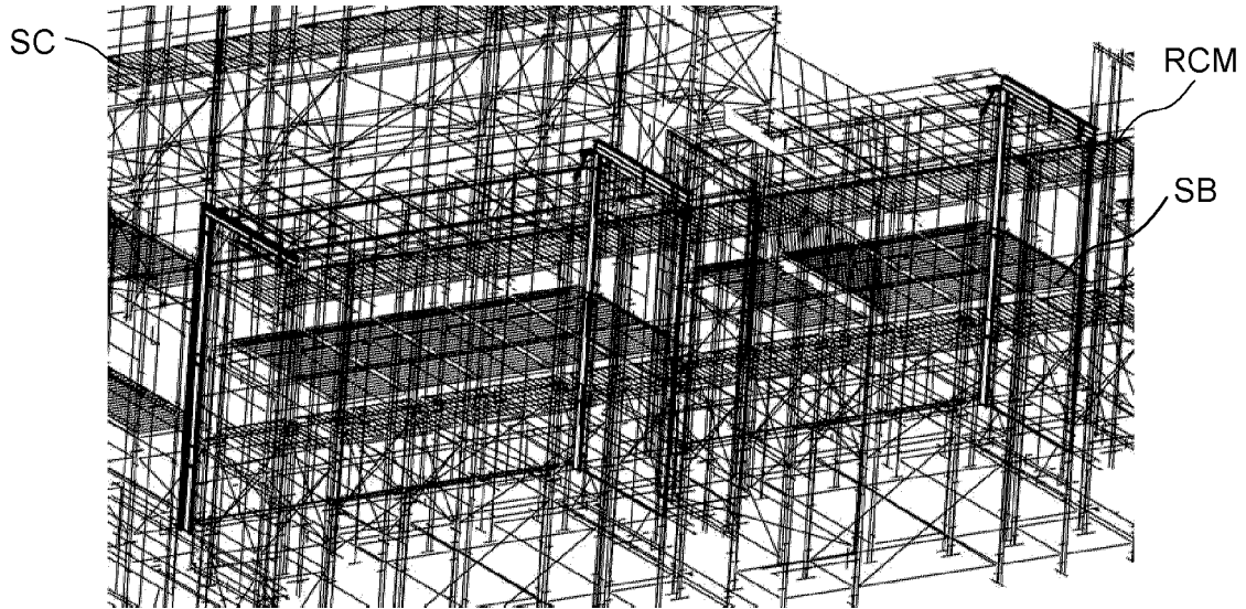
OPEN POSITION – ISOMETRIC VIEW
