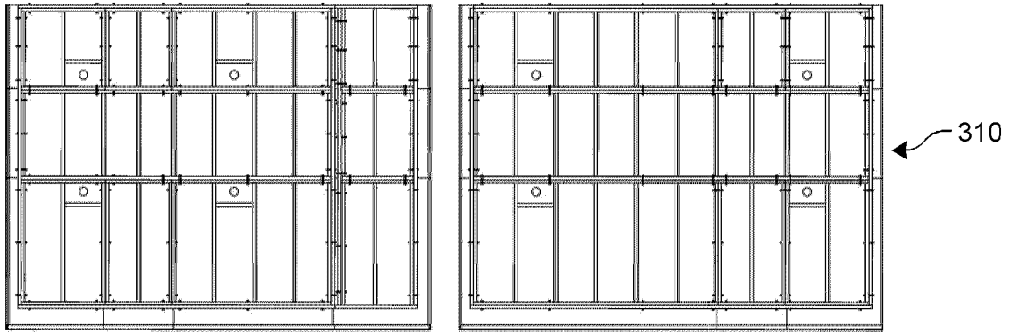
LOGITUDINAL INTERIOR – FRONT VIEW
