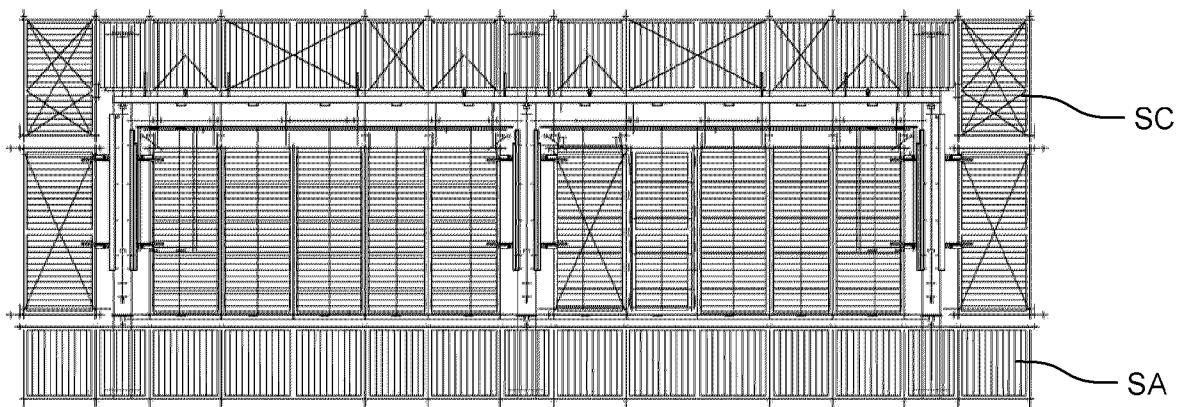
OPEN POSITION SHOWN WITH ACTUATORS – TOP VIEW
