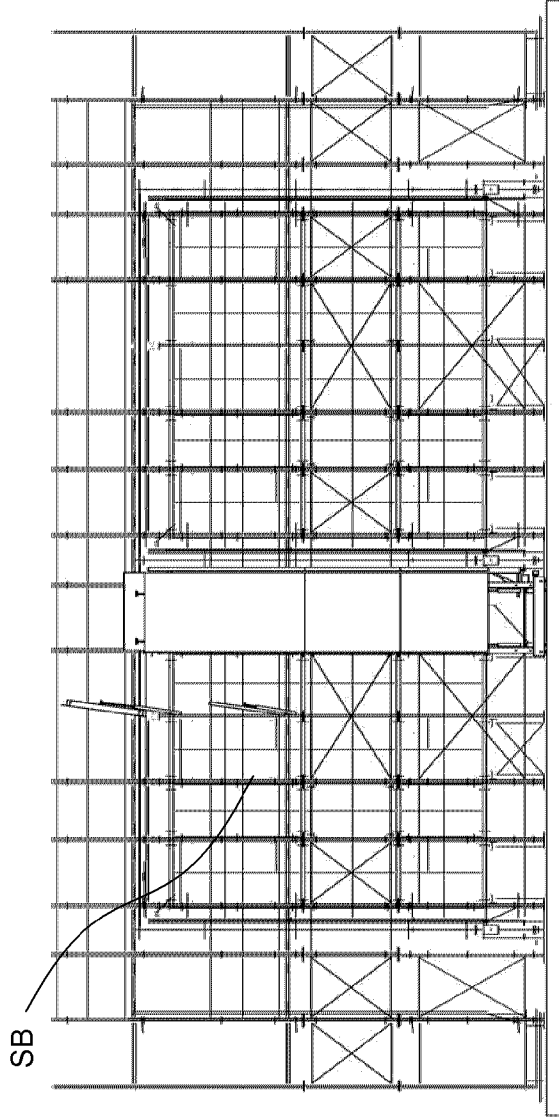
CLOSED POSITION - REAR VIEW
