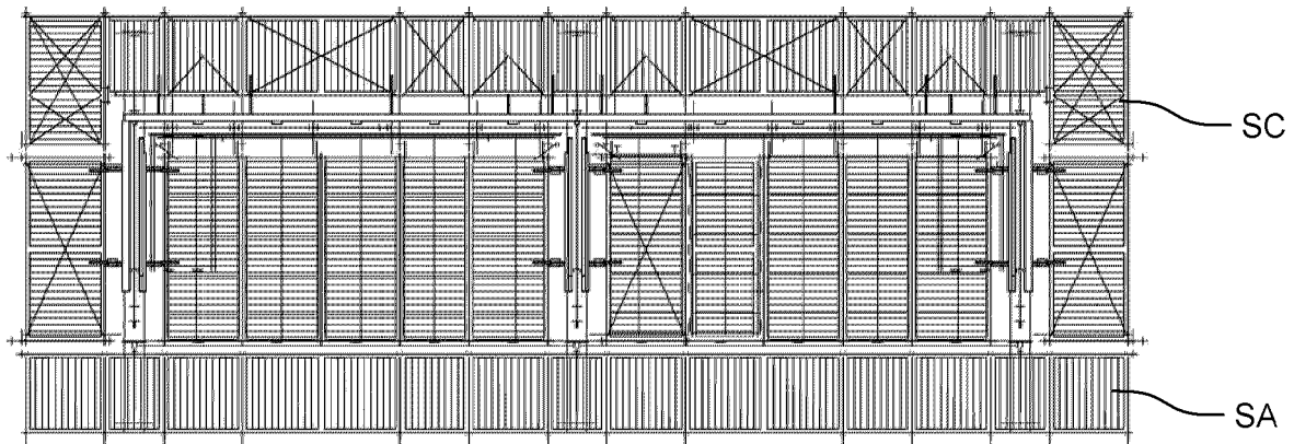
CLOSED POSITION SHOWN WITH ACTUATORS – TOP VIEW
