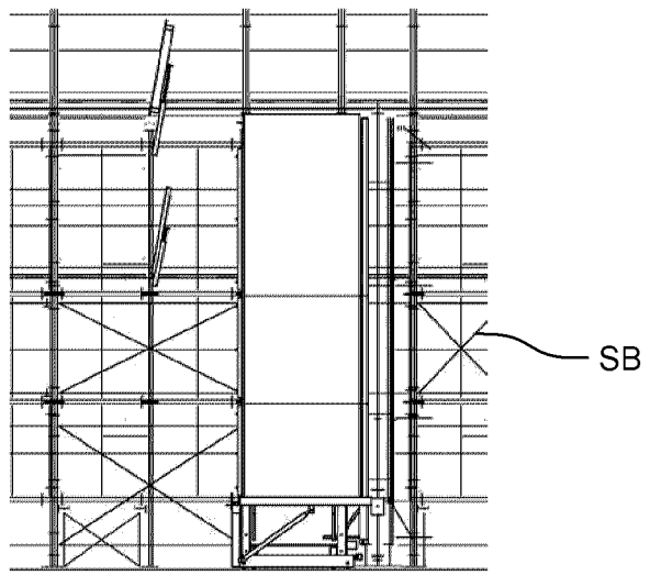
RAISED - REAR VIEW
