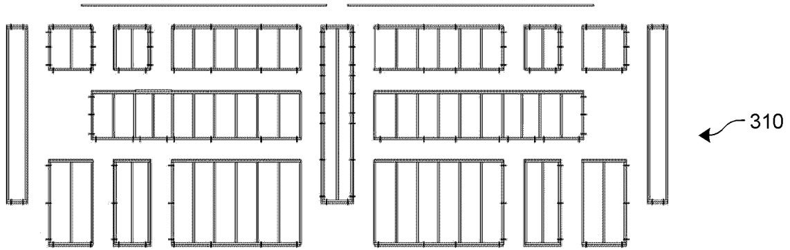
PREFABRICATED FORM COMPONENTS – REAR VIEW FIGURE 62 (CONT'D) – FORM SYSTEM LONGITUDINAL WALLS
