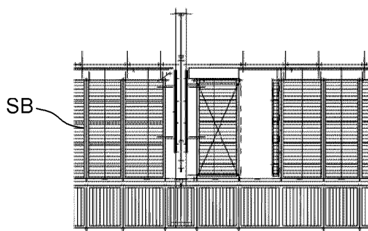
CLOSED - TOP VIEW
