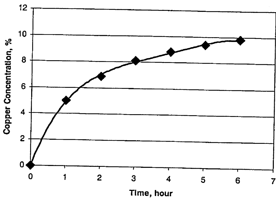
Figur 8. Copper Dissolution at 2% Initial Carbonation L v Is
