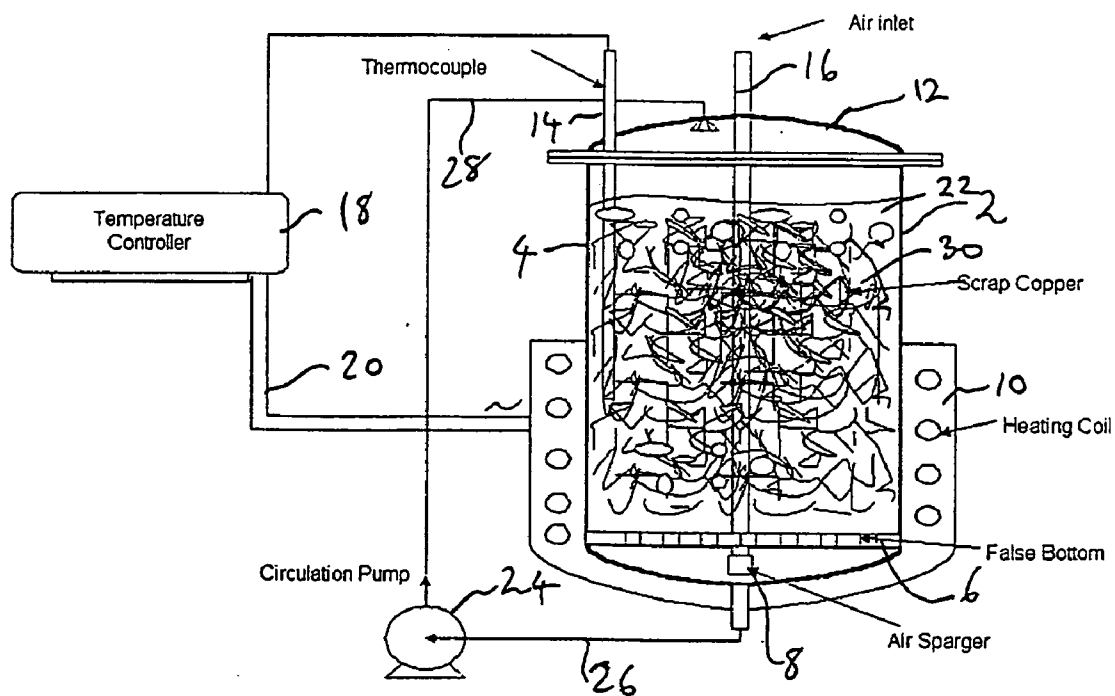
A Batch Dissolver
