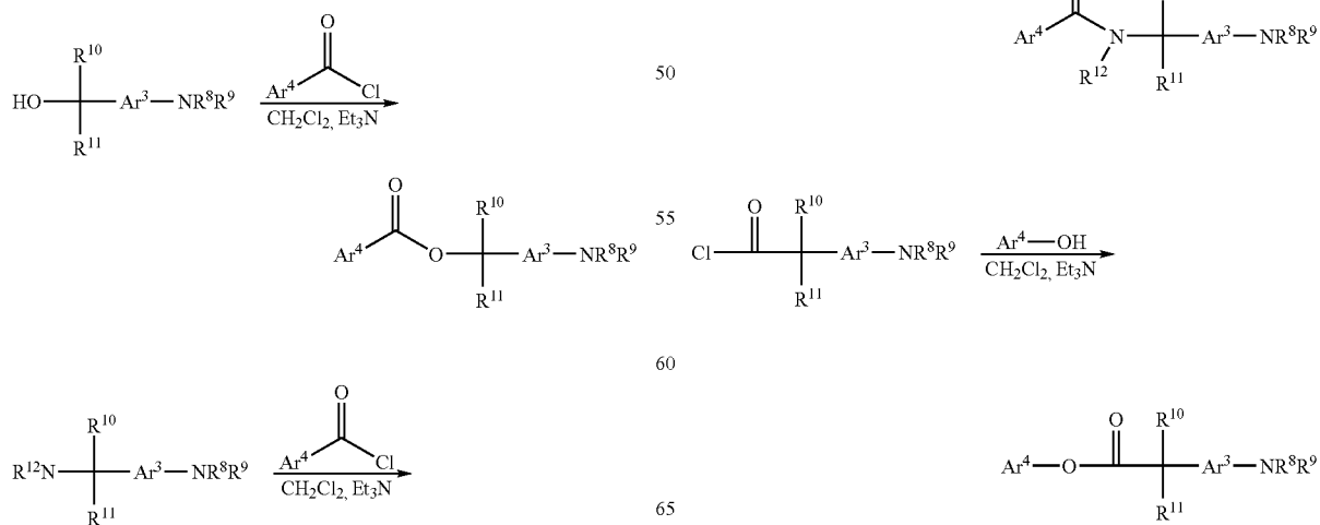
Reaction Scheme 2
