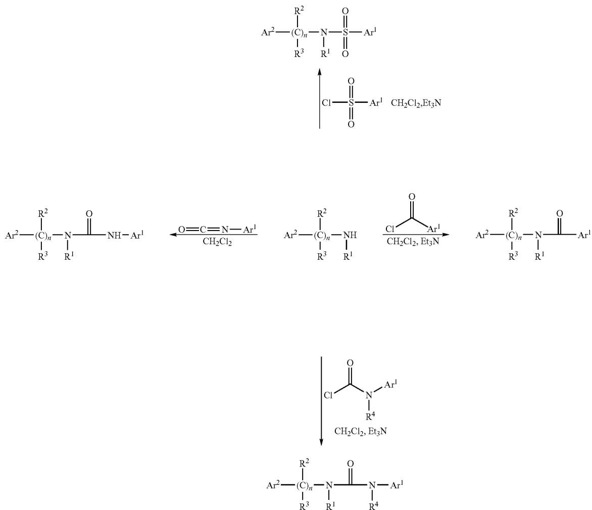
Reaction scheme 1
