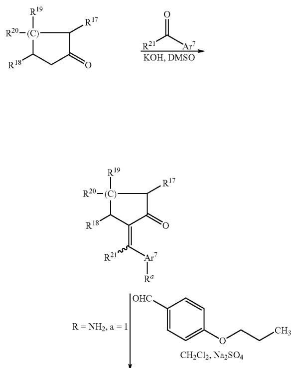
Reaction Scheme 4
