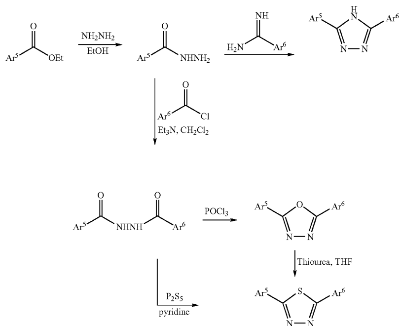
Reaction Scheme 3
