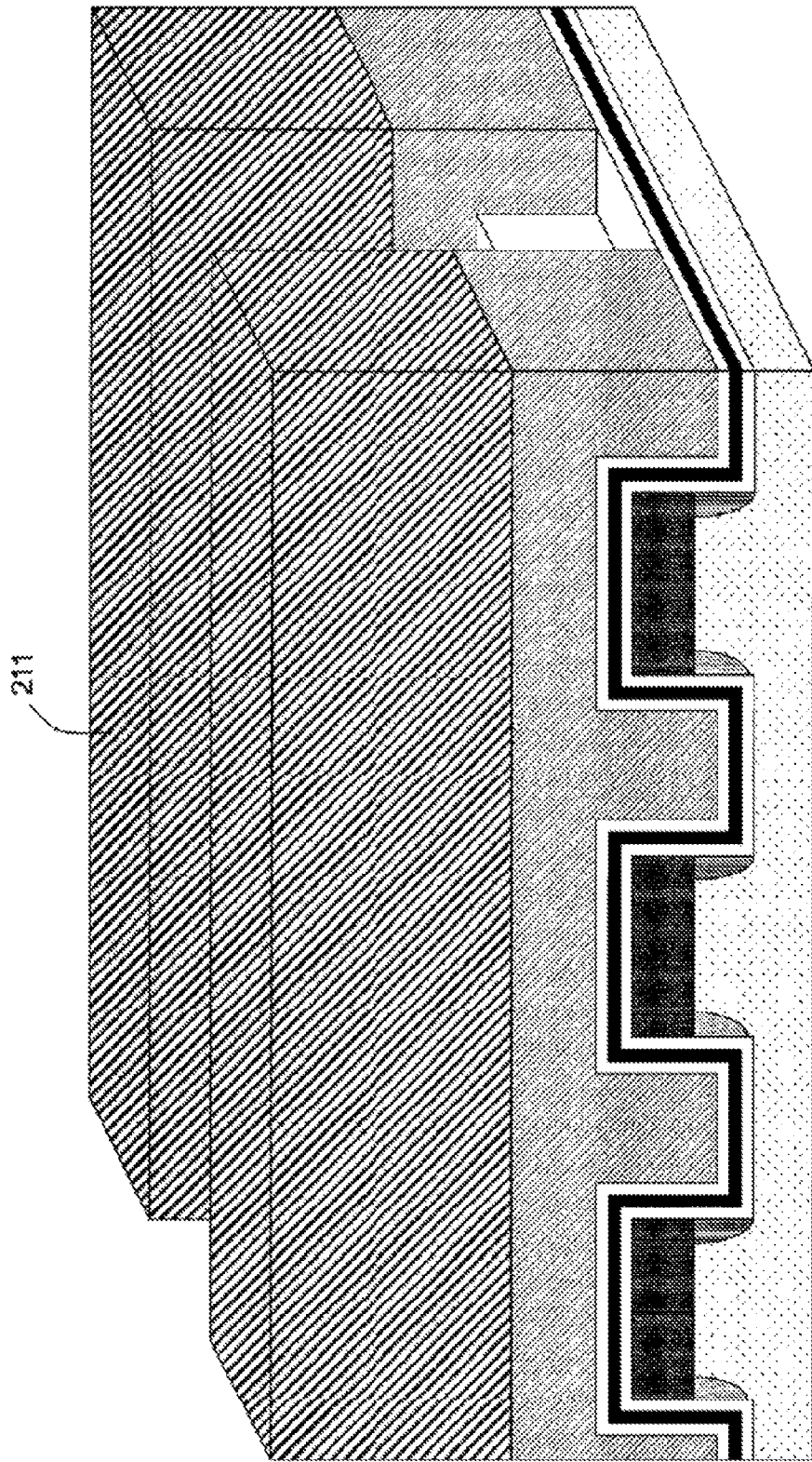
Fig.24 Process 9 : gate electrode polysilicon patterning
