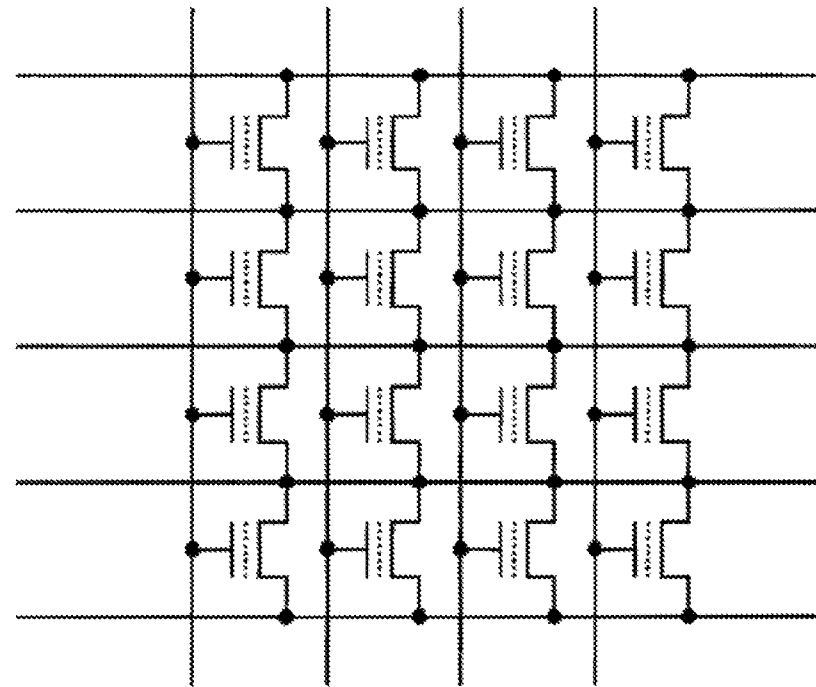
(B): Virtual Ground Array Structure
