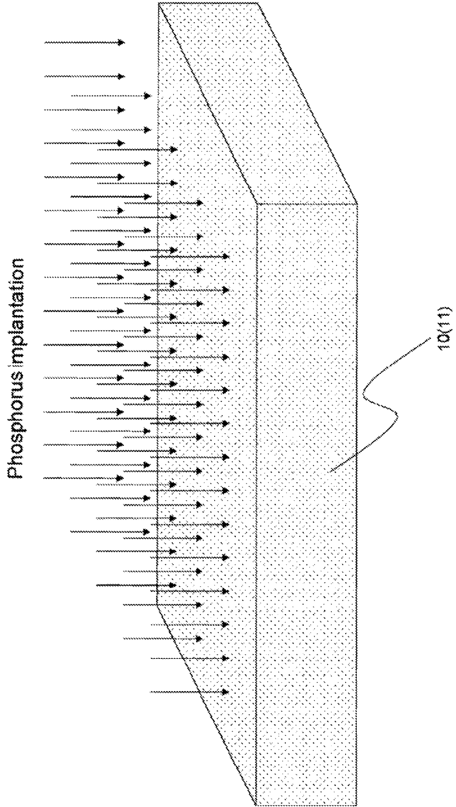
Fig. 8 Process 1 : n-Well formation (Phosphorus implantation)
