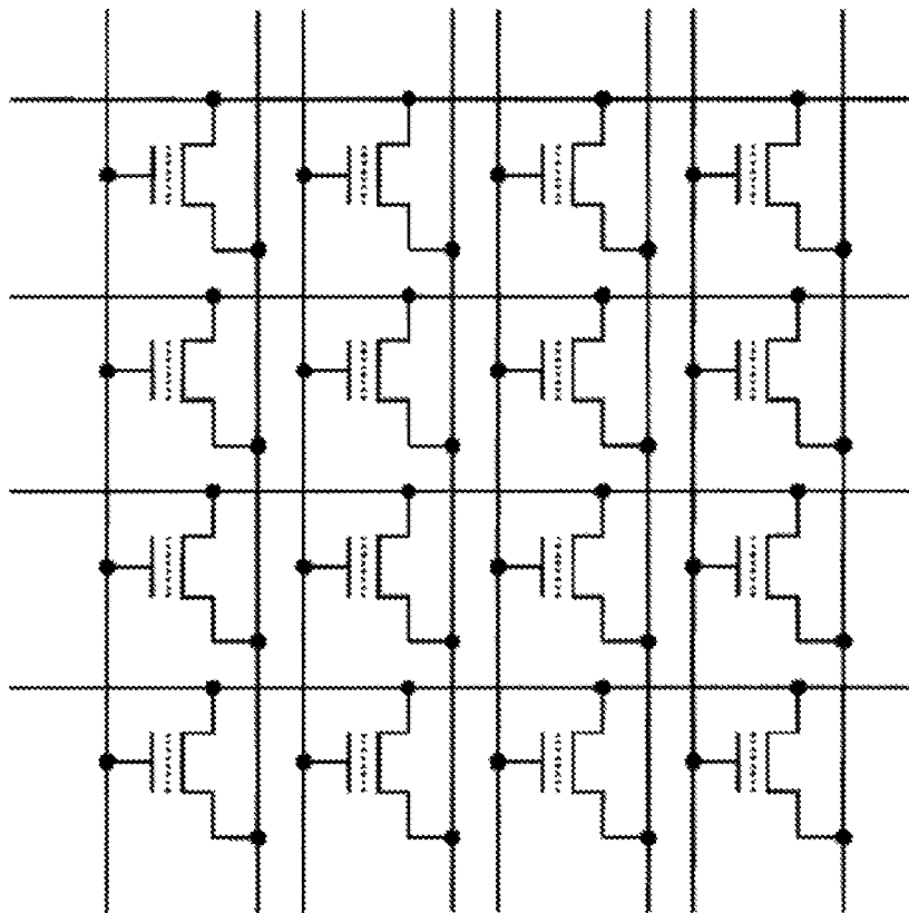
(A): NOR Array Structure
