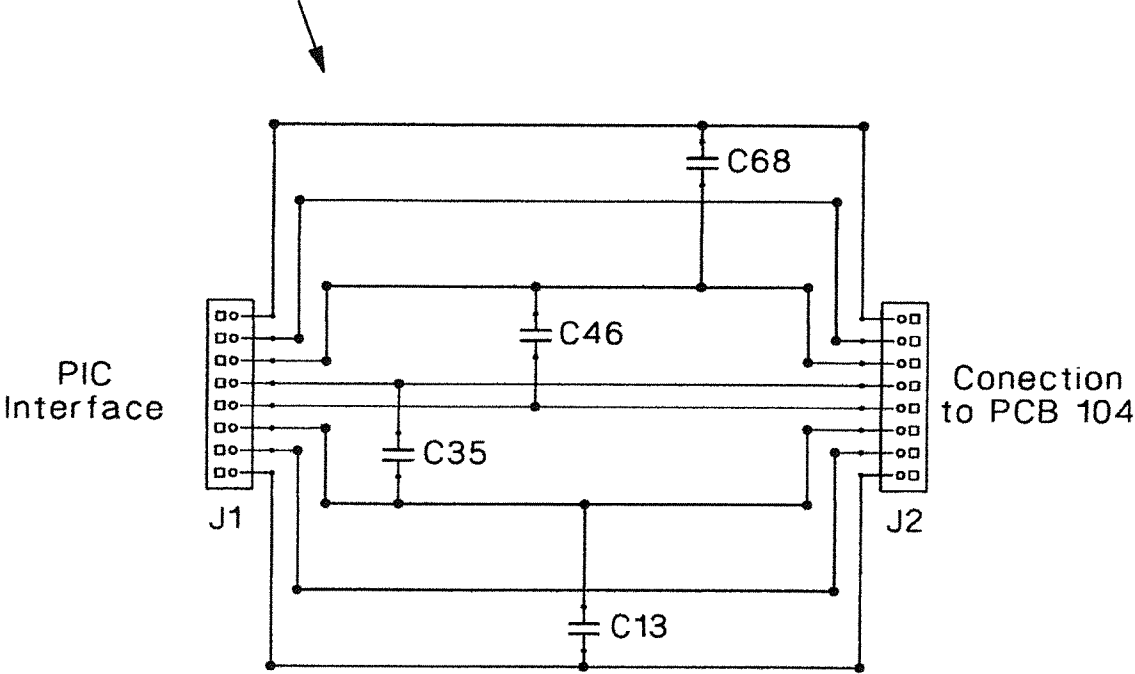
PCB 60 Schematic
