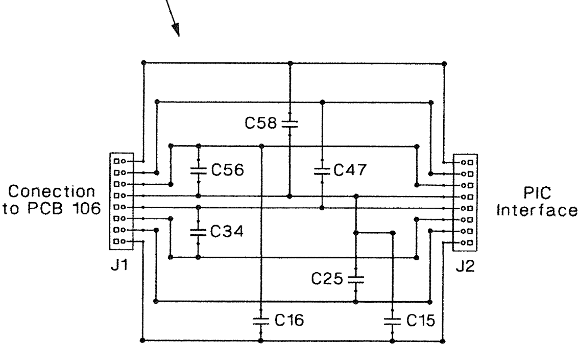
PCB 50 Schematic
