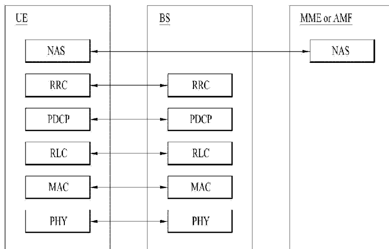
(b) Control Plane Protocol Stack
