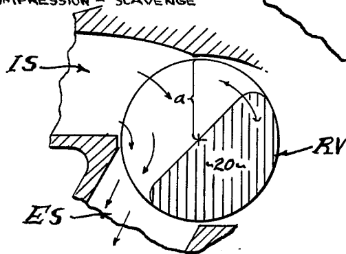
FIG. 4. COMPRESSION - SCAVENGE
