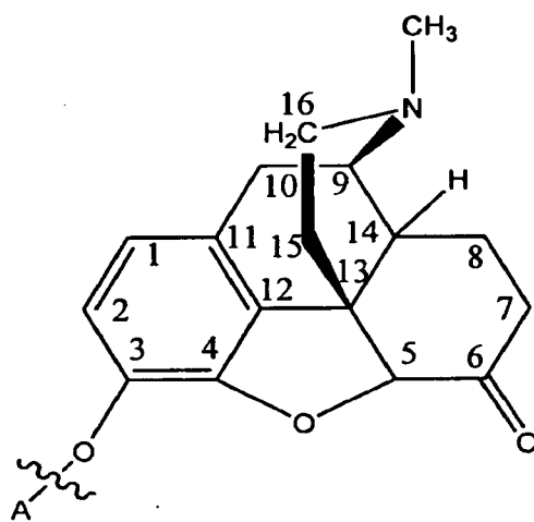
Figure 4. Structure of Hydromorphone with Attachment at the 3 Position
