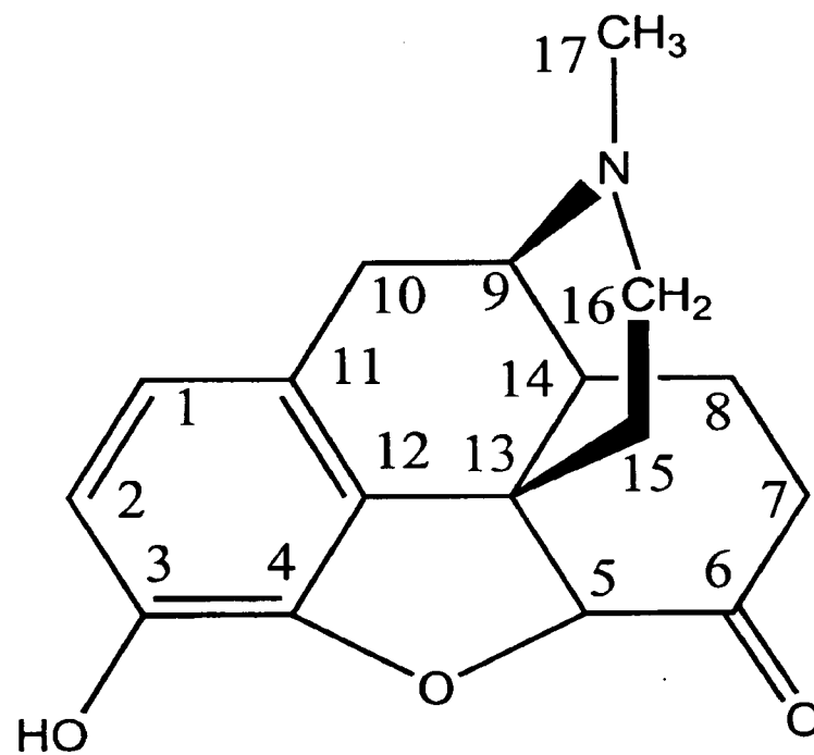
Figure 3. Structure of Hydromorphone
