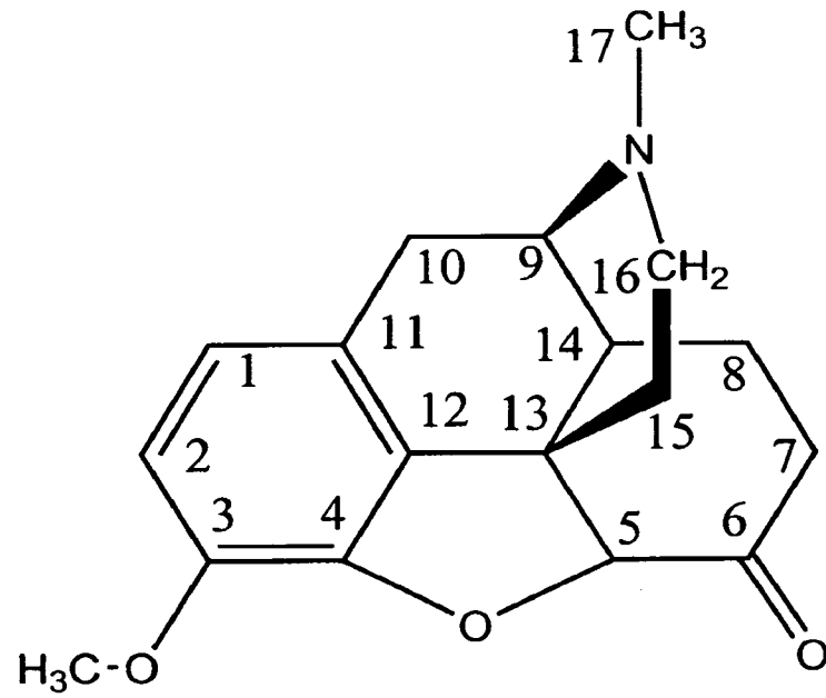
Figure 1. Structure of Hydrocodone
