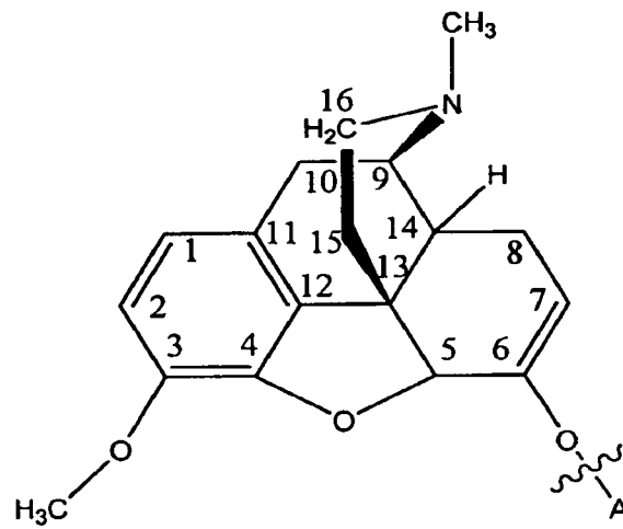
Figure 2. Structure of Hydrocodone with Attachment at the 6 Position
