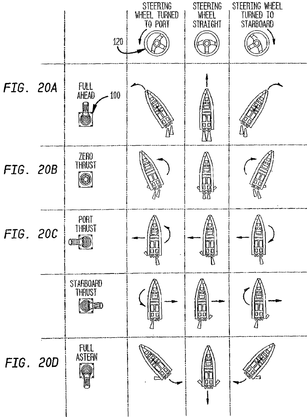
DUAL WATERJET MOTION DIAGRAM
