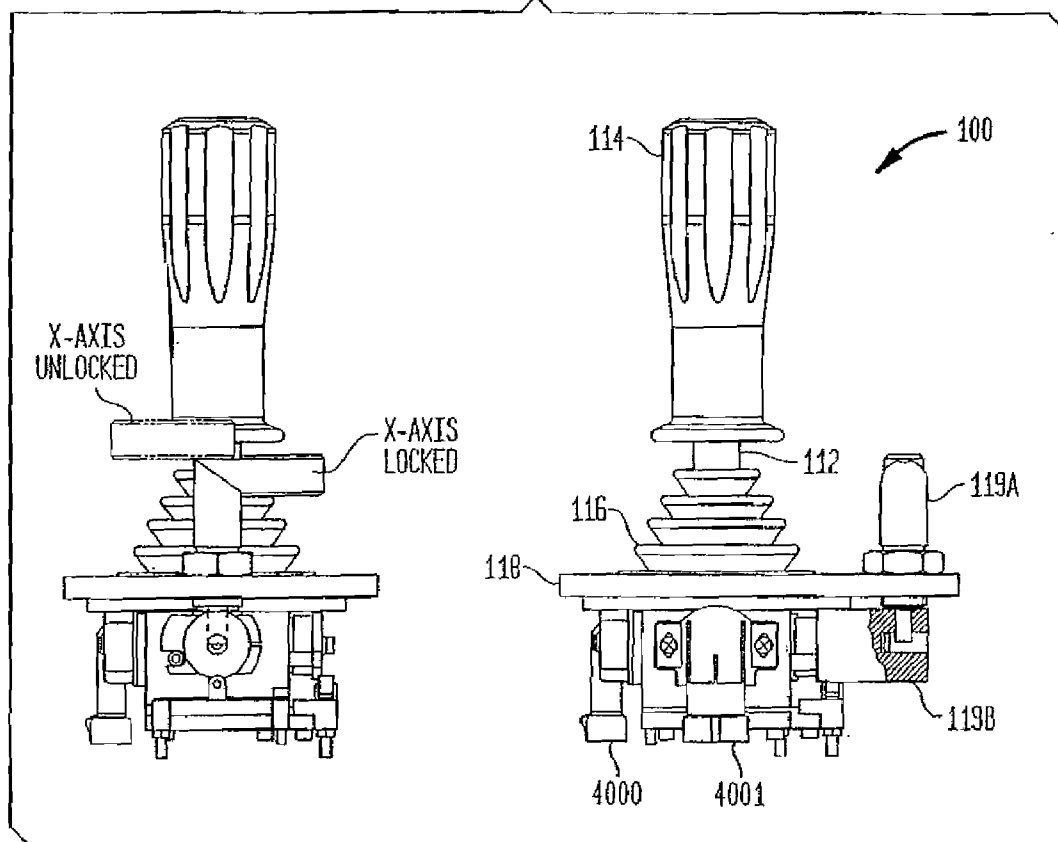
FIG. 27 LOCKING JOYSTICK WITH CAM PLUNGER
