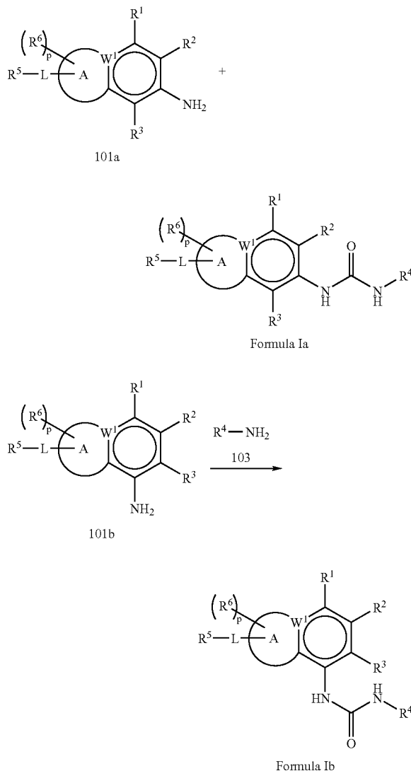
REACTION SCHEME 1
