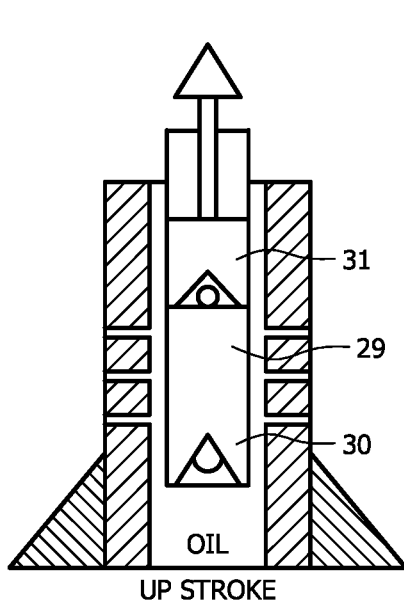
UP STROKE FIG. 3A (Prior Art)
