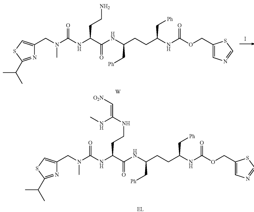
Scheme 112
