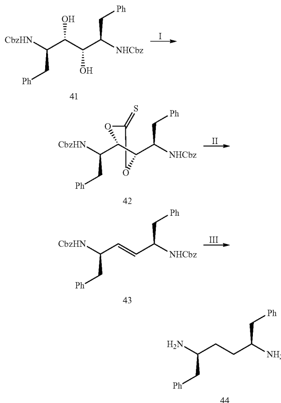
Scheme 16
