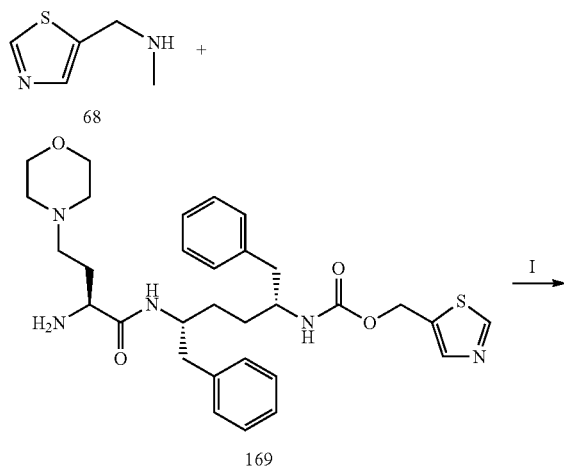
Scheme 114
