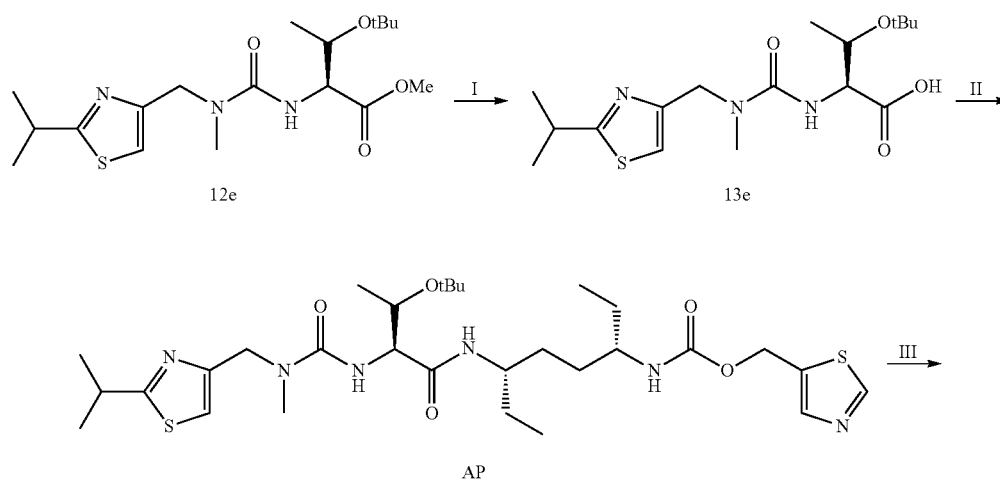
Scheme 34
