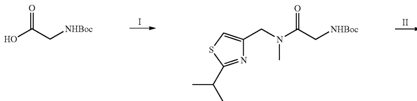
Scheme 108
