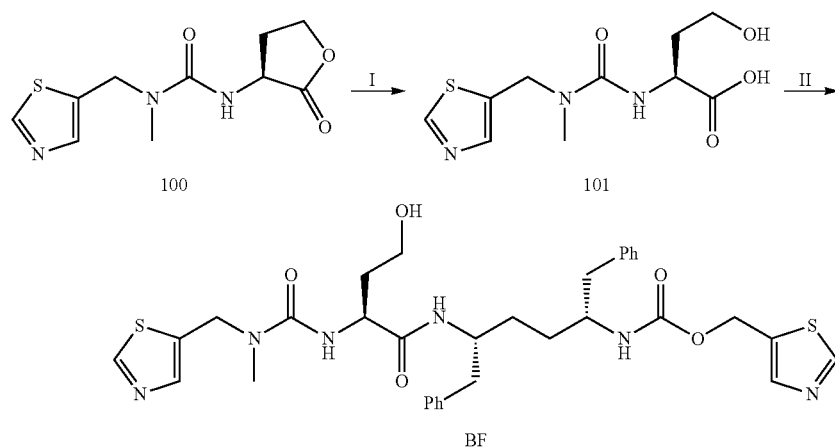
Scheme 46
