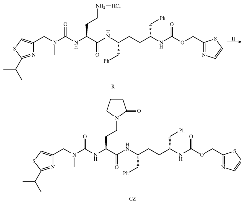
Scheme 81
