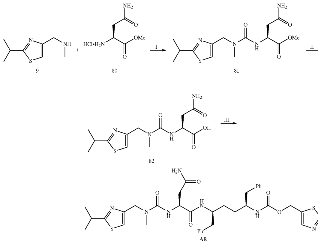
Scheme 35
