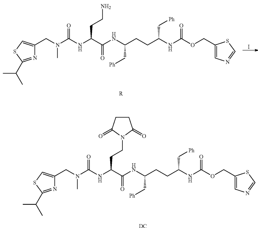
Scheme 84
