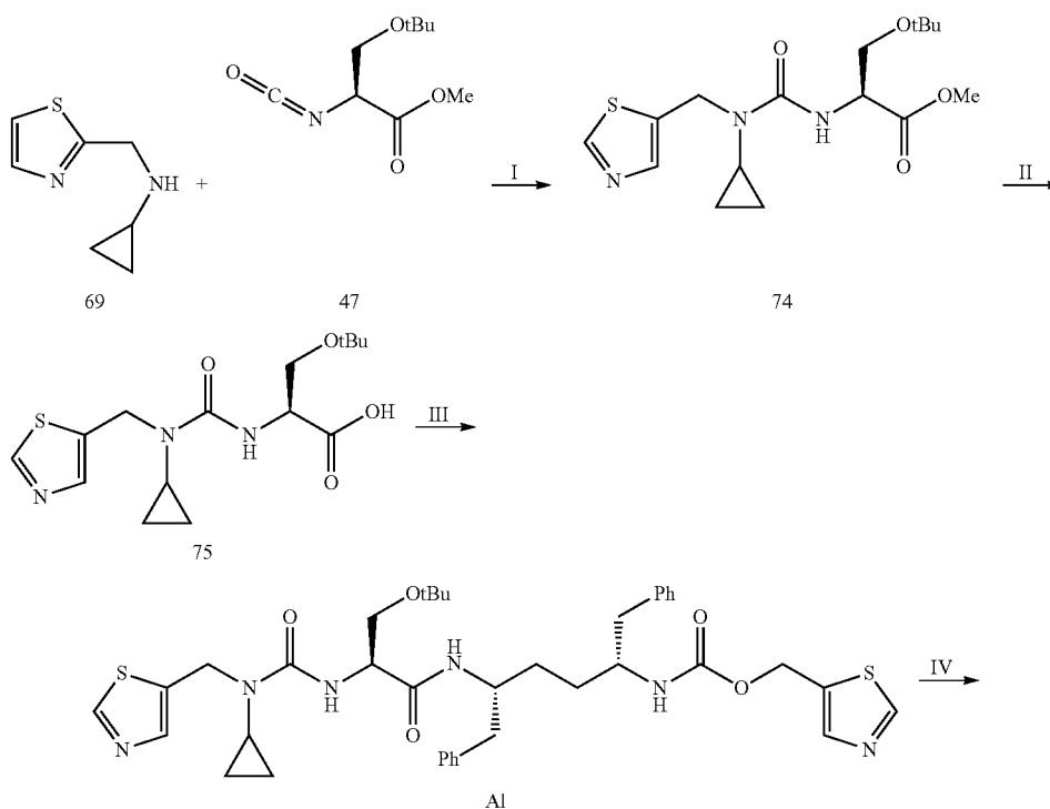
Scheme 31
