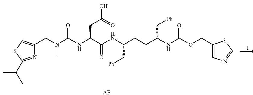
Scheme 95
