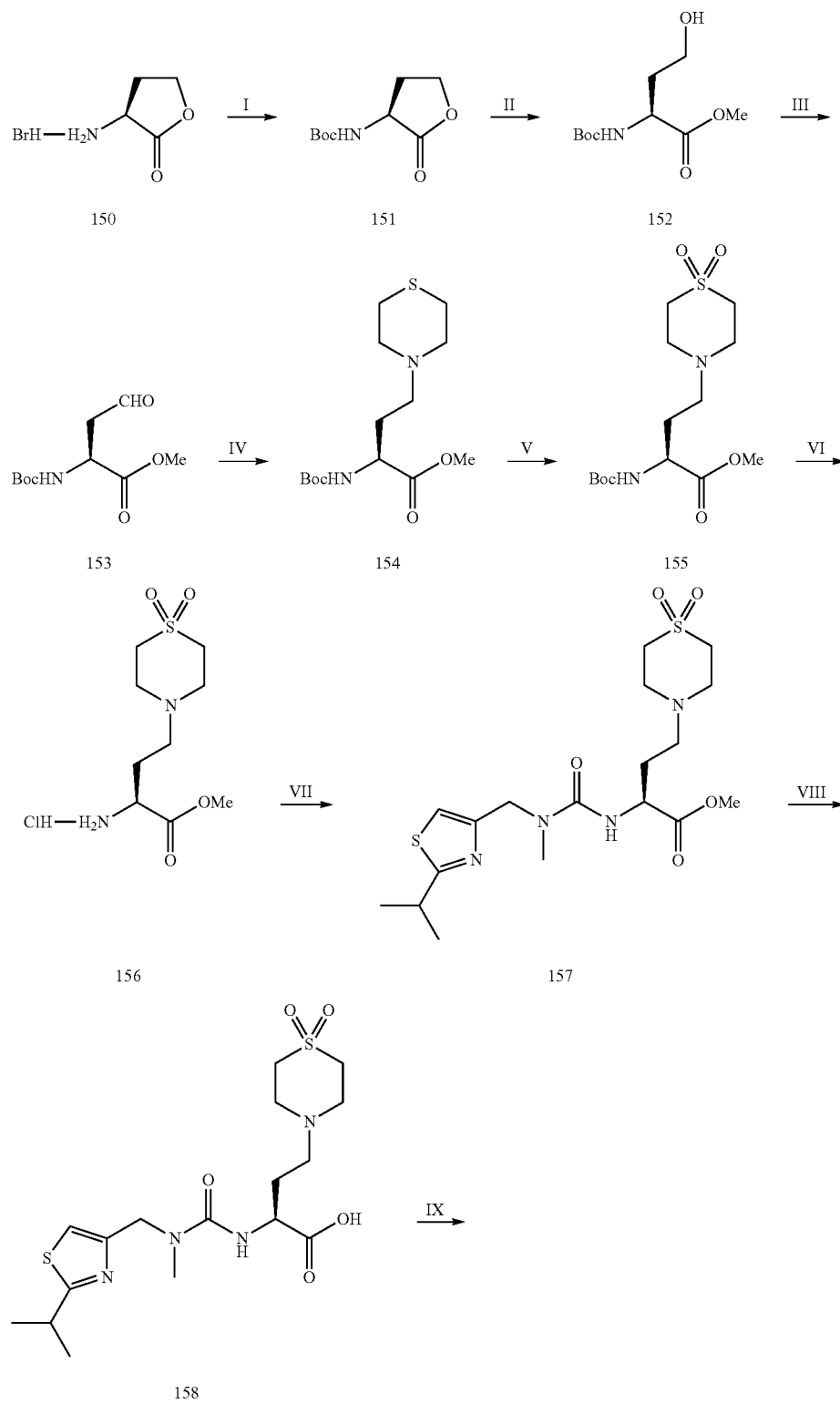
Scheme 100
