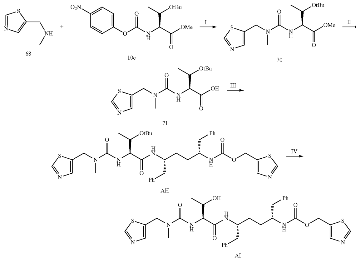
Scheme 29
