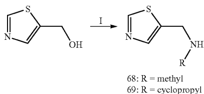
Scheme 28
