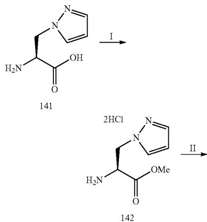
Scheme 93
