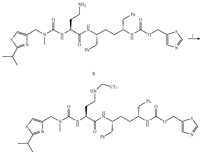
Scheme 85
