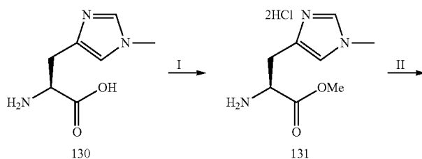
Scheme 75
