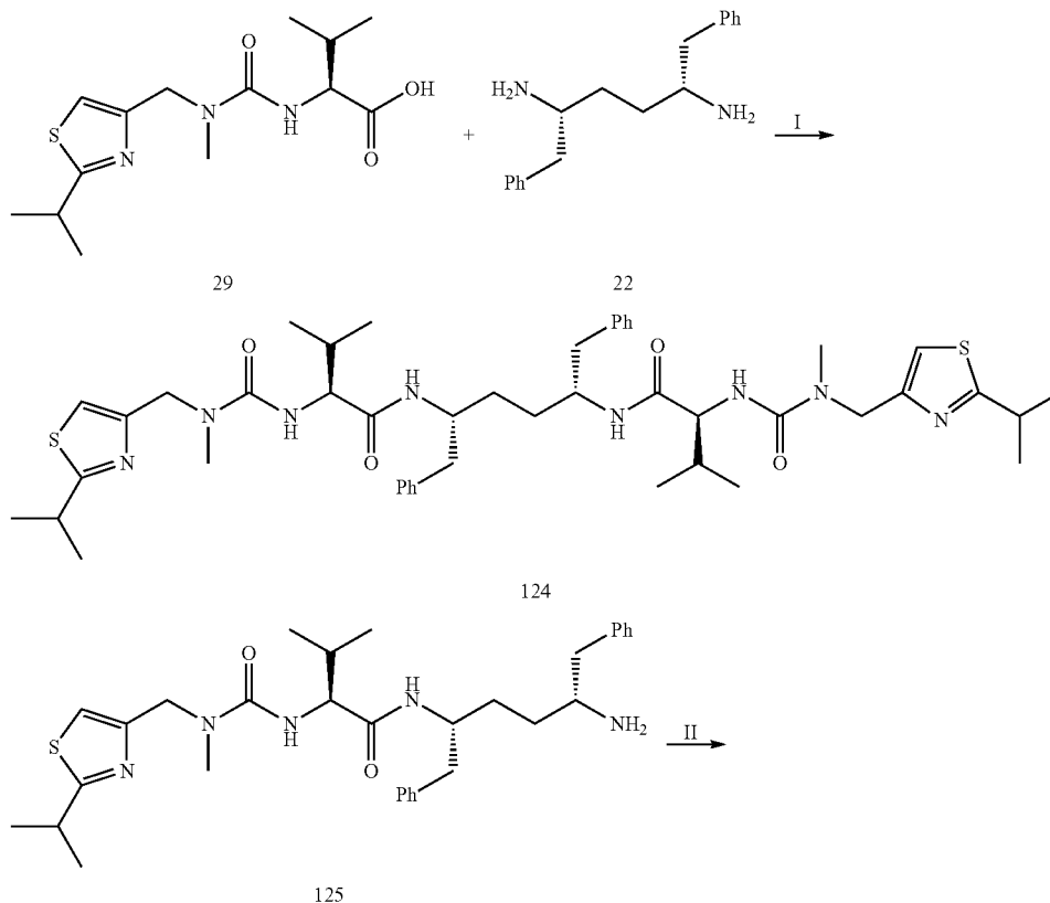
Scheme 71
