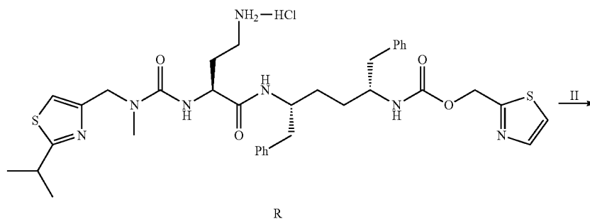
Scheme 82
