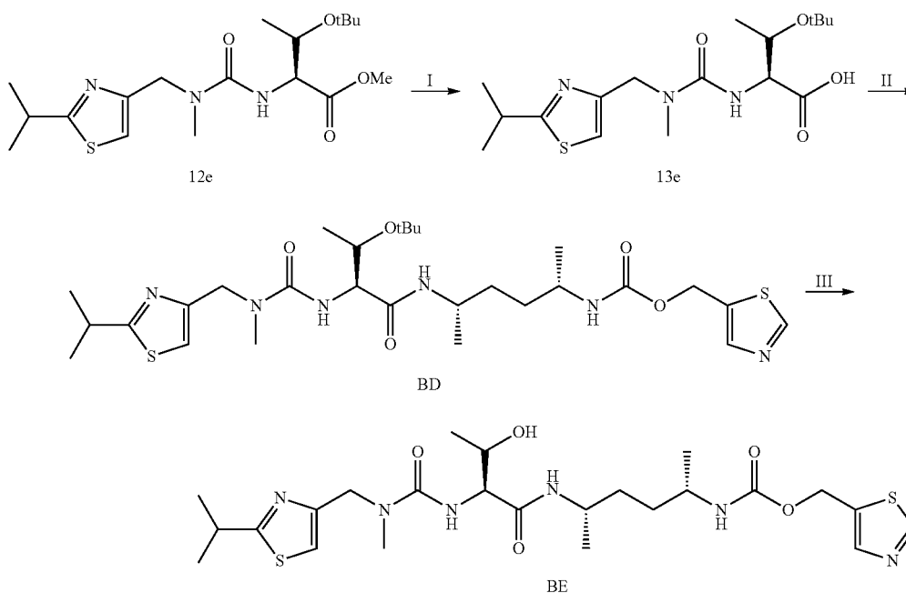
Scheme 45
