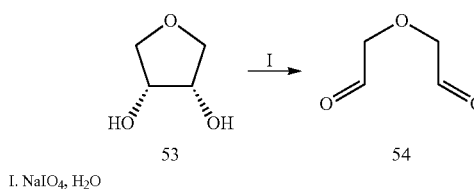
Scheme 20
