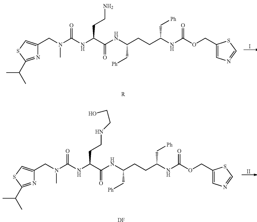
Scheme 87
