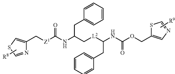
Formula IB
