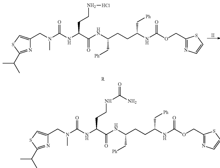
Scheme 79
