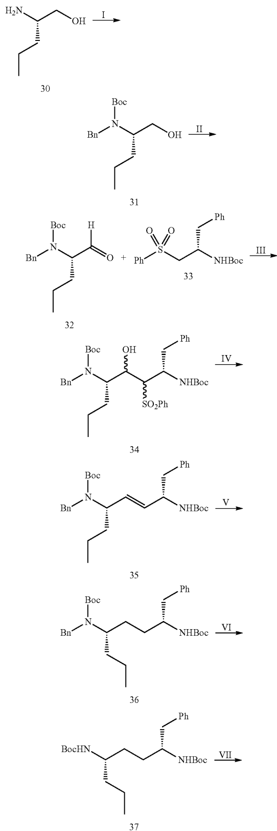
Scheme 14
