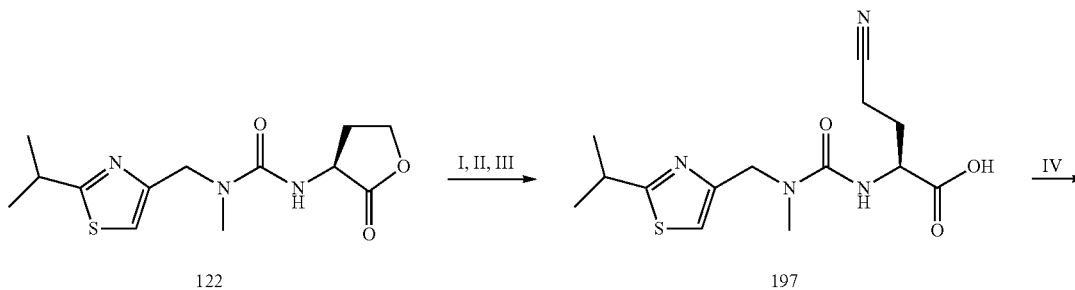
Scheme 113
