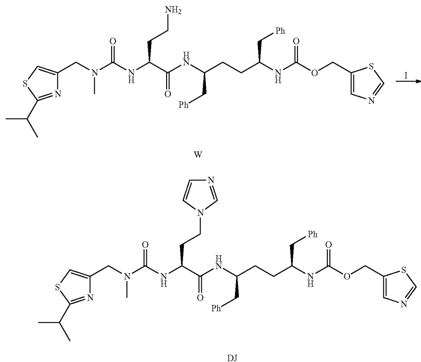
Scheme 90
