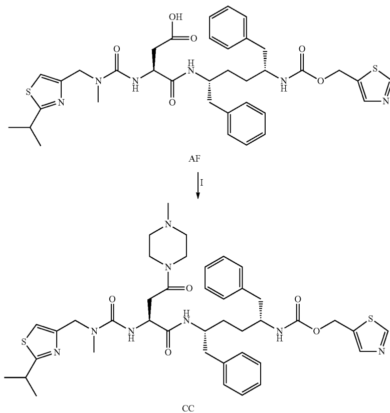
Scheme 65
