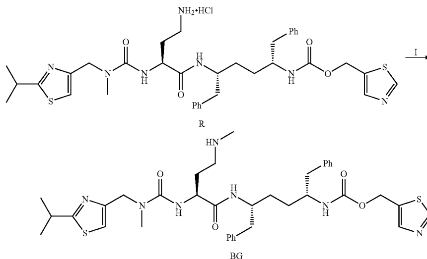
Scheme 47
