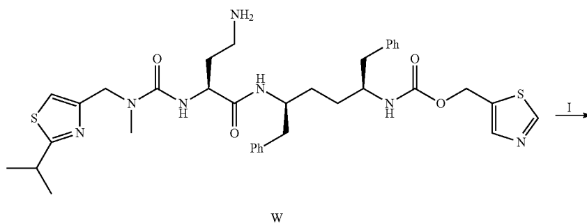
Scheme 91
