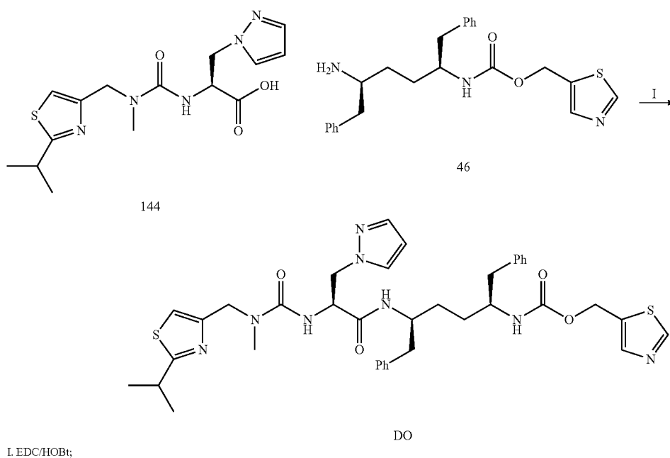
Scheme 94
