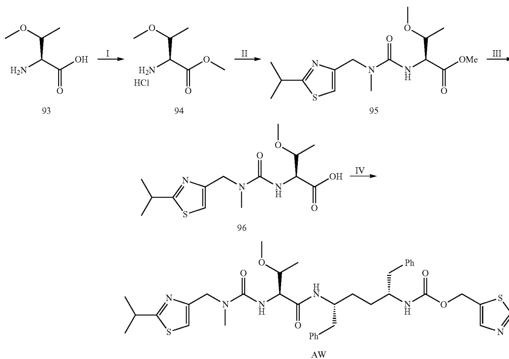
Scheme 40
