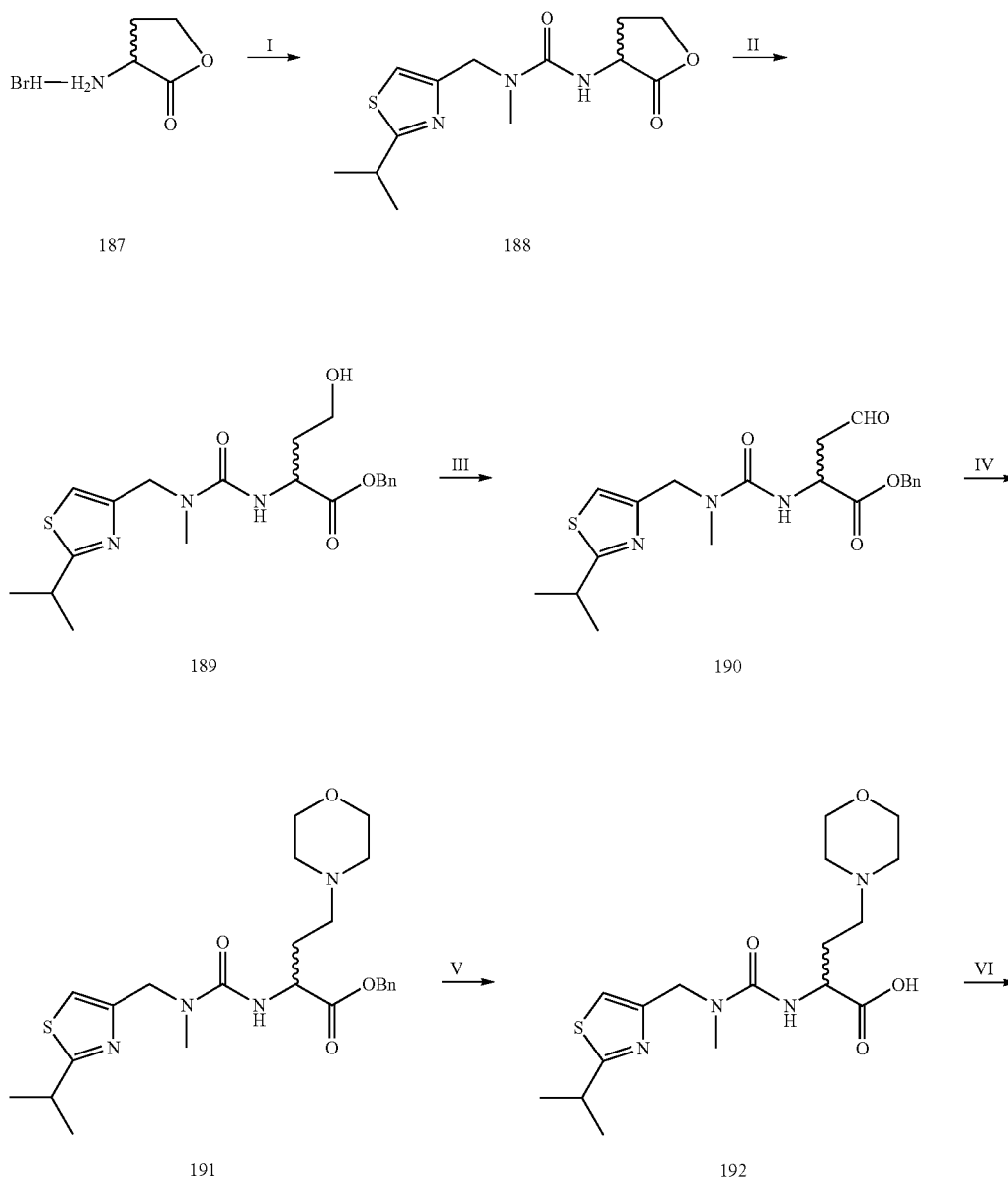
Scheme 110
