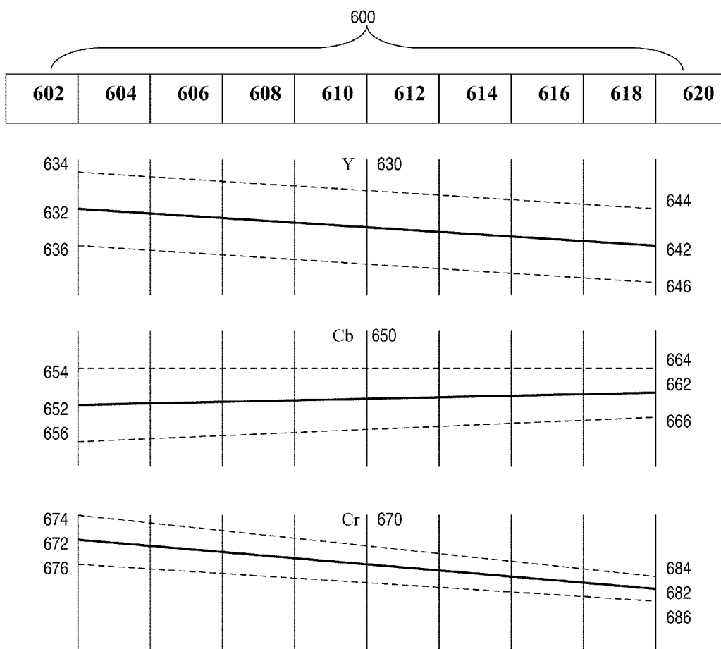
Example occlusion color processing over scene transition
