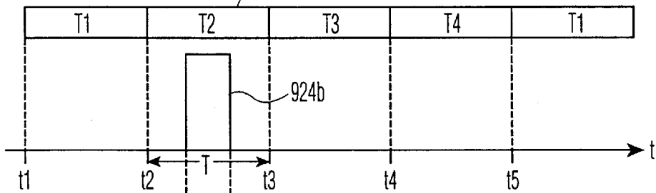
(3) RECORDED SIGNAL OF "01"
