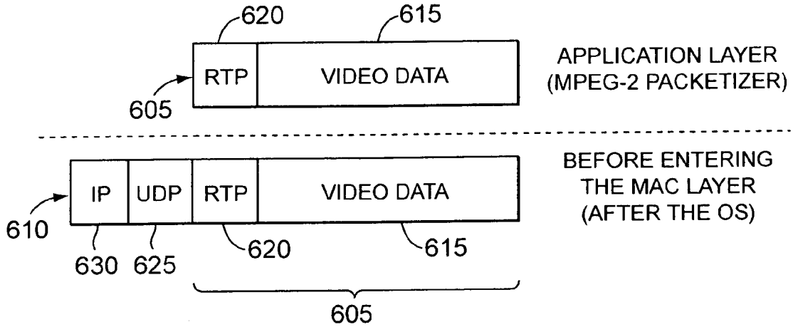
FIG. 6 (PRIOR ART)
