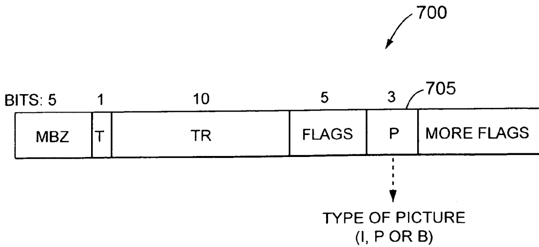
FIG. 7 (PRIOR ART)
