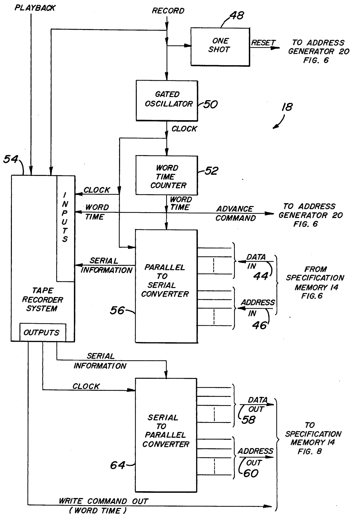
FIG. 7 EXTERNAL NON-VOLATILE READ-WRITE MEMORY SYSTEM
